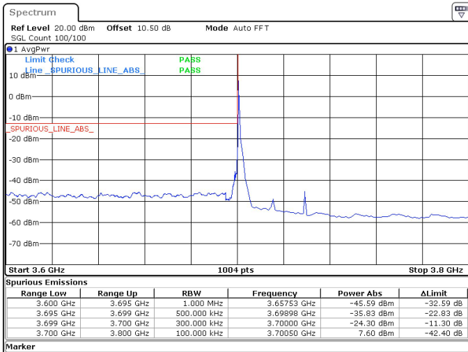
30MHz_15kHz_3715MHz_DFT-s-OFDM QPSK_RB1@0 -24.30 dBm
