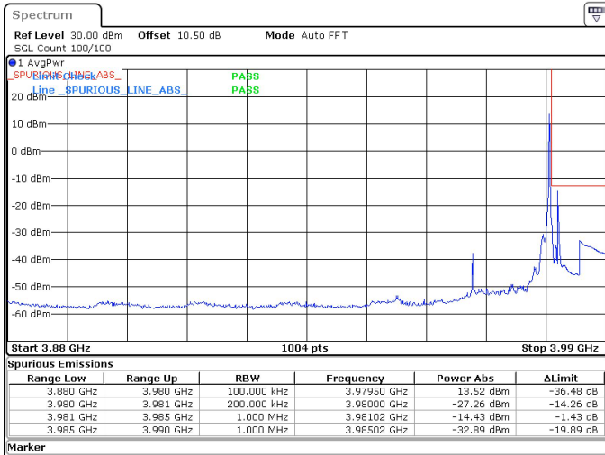
15MHz_15kHz_3972.5MHz_DFT-s-OFDM QPSK_RB1@78 -14.43 dBm
