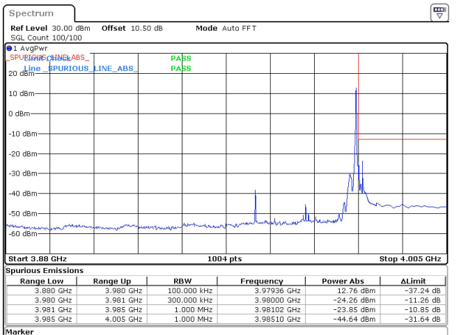
30MHz_15kHz_3965MHz_DFT-s-OFDM QPSK_RB1@159 -23.85 dBm
