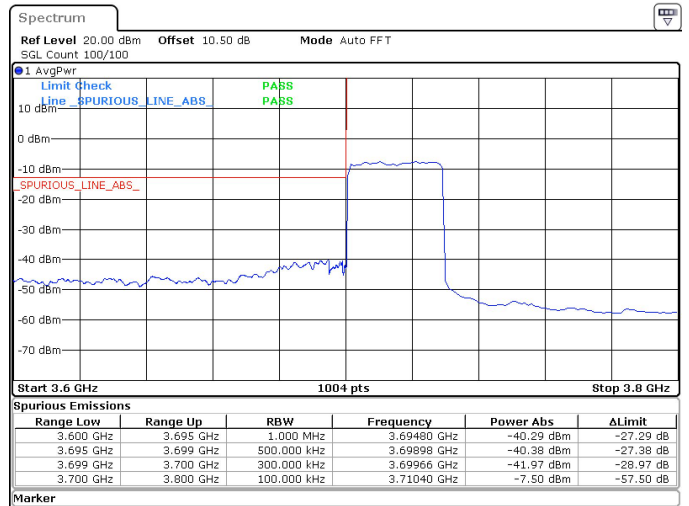
30MHz_15kHz_3715MHz_DFT-s-OFDM QPSK_RB160@0 -40.29 dBm
