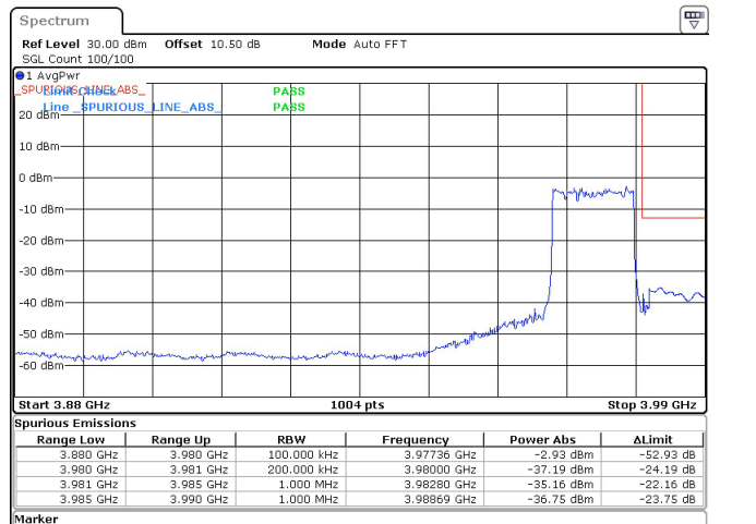
15MHz_30kHz_3972.5MHz_DFT-s-OFDM QPSK_RB36@0 -35.16 dBm
