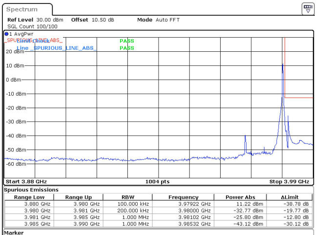
15MHz_30kHz_3972.5MHz_DFT-s-OFDM QPSK_RB1@37 -25.80 dBm
