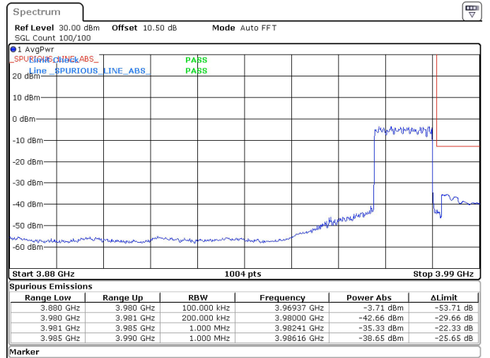
15MHz_15kHz_3972.5MHz_DFT-s-OFDM QPSK_RB75@0 -35.33 dBm
