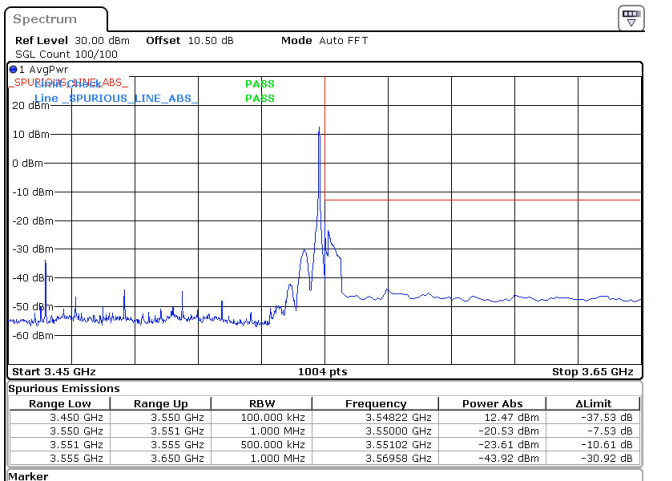
90MHz_30kHz_3505MHz_DFT-s-OFDM QPSK_RB1@244 -20.53 dBm
