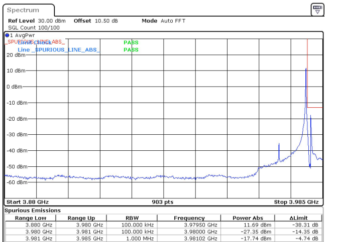
10MHz_15kHz_3975MHz_DFT-s-OFDM QPSK_RB1@51 -17.74 dBm
