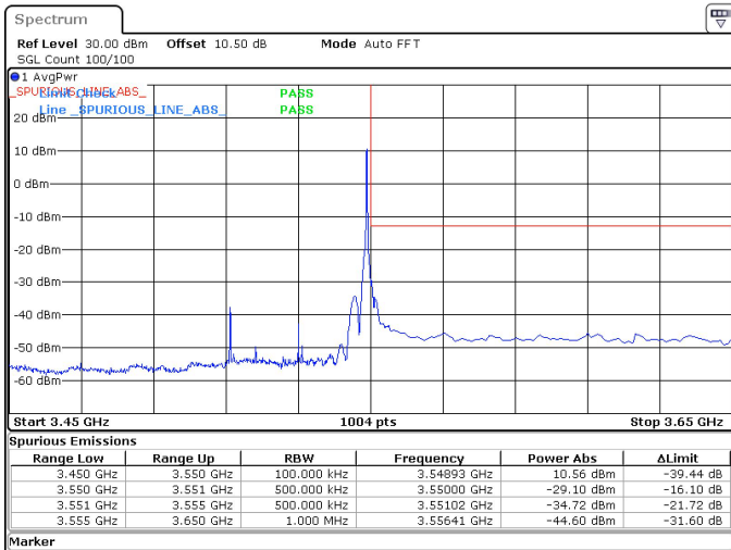
40MHz_30kHz_3530MHz_DFT-s-OFDM QPSK_RB1@105 -29.10 dBm
