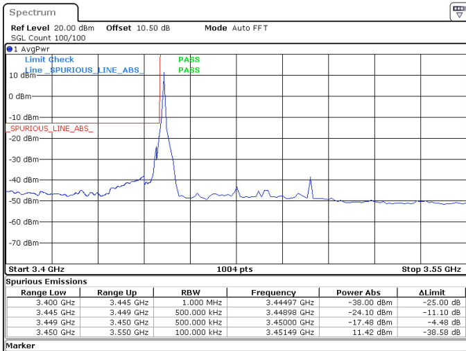
50MHz_30kHz_3475MHz_DFT-s-OFDM QPSK_RB1@0 -17.48 dBm
