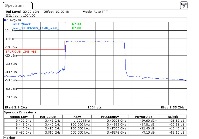
50MHz_15kHz_3475MHz_DFT-s-OFDM QPSK_RB270@0 -32.49 dBm
