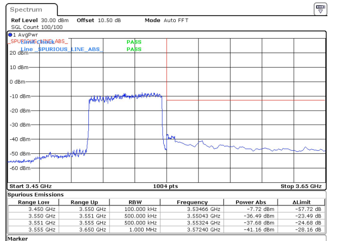
50MHz_30kHz_3525MHz_DFT-s-OFDM QPSK_RB128@0 -36.49 dBm
