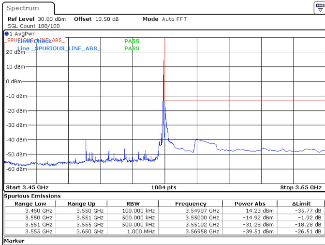
50MHz_15kHz_3525MHz_DFT-s-OFDM QPSK_RB1@269 -14.92 dBm
