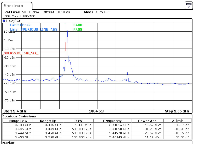
50MHz_15kHz_3475MHz_DFT-s-OFDM QPSK_RB1@0 -23.62 dBm
