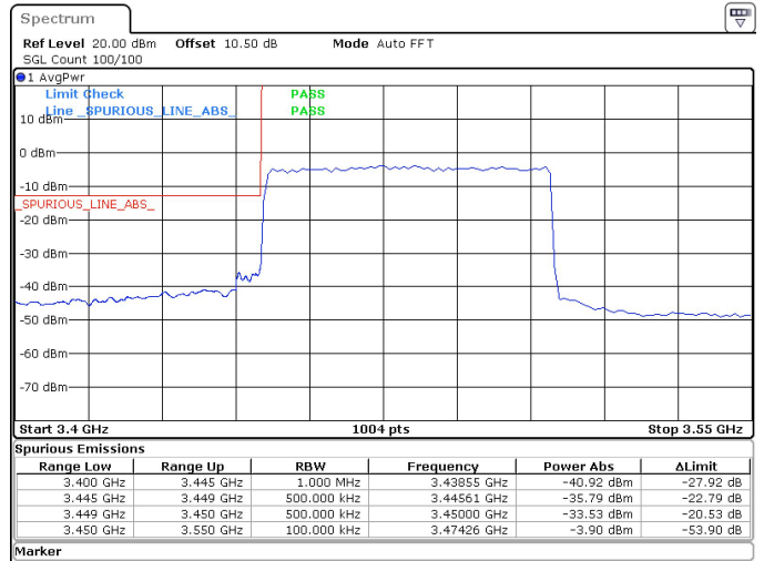
60MHz_30kHz_3480MHz_DFT-s-OFDM QPSK_RB162@0 -33.53 dBm
