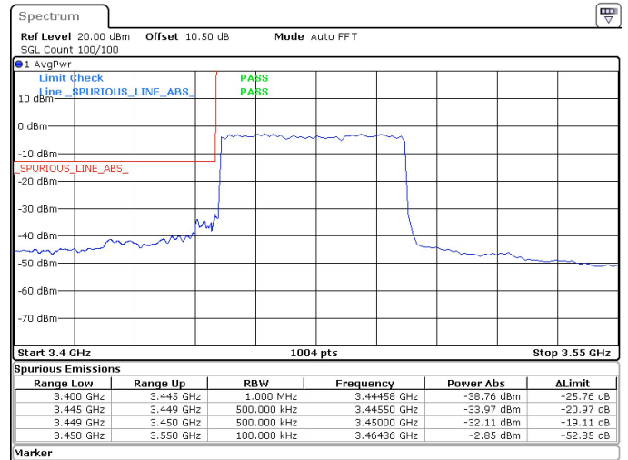
50MHz_30kHz_3475MHz_DFT-s-OFDM QPSK_RB128@0 -32.11 dBm
