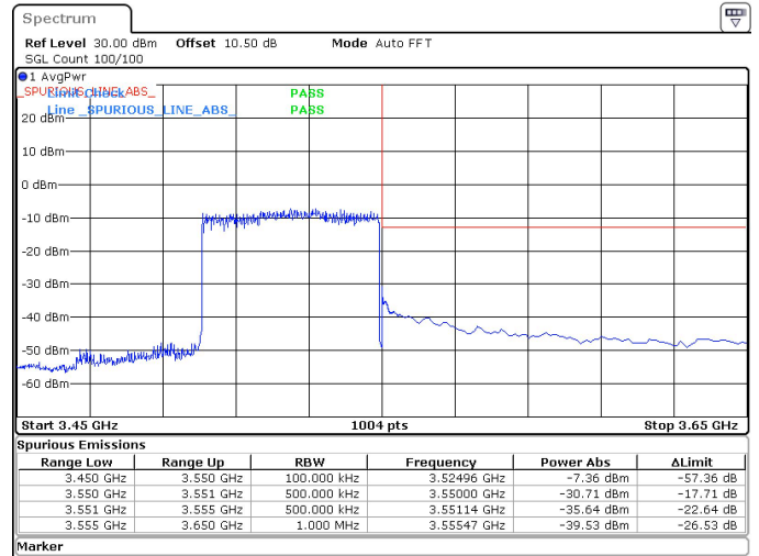
50MHz_15kHz_3525MHz_DFT-s-OFDM QPSK_RB270@0 -30.71 dBm
