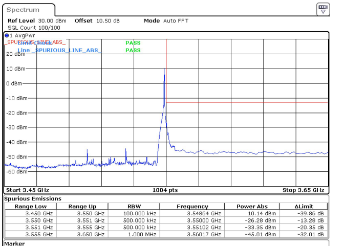
50MHz_30kHz_3525MHz_DFT-s-OFDM QPSK_RB1@132 -26.28 dBm
