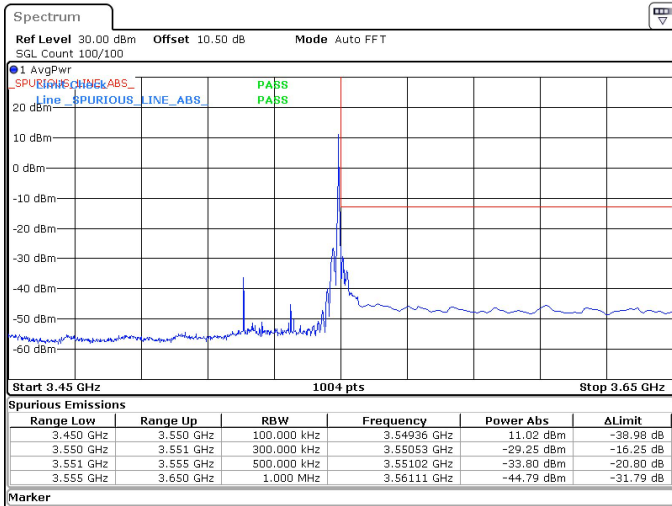
30MHz_15kHz_3535MHz_DFT-s-OFDM QPSK_RB1@159 -29.25 dBm
