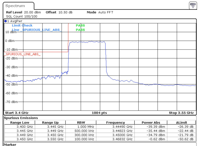
30MHz_15kHz_3465MHz_DFT-s-OFDM QPSK_RB160@0 -34.79 dBm
