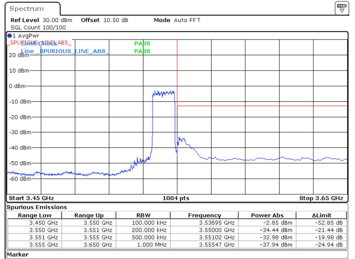
15MHz_30kHz_3542.5MHz_DFT-s-OFDM QPSK_RB36@0 -32.98 dBm
