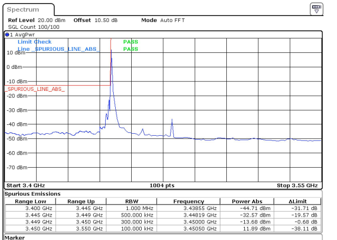
30MHz_15kHz_3465MHz_DFT-s-OFDM QPSK_RB1@0 -13.68 dBm
