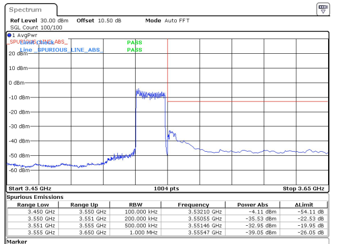
20MHz_15kHz_3540MHz_DFT-s-OFDM QPSK_RB100@0 -32.95 dBm
