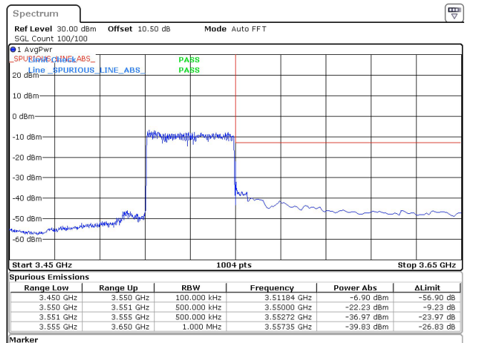
40MHz_15kHz_3530MHz_DFT-s-OFDM QPSK_RB216@0 -22.23 dBm
