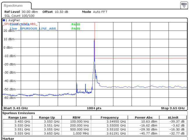
20MHz_15kHz_3540MHz_DFT-s-OFDM QPSK_RB1@105 -16.62 dBm
