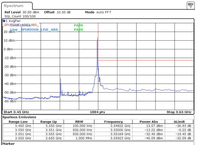
40MHz_15kHz_3530MHz_DFT-s-OFDM QPSK_RB1@215 -13.22 dBm
