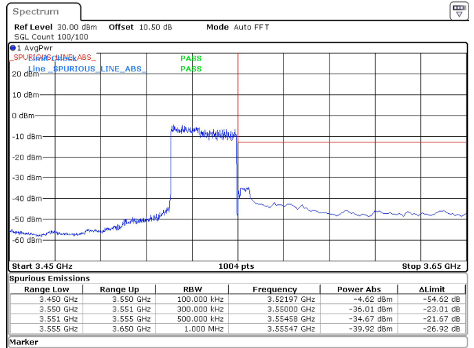
30MHz_15kHz_3535MHz_DFT-s-OFDM QPSK_RB160@0 -34.67 dBm
