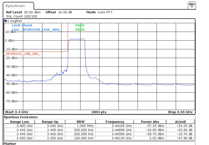
15MHz_30kHz_3457.5MHz_DFT-s-OFDM QPSK_RB36@0 -28.70 dBm
