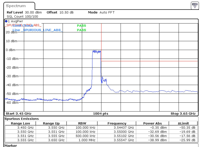
10MHz_30kHz_3545MHz_DFT-s-OFDM QPSK_RB24@0 -30.56 dBm
