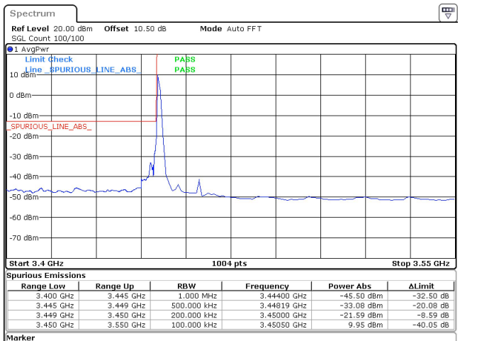
15MHz_30kHz_3457.5MHz_DFT-s-OFDM QPSK_RB1@0 -21.59 dBm
