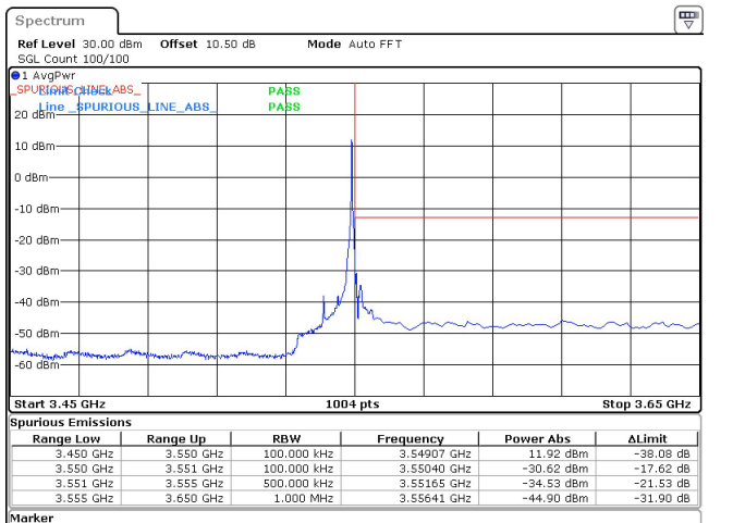
10MHz_30kHz_3545MHz_DFT-s-OFDM QPSK_RB1@23 -30.62 dBm
