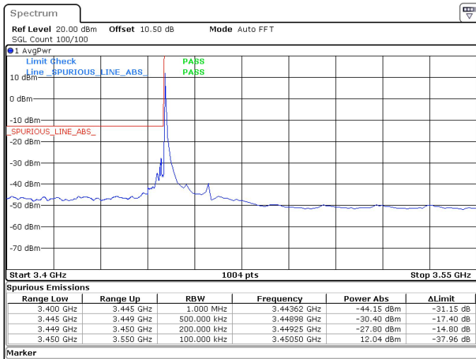
15MHz_15kHz_3457.5MHz_DFT-s-OFDM QPSK_RB1@0 -27.80 dBm
