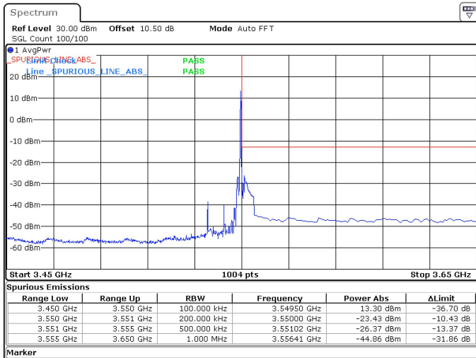
15MHz_15kHz_3542.5MHz_DFT-s-OFDM QPSK_RB1@78 -23.43 dBm
