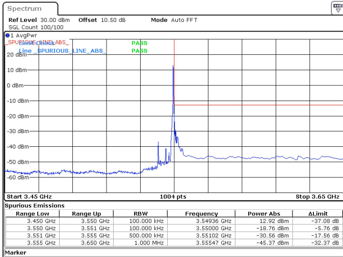
10MHz_15kHz_3545MHz_DFT-s-OFDM QPSK_RB1@51 -18.76 dBm
