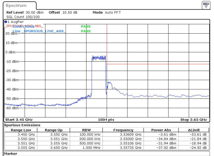
15MHz_15kHz_3542.5MHz_DFT-s-OFDM QPSK_RB75@0 -31.94 dBm
