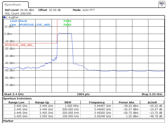
15MHz_15kHz_3457.5MHz_DFT-s-OFDM QPSK_RB75@0 -26.72 dBm
