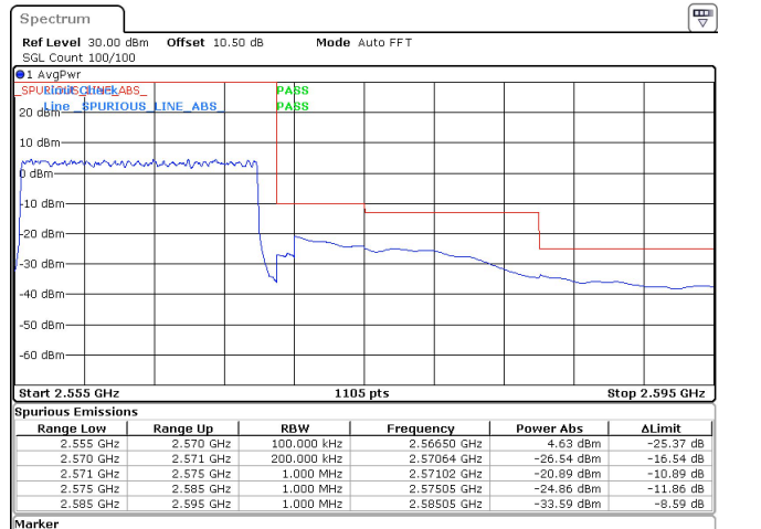
15MHz_15kHz_2562.5MHz_DFT-s-OFDM QPSK_RB75@0 -33.59 dBm
