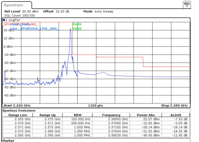
15MHz_15kHz_2562.5MHz_DFT-s-OFDM QPSK_RB1@78 -12.05 dBm
