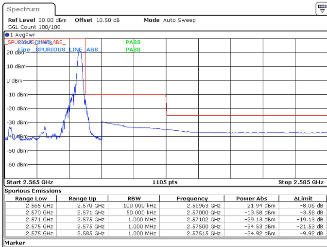
5MHz_15kHz_2567.5MHz_DFT-s-OFDM QPSK_RB1@24 -13.58 dBm
