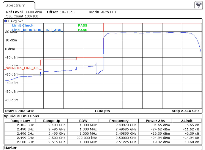
15MHz_15kHz_2507.5MHz_DFT-s-OFDM QPSK_RB75@0 -16.39 dBm
