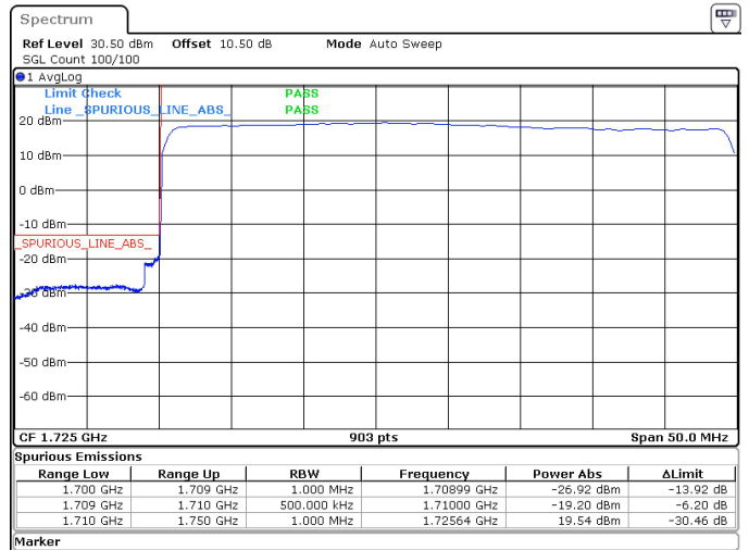
40MHz_15kHz_1730MHz_DFT-s-OFDM QPSK_RB216@0 -19.20 dBm
