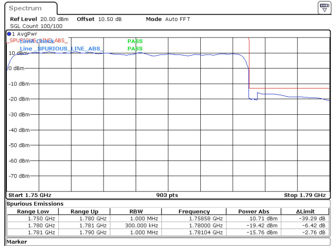
30MHz_15kHz_1765MHz_DFT-s-OFDM QPSK_RB160@0 -15.76 dBm
