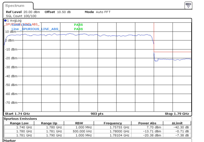
40MHz_15kHz_1760MHz_DFT-s-OFDM QPSK_RB216@0 -13.71 dBm
