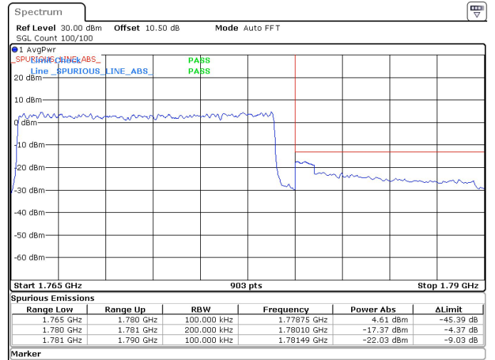
15MHz_15kHz_1772.5MHz_DFT-s-OFDM QPSK_RB75@0 -17.37 dBm
