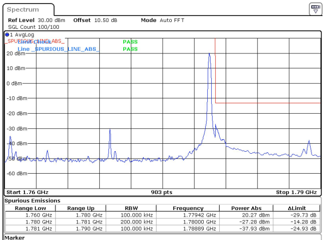
20MHz_15kHz_1770MHz_DFT-s-OFDM QPSK_RB1@105 -27.28 dBm
