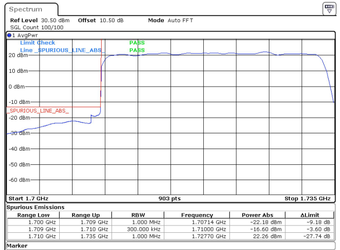
25MHz_15kHz_1722.5MHz_DFT-s-OFDM QPSK_RB128@0 -16.60 dBm
