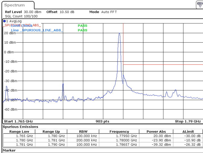
15MHz_15kHz_1772.5MHz_DFT-s-OFDM QPSK_RB1@78 -23.90 dBm
