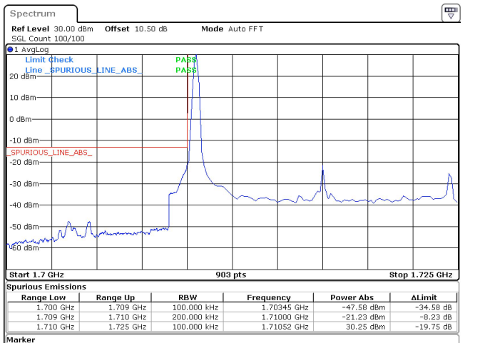
15MHz_15kHz_1717.5MHz_DFT-s-OFDM QPSK_RB1@0 -21.23 dBm
