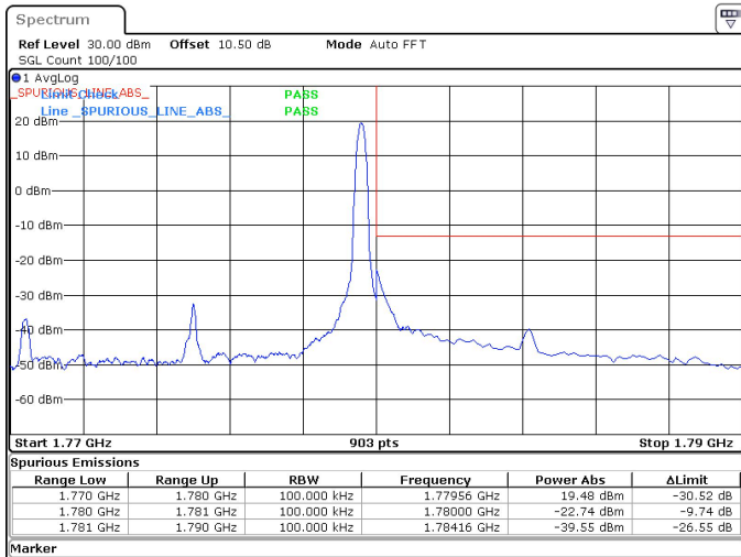
10MHz_15kHz_1775MHz_DFT-s-OFDM QPSK_RB1@51 -22.74 dBm
