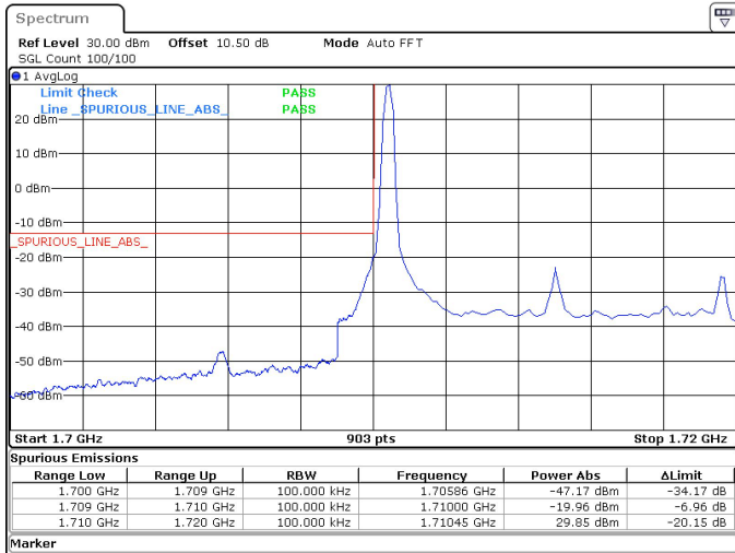
10MHz_15kHz_1715MHz_DFT-s-OFDM QPSK_RB1@0 -19.96 dBm
