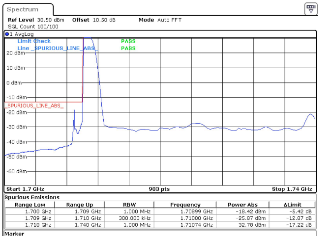
30MHz_15kHz_1725MHz_DFT-s-OFDM QPSK_RB1@0 -18.42 dBm
