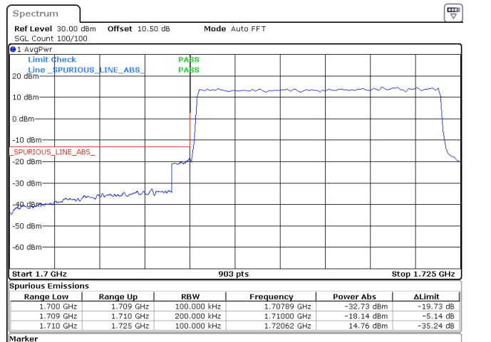
15MHz_15kHz_1717.5MHz_DFT-s-OFDM QPSK_RB75@0 -18.14 dBm
