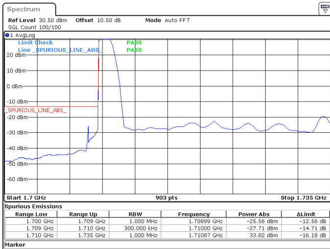
25MHz_15kHz_1722.5MHz_DFT-s-OFDM QPSK_RB1@0 -25.56 dBm
