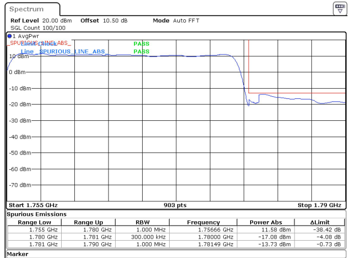
25MHz_15kHz_1767.5MHz_DFT-s-OFDM QPSK_RB128@0 -13.73 dBm
