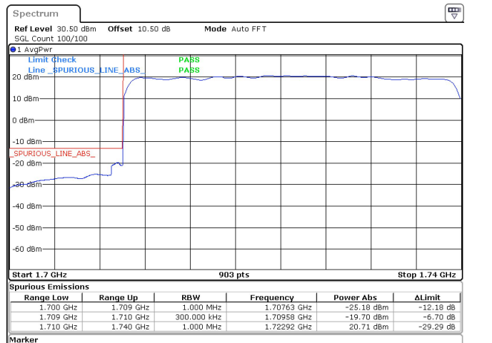
30MHz_15kHz_1725MHz_DFT-s-OFDM QPSK_RB160@0 -19.70 dBm
