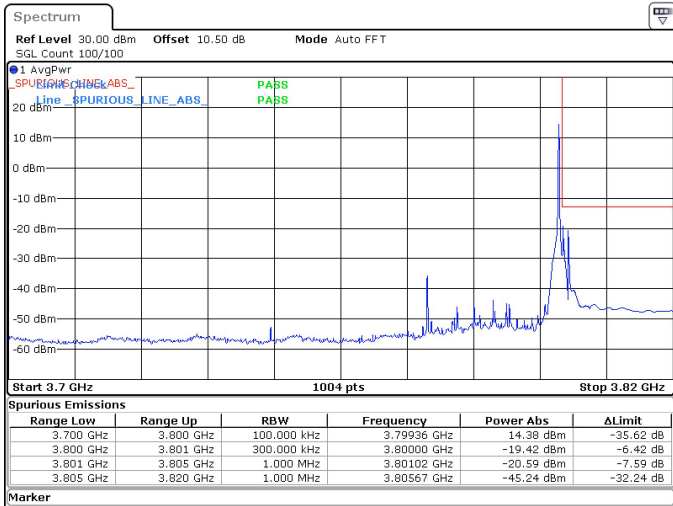
25MHz_15kHz_3787.5MHz_DFT-s-OFDM QPSK_RB1@132 -19.42 dBm
