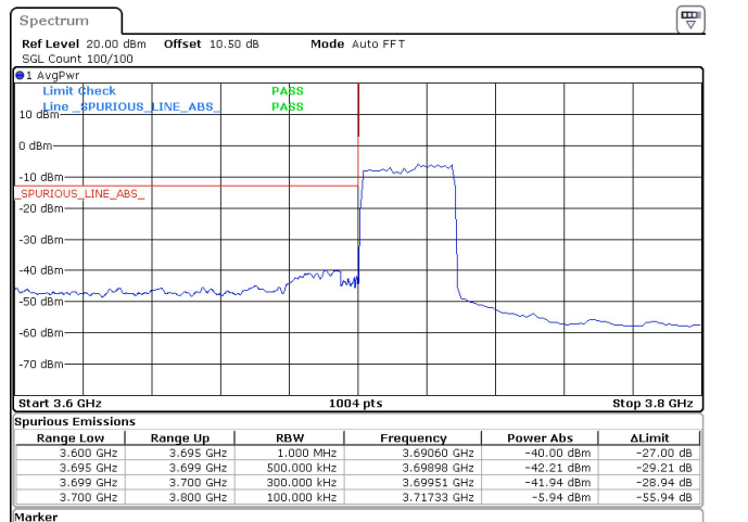
30MHz_30kHz_3715MHz_DFT-s-OFDM QPSK_RB75@0 -40.00 dBm
