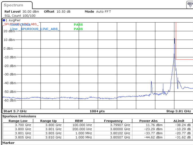
15MHz_30kHz_3792.5MHz_DFT-s-OFDM QPSK_RB1@37 -23.29 dBm
