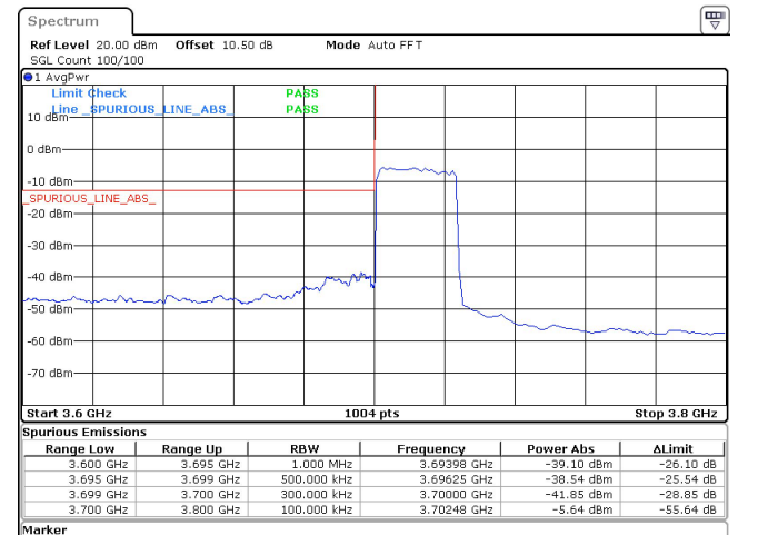
25MHz_15kHz_3712.5MHz_DFT-s-OFDM QPSK_RB128@0 -38.54 dBm
