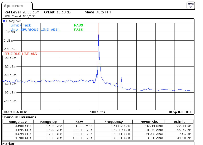
25MHz_15kHz_3712.5MHz_DFT-s-OFDM QPSK_RB1@0 -20.25 dBm
