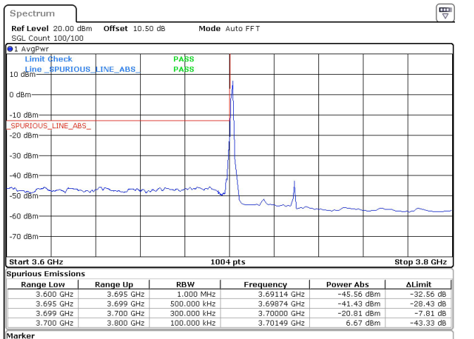
30MHz_30kHz_3715MHz_DFT-s-OFDM QPSK_RB1@0 -20.81 dBm
