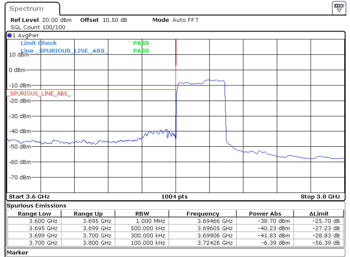
30MHz_15kHz_3715MHz_DFT-s-OFDM QPSK_RB160@0 -38.70 dBm
