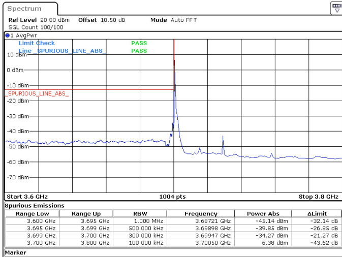
30MHz_15kHz_3715MHz_DFT-s-OFDM QPSK_RB1@0 -34.27 dBm
