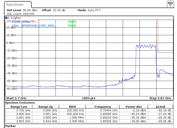
15MHz_30kHz_3792.5MHz_DFT-s-OFDM QPSK_RB36@0 -35.32 dBm
