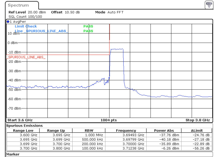
15MHz_30kHz_3707.5MHz_DFT-s-OFDM QPSK_RB36@0 -35.89 dBm
