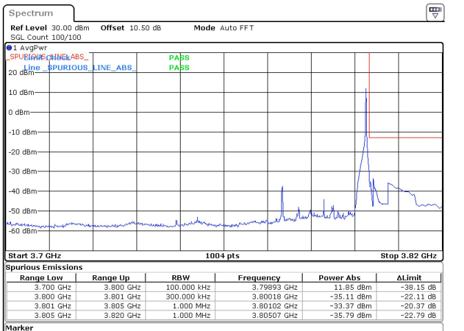
25MHz_30kHz_3787.5MHz_DFT-s-OFDM QPSK_RB1@64 -33.37 dBm
