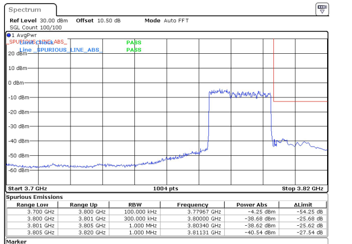
25MHz_30kHz_3787.5MHz_DFT-s-OFDM QPSK_RB64@0 -38.62 dBm
