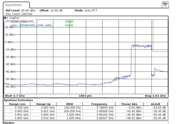
15MHz_15kHz_3792.5MHz_DFT-s-OFDM QPSK_RB75@0 -35.42 dBm
