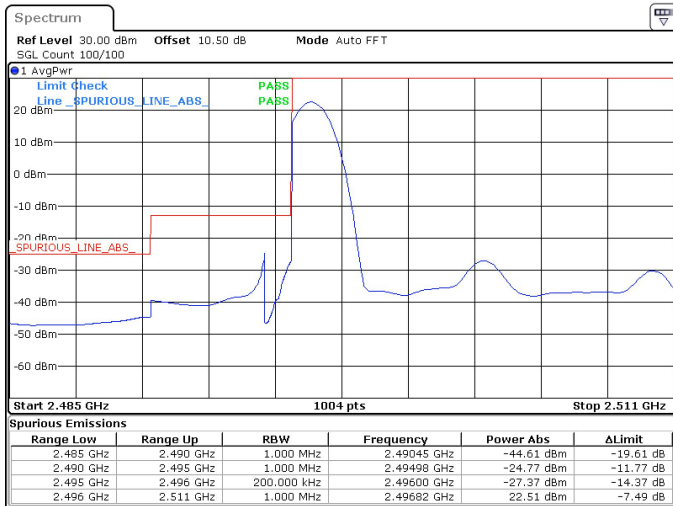
15MHz_30kHz_2503.5MHz_DFT-s-OFDM QPSK_RB1@0 22.51 dBm
