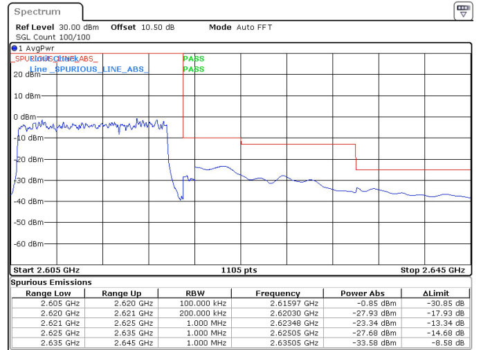
15MHz_30kHz_2612.5MHz_DFT-s-OFDM QPSK_RB36@0 -33.58 dBm
