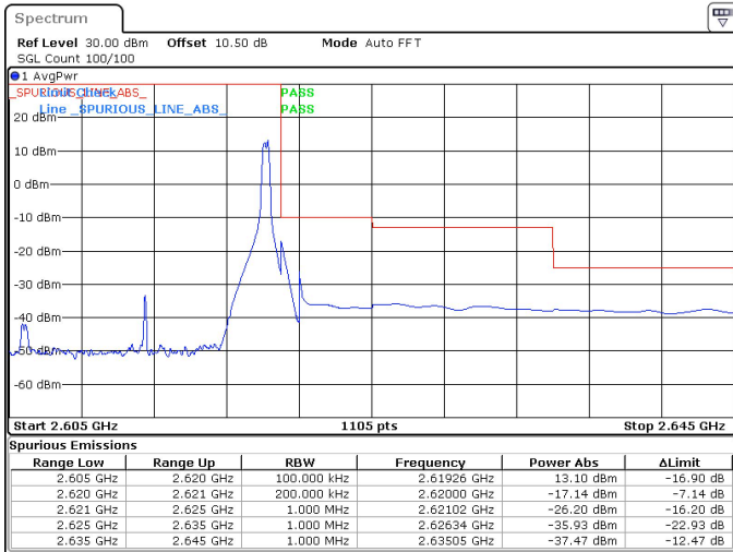
15MHz_30kHz_2612.5MHz_DFT-s-OFDM QPSK_RB1@37 -17.14 dBm
