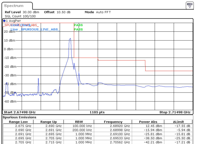
15MHz_30kHz_2682.48MHz_DFT-s-OFDM QPSK_RB1@37 -15.94 dBm
