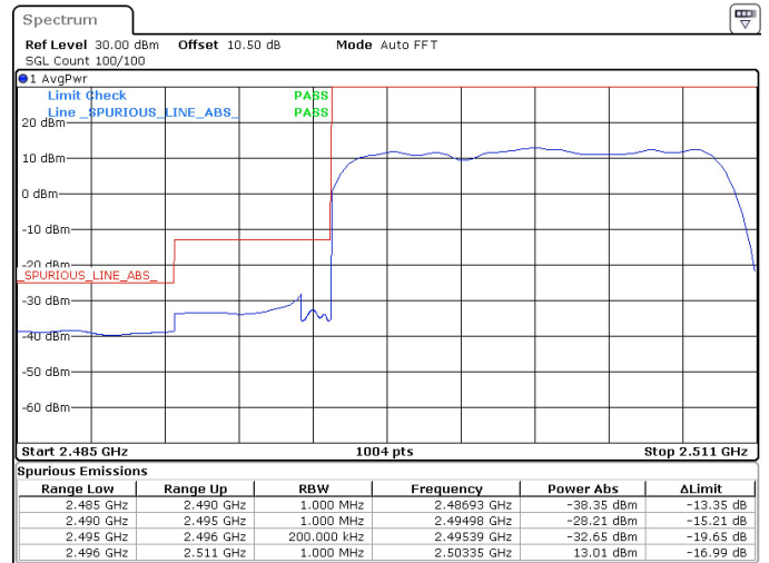
15MHz_30kHz_2503.5MHz_DFT-s-OFDM QPSK_RB36@0 -38.35 dBm
