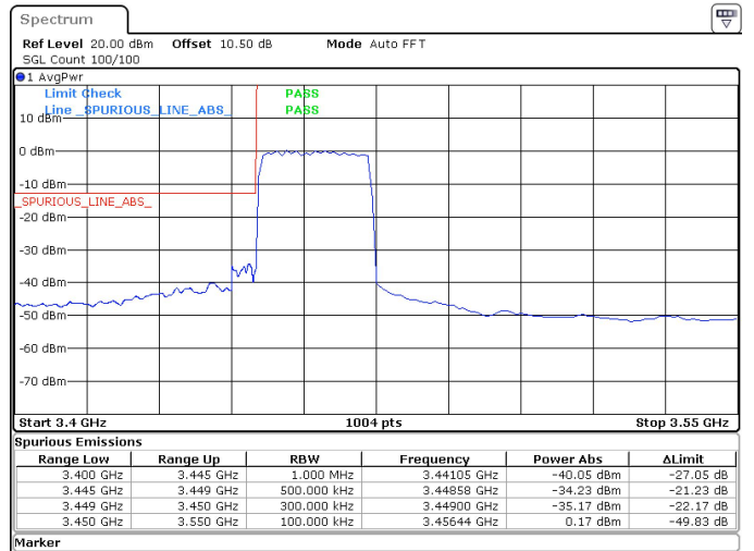
25MHz_30kHz_3462.5MHz_DFT-s-OFDM QPSK_RB64@0 -34.23 dBm
