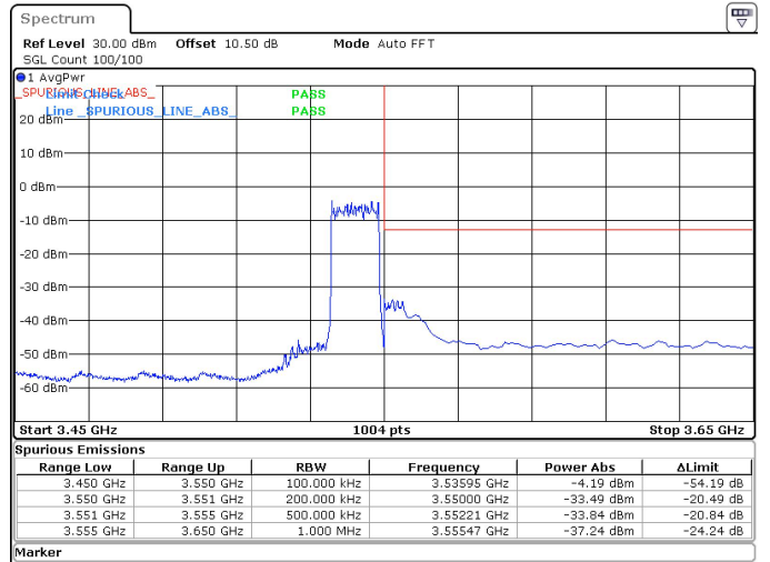
15MHz_30kHz_3542.5MHz_DFT-s-OFDM QPSK_RB36@0 -33.49 dBm
