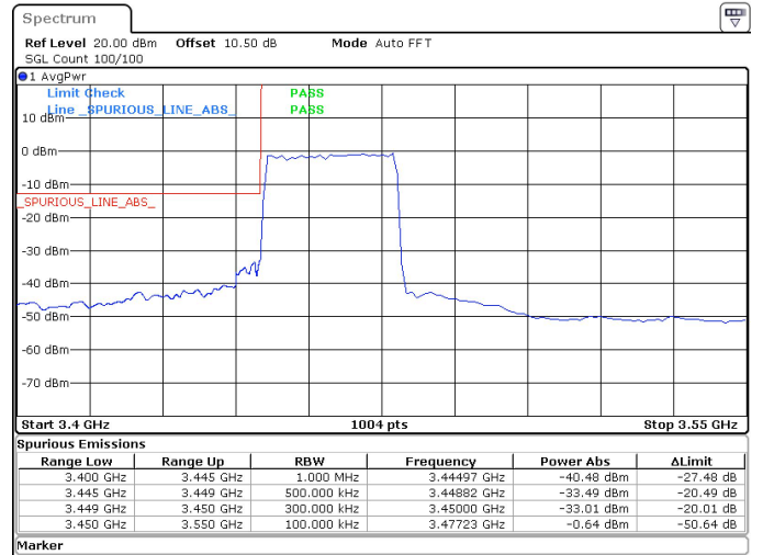
30MHz_30kHz_3465MHz_DFT-s-OFDM QPSK_RB75@0 -33.01 dBm
