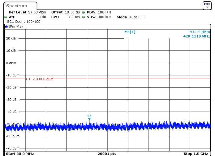
15MHz_15kHz_3750MHz_DFT-s-OFDM QPSK_RB75@0 -47.12 dBm
