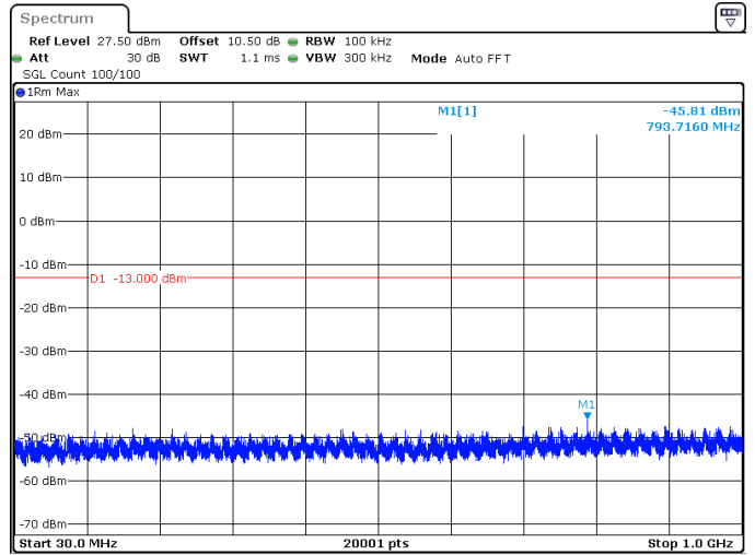
50MHz_15kHz_3775MHz_DFT-s-OFDM QPSK_RB1@0 -45.81 dBm
