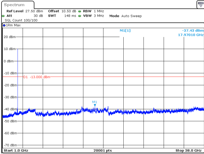
50MHz_15kHz_3725MHz_DFT-s-OFDM QPSK_RB1@269 -37.43 dBm
