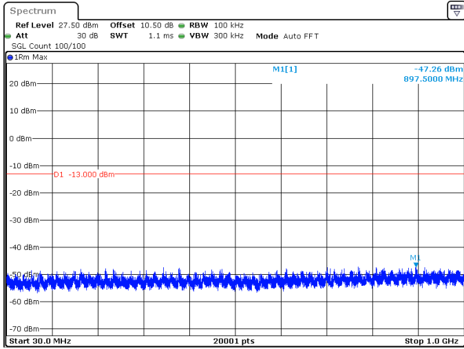
50MHz_15kHz_3775MHz_DFT-s-OFDM QPSK_RB1@269 -47.26 dBm
