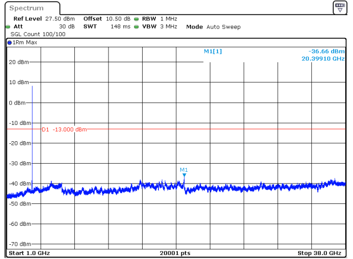
25MHz_15kHz_3750MHz_DFT-s-OFDM QPSK_RB1@132 -36.66 dBm
