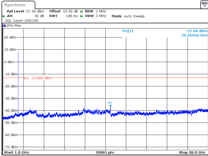
15MHz_30kHz_3750MHz_DFT-s-OFDM QPSK_RB1@37 -37.06 dBm
