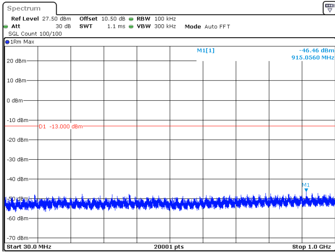
15MHz_30kHz_3707.5MHz_DFT-s-OFDM QPSK_RB1@0 -46.46 dBm
