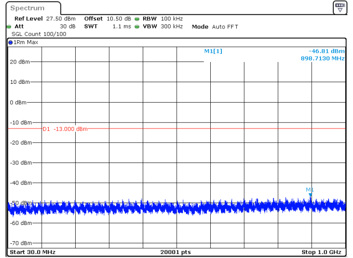
40MHz_30kHz_3780MHz_DFT-s-OFDM QPSK_RB1@105 -46.81 dBm
