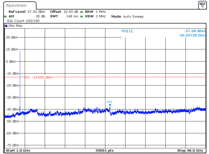
25MHz_15kHz_3787.5MHz_DFT-s-OFDM QPSK_RB1@132 -37.30 dBm
