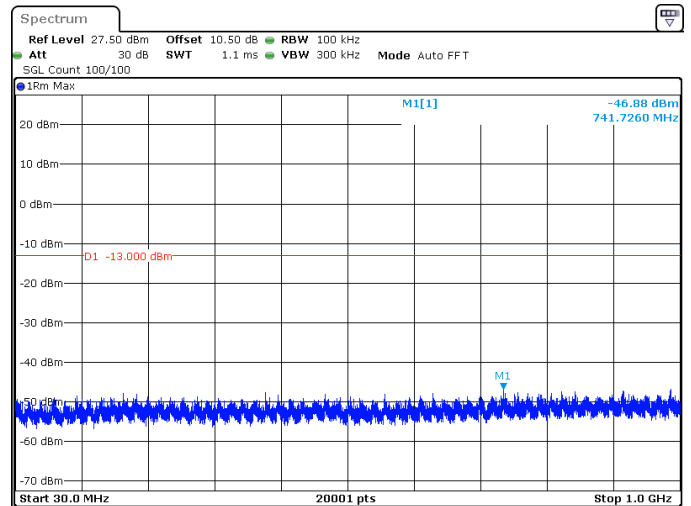
15MHz_30kHz_3707.5MHz_DFT-s-OFDM QPSK_RB36@0 -46.88 dBm
