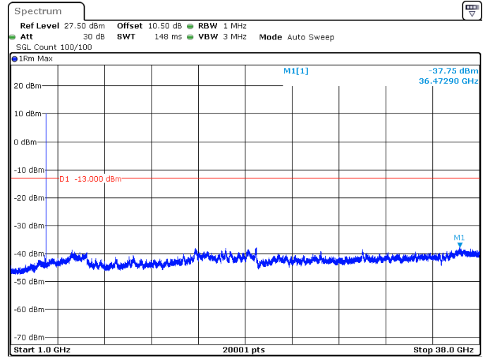
50MHz_15kHz_3750MHz_DFT-s-OFDM QPSK_RB1@269 -37.75 dBm
