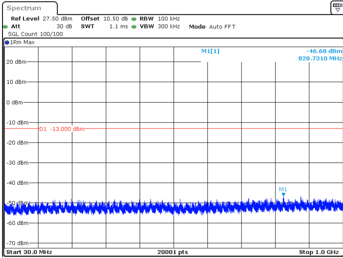
25MHz_15kHz_3750MHz_DFT-s-OFDM QPSK_RB1@132 -46.68 dBm
