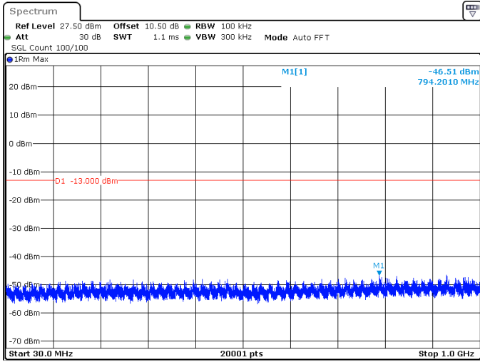
40MHz_30kHz_3750MHz_DFT-s-OFDM QPSK_RB1@105 -46.51 dBm
