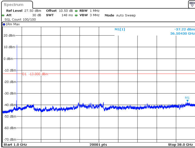
50MHz_30kHz_3750MHz_DFT-s-OFDM QPSK_RB1@132 -37.22 dBm
