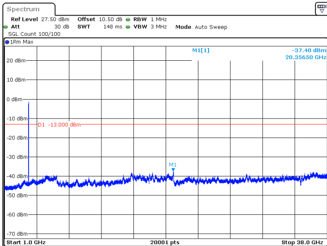
30MHz_15kHz_3750MHz_DFT-s-OFDM QPSK_RB160@0 -37.40 dBm
