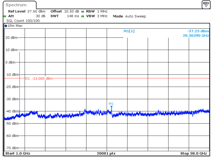
30MHz_15kHz_3750MHz_DFT-s-OFDM QPSK_RB1@159 -37.23 dBm
