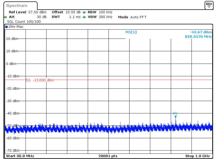
25MHz_30kHz_3787.5MHz_DFT-s-OFDM QPSK_RB1@64 -43.67 dBm
