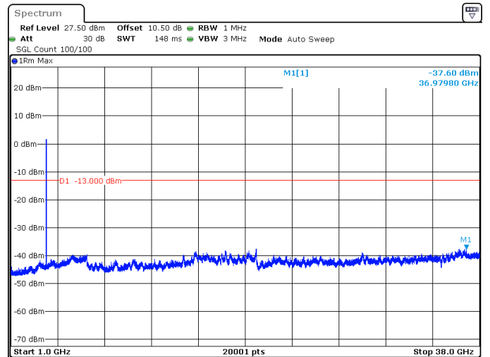
25MHz_30kHz_3787.5MHz_DFT-s-OFDM QPSK_RB64@0 -37.60 dBm
