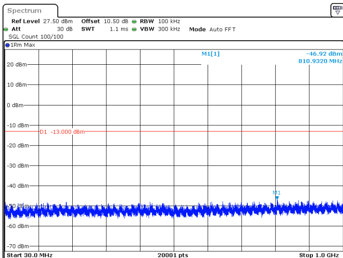
25MHz_30kHz_3712.5MHz_DFT-s-OFDM QPSK_RB64@0 -46.92 dBm
