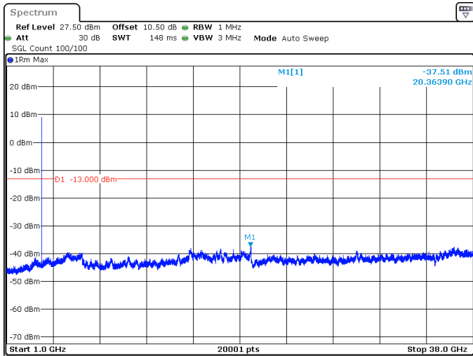
15MHz_15kHz_3750MHz_DFT-s-OFDM QPSK_RB1@78 -37.51 dBm
