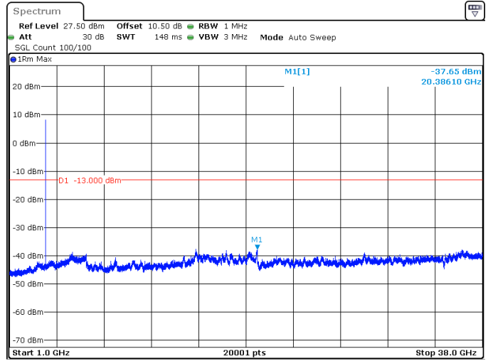
30MHz_15kHz_3785MHz_DFT-s-OFDM QPSK_RB1@159 -37.65 dBm
