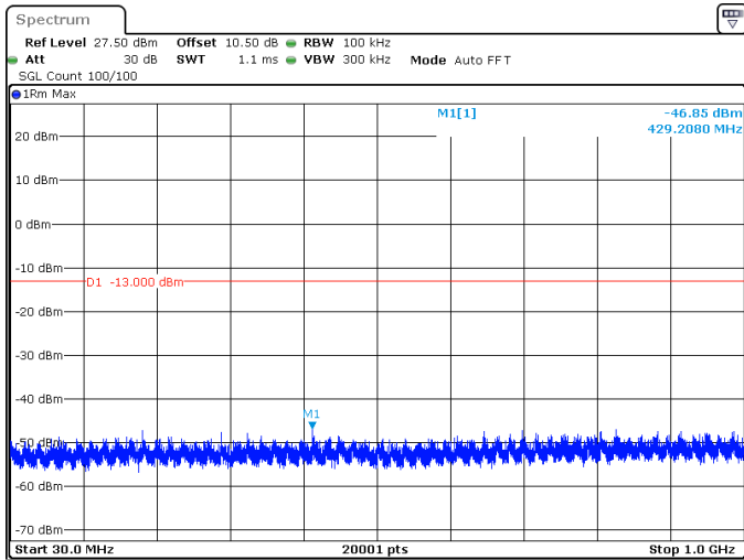
15MHz_30kHz_3707.5MHz_DFT-s-OFDM QPSK_RB1@37 -46.85 dBm
