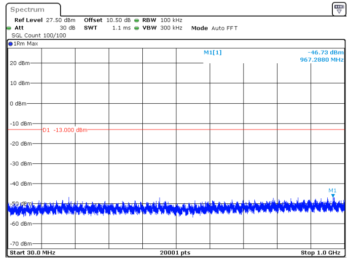
15MHz_15kHz_3792.5MHz_DFT-s-OFDM QPSK_RB1@0 -46.73 dBm
