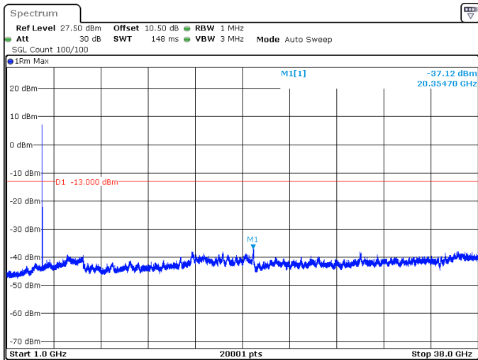
15MHz_30kHz_3792.5MHz_DFT-s-OFDM QPSK_RB1@0 -37.12 dBm
