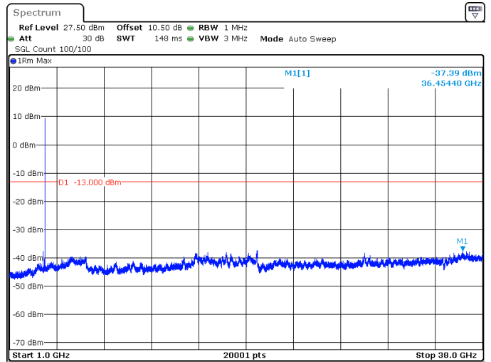
80MHz_30kHz_3740MHz_DFT-s-OFDM QPSK_RB1@216 -37.39 dBm
