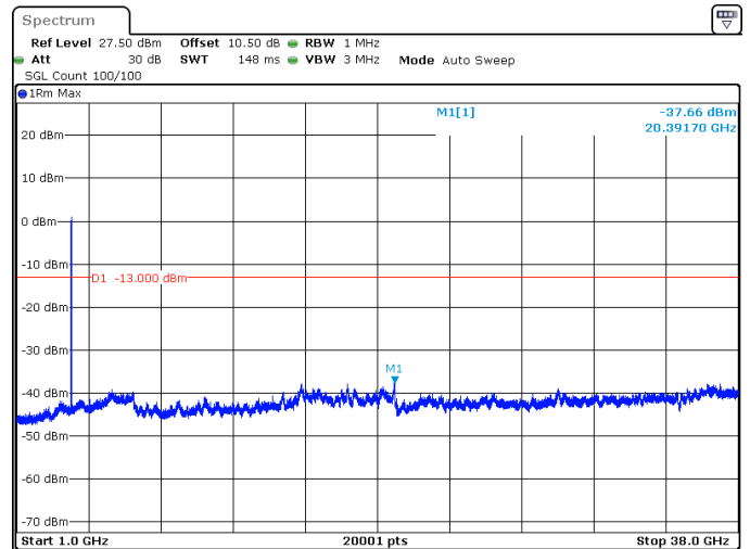
15MHz_15kHz_3792.5MHz_DFT-s-OFDM QPSK_RB75@0 -37.66 dBm
