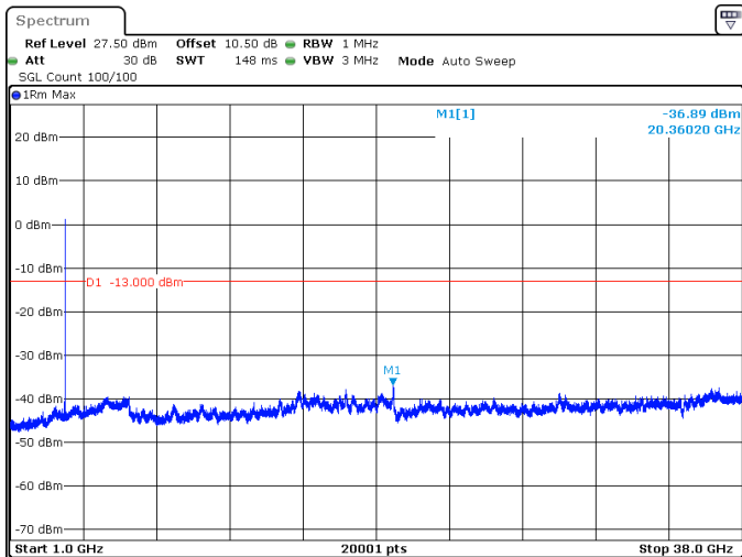
15MHz_15kHz_3750MHz_DFT-s-OFDM QPSK_RB75@0 -36.89 dBm
