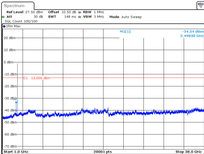
30MHz_15kHz_3715MHz_DFT-s-OFDM QPSK_RB160@0 -34.54 dBm
