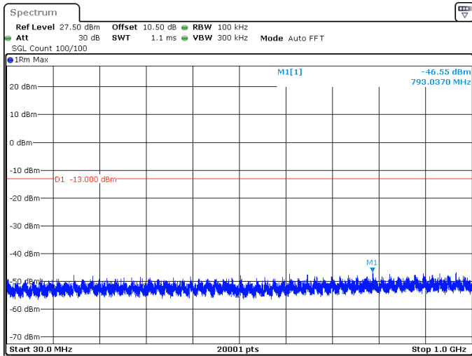
25MHz_15kHz_3712.5MHz_DFT-s-OFDM QPSK_RB1@132 -46.55 dBm
