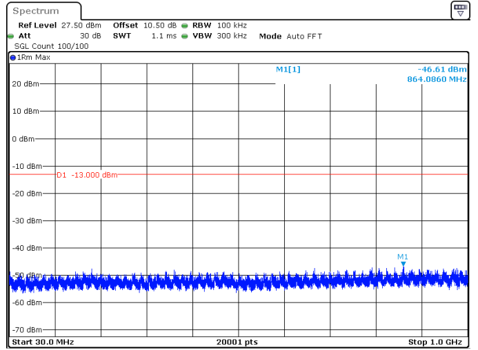
60MHz_30kHz_3730MHz_DFT-s-OFDM QPSK_RB1@161 -46.61 dBm
