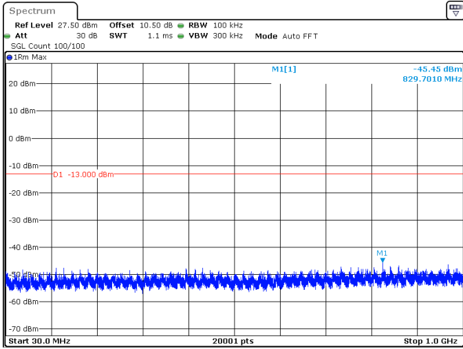
30MHz_15kHz_3715MHz_DFT-s-OFDM QPSK_RB1@159 -45.45 dBm
