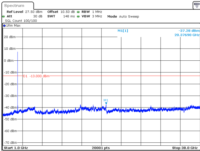
25MHz_30kHz_3787.5MHz_DFT-s-OFDM QPSK_RB1@0 -37.28 dBm
