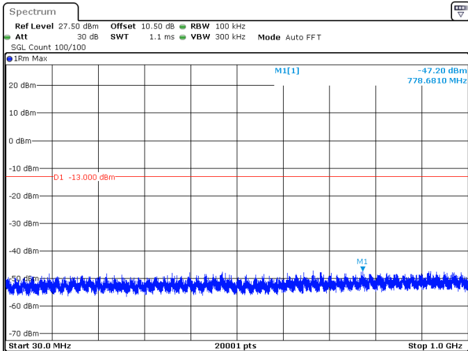
40MHz_30kHz_3750MHz_DFT-s-OFDM QPSK_RB100@0 -47.20 dBm
