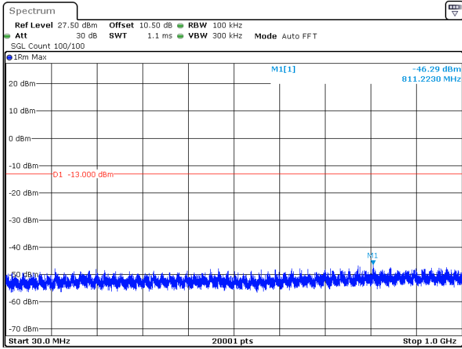
30MHz_15kHz_3785MHz_DFT-s-OFDM QPSK_RB1@159 -46.29 dBm
