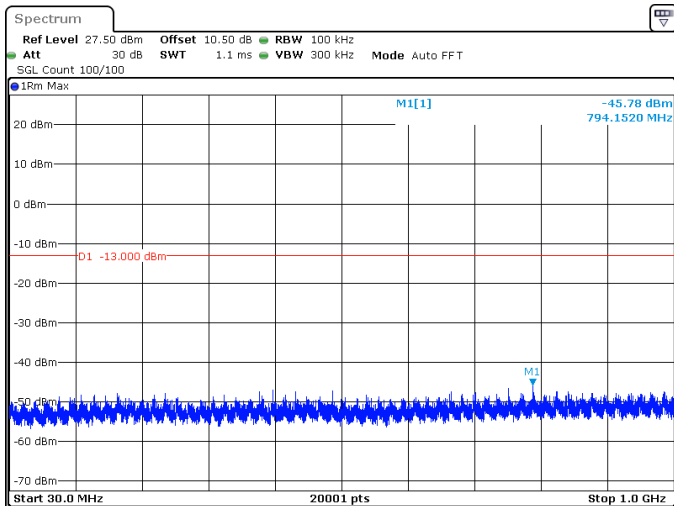
50MHz_30kHz_3775MHz_DFT-s-OFDM QPSK_RB128@0 -45.78 dBm
