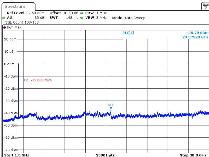
15MHz_30kHz_3792.5MHz_DFT-s-OFDM QPSK_RB36@0 -36.79 dBm
