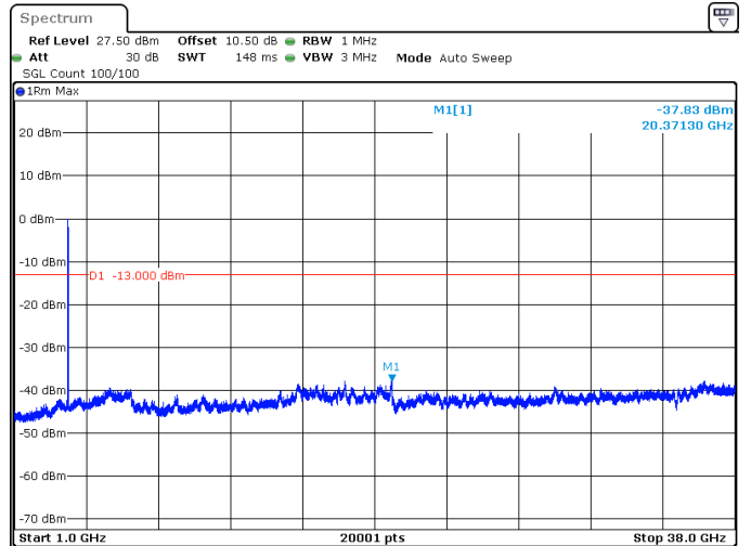
60MHz_30kHz_3730MHz_DFT-s-OFDM QPSK_RB162@0 -37.83 dBm
