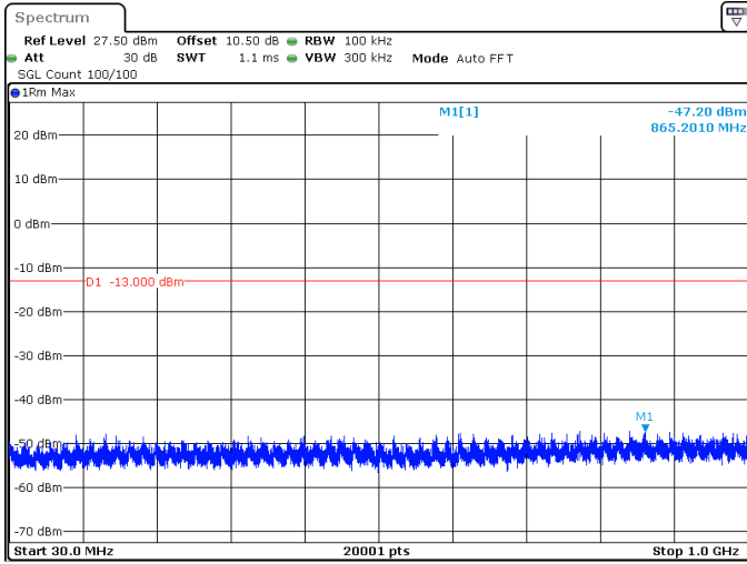
50MHz_30kHz_3725MHz_DFT-s-OFDM QPSK_RB1@132 -47.20 dBm
