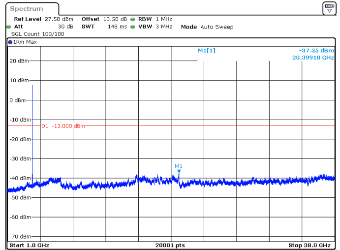
15MHz_30kHz_3792.5MHz_DFT-s-OFDM QPSK_RB1@37 -37.35 dBm
