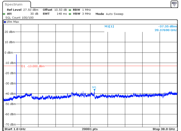
60MHz_30kHz_3750MHz_DFT-s-OFDM QPSK_RB162@0 -37.35 dBm
