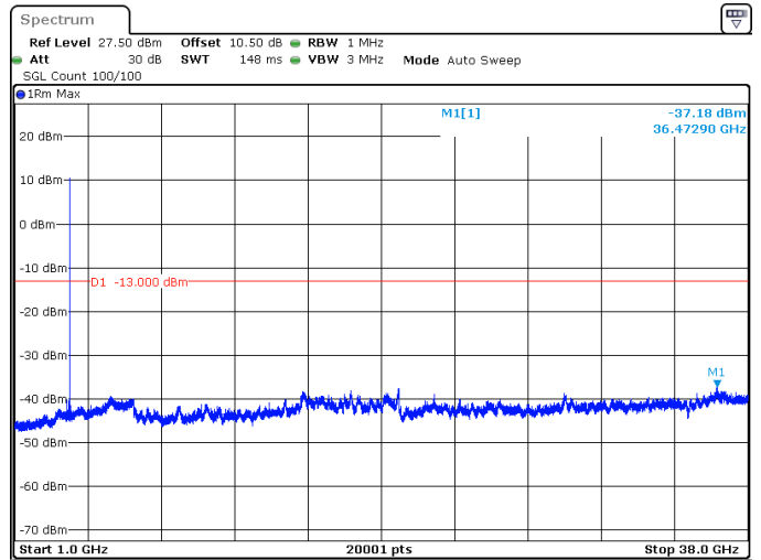
70MHz_30kHz_3735MHz_DFT-s-OFDM QPSK_RB1@188 -37.18 dBm
