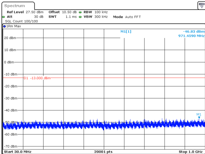
15MHz_30kHz_3750MHz_DFT-s-OFDM QPSK_RB36@0 -46.83 dBm
