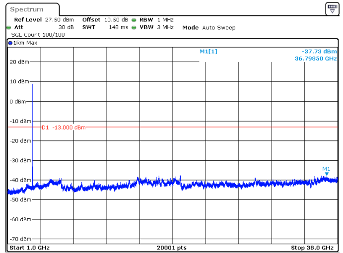
25MHz_15kHz_3787.5MHz_DFT-s-OFDM QPSK_RB1@0 -37.73 dBm
