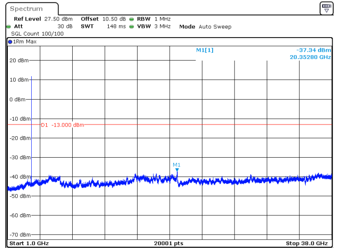
25MHz_15kHz_3712.5MHz_DFT-s-OFDM QPSK_RB1@132 -37.34 dBm
