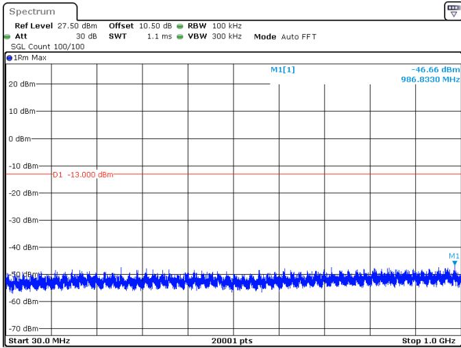
30MHz_15kHz_3785MHz_DFT-s-OFDM QPSK_RB1@0 -46.66 dBm
