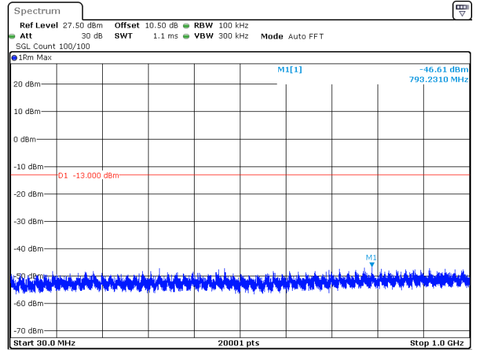
15MHz_30kHz_3750MHz_DFT-s-OFDM QPSK_RB1@37 -46.61 dBm
