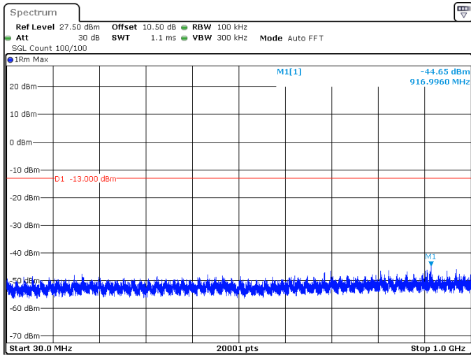
70MHz_30kHz_3735MHz_DFT-s-OFDM QPSK_RB1@188 -44.65 dBm
