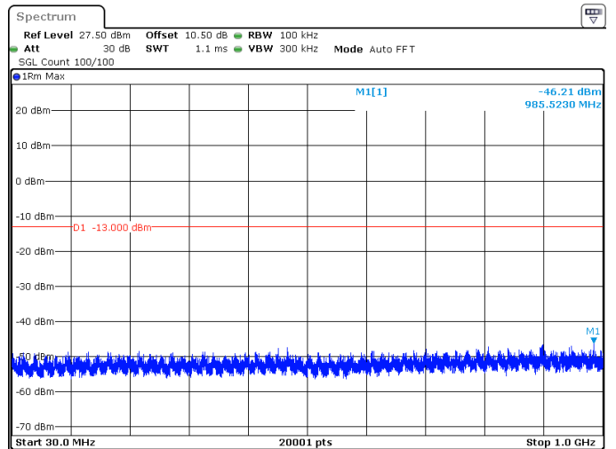
5MHz_15kHz_1777.5MHz_DFT-s-OFDM QPSK_RB25@0 -46.21 dBm
