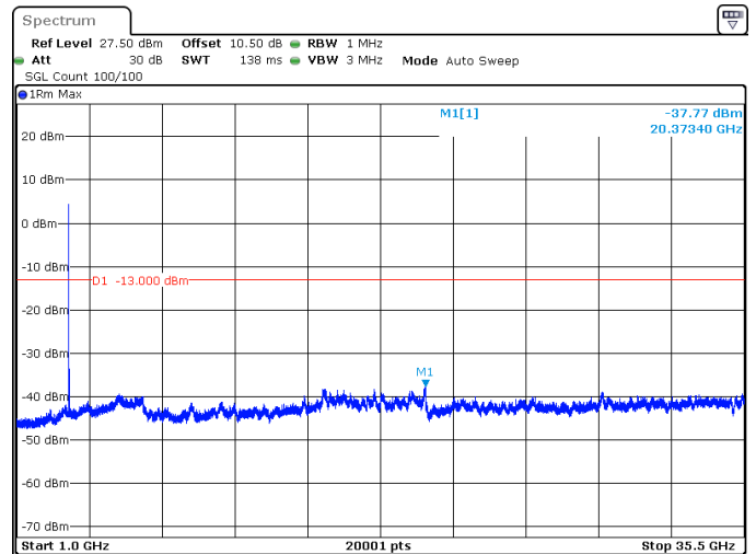
15MHz_30kHz_3457.5MHz_DFT-s-OFDM QPSK_RB36@0 -37.77 dBm
