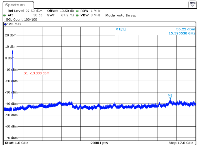
40MHz_15kHz_1745MHz_DFT-s-OFDM QPSK_RB216@0 -36.22 dBm
