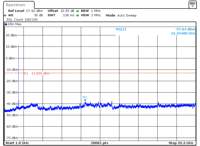
10MHz_30kHz_3545MHz_DFT-s-OFDM QPSK_RB1@0 -37.64 dBm
