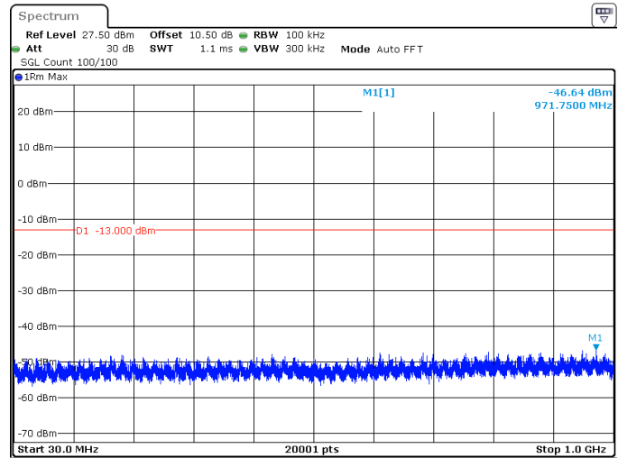
25MHz_15kHz_1767.5MHz_DFT-s-OFDM QPSK_RB1@132 -46.64 dBm
