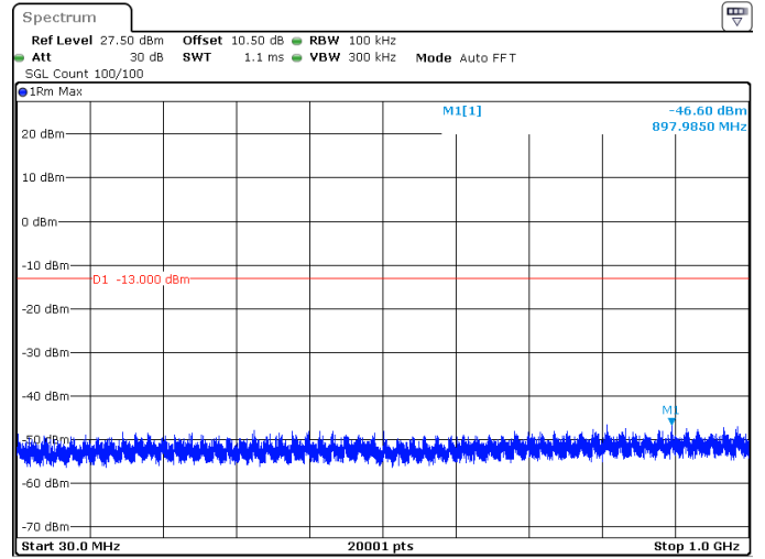
20MHz_15kHz_1745MHz_DFT-s-OFDM QPSK_RB1@105 -46.60 dBm
