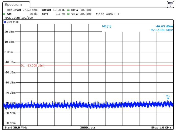
15MHz_30kHz_3542.5MHz_DFT-s-OFDM QPSK_RB1@37 -46.65 dBm
