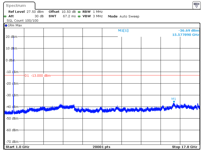
25MHz_15kHz_1767.5MHz_DFT-s-OFDM QPSK_RB1@0 -36.69 dBm
