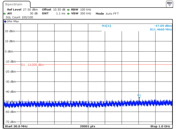
25MHz_15kHz_1722.5MHz_DFT-s-OFDM QPSK_RB1@0 -47.09 dBm
