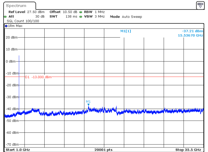
15MHz_30kHz_3500MHz_DFT-s-OFDM QPSK_RB36@0 -37.21 dBm
