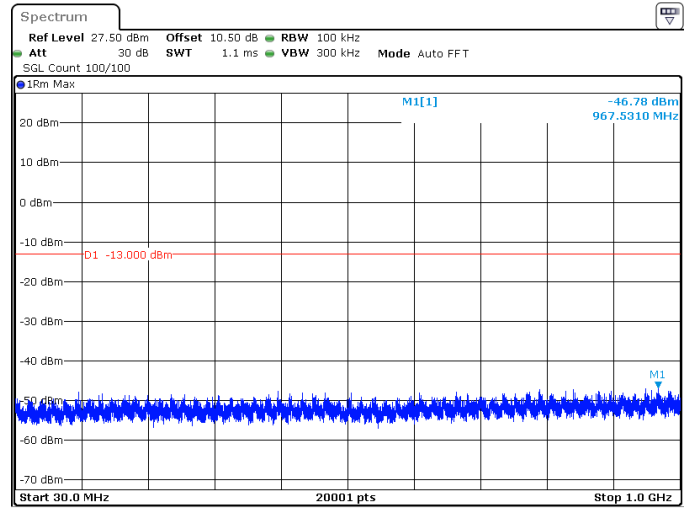
10MHz_15kHz_1745MHz_DFT-s-OFDM QPSK_RB1@0 -46.78 dBm
