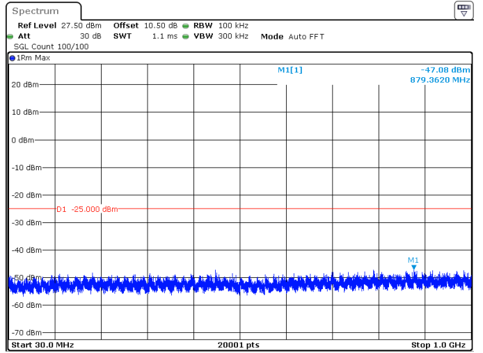
100MHz_30kHz_2592.99MHz_DFT-s-OFDM QPSK_RB1@272 -47.08 dBm
