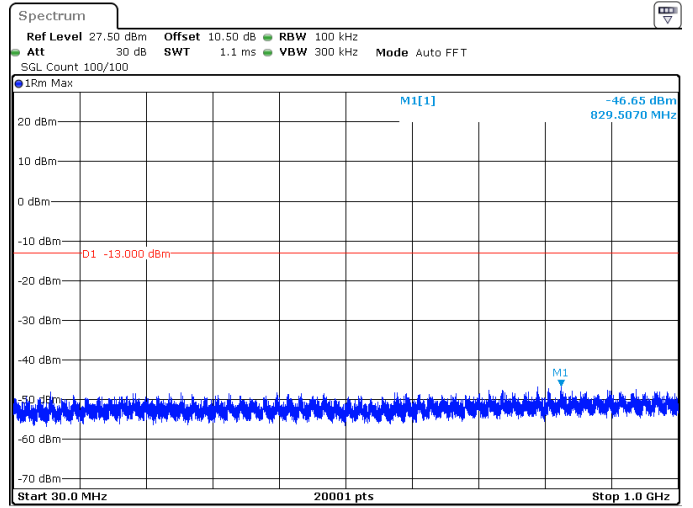
30MHz_15kHz_1745MHz_DFT-s-OFDM QPSK_RB1@159 -46.65 dBm
