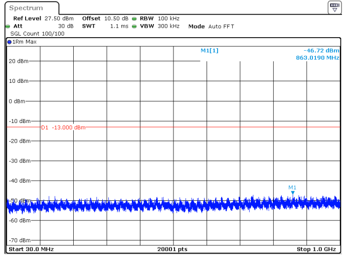
20MHz_15kHz_1720MHz_DFT-s-OFDM QPSK_RB1@105 -46.72 dBm
