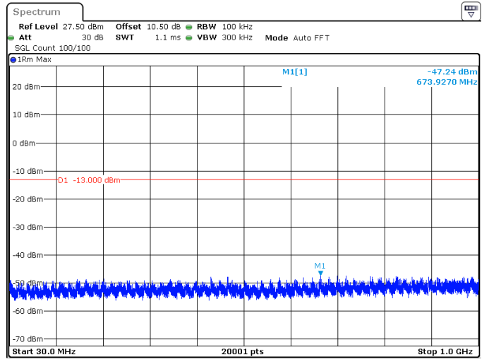
5MHz_15kHz_1777.5MHz_DFT-s-OFDM QPSK_RB1@0 -47.24 dBm
