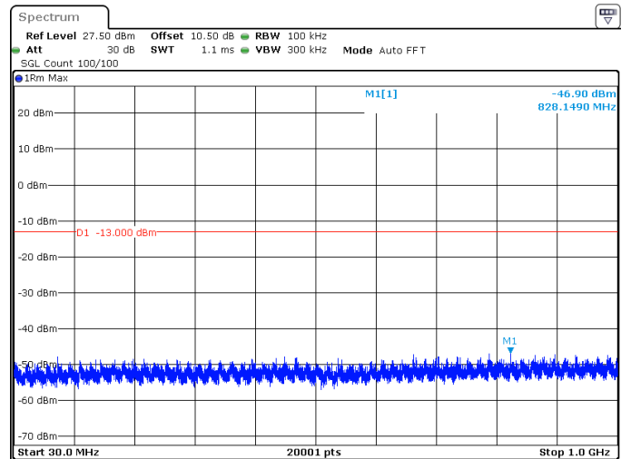
25MHz_15kHz_1722.5MHz_DFT-s-OFDM QPSK_RB128@0 -46.90 dBm
