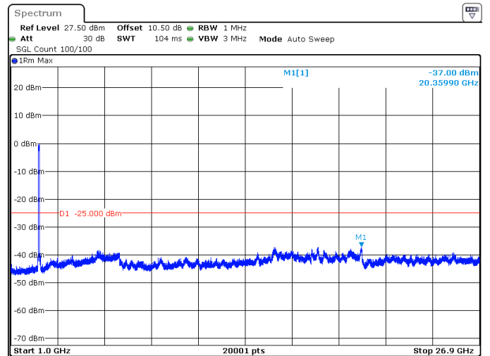
80MHz_30kHz_2536.02MHz_DFT-s-OFDM QPSK_RB216@0 -37.00 dBm
