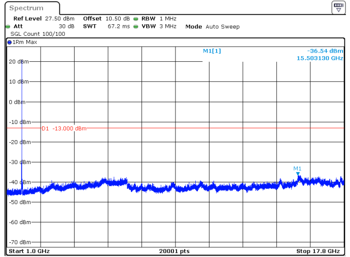
15MHz_15kHz_1745MHz_DFT-s-OFDM QPSK_RB1@78 -36.54 dBm
