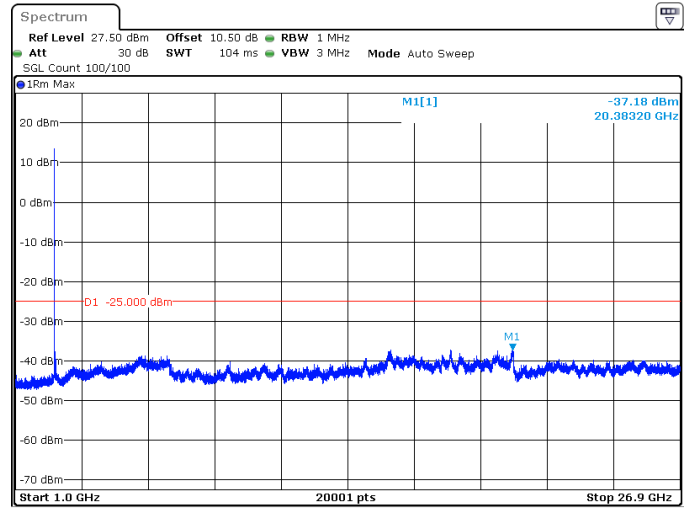
80MHz_30kHz_2536.02MHz_DFT-s-OFDM QPSK_RB1@0 -37.18 dBm
