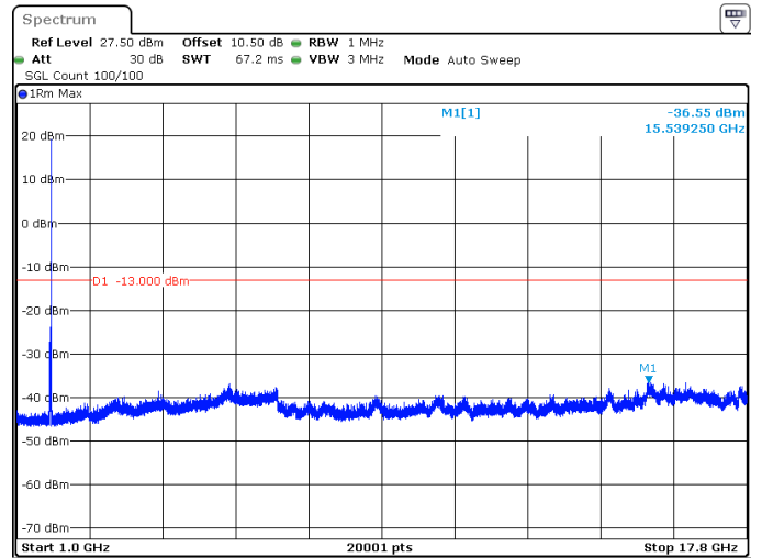
15MHz_15kHz_1772.5MHz_DFT-s-OFDM QPSK_RB1@78 -36.55 dBm
