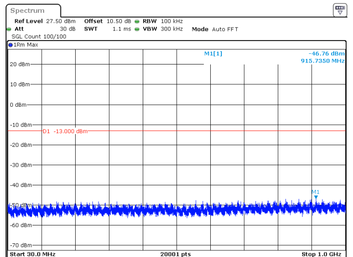
25MHz_15kHz_1767.5MHz_DFT-s-OFDM QPSK_RB128@0 -46.76 dBm
