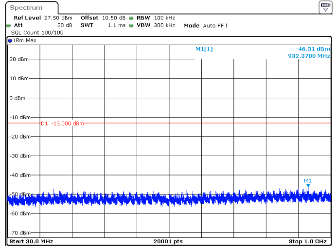
10MHz_15kHz_1745MHz_DFT-s-OFDM QPSK_RB1@51 -46.31 dBm
