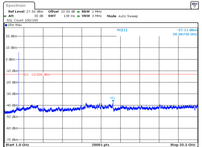
10MHz_30kHz_3545MHz_DFT-s-OFDM QPSK_RB24@0 -37.11 dBm
