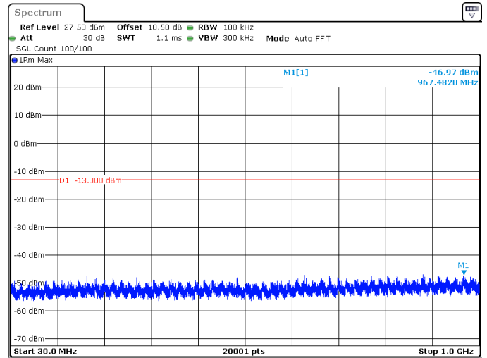
15MHz_30kHz_3457.5MHz_DFT-s-OFDM QPSK_RB1@37 -46.97 dBm
