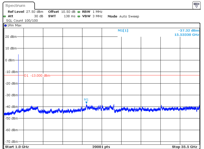
15MHz_30kHz_3542.5MHz_DFT-s-OFDM QPSK_RB36@0 -37.32 dBm
