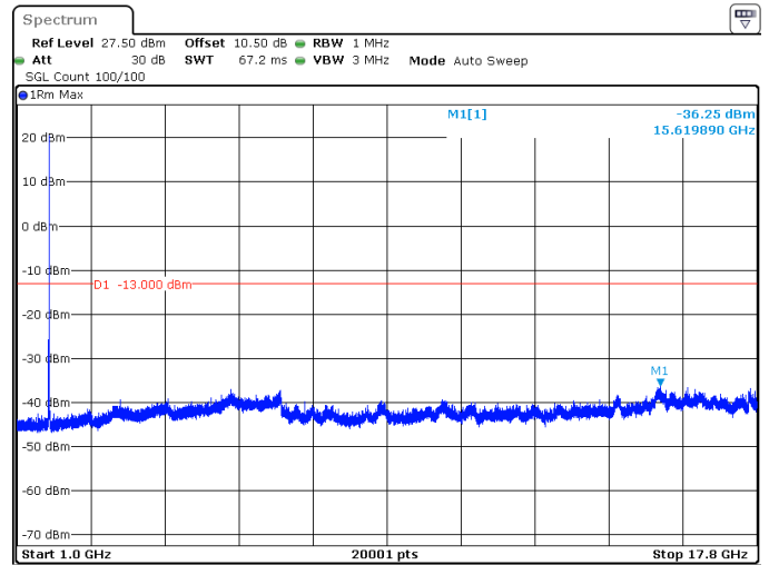
15MHz_15kHz_1717.5MHz_DFT-s-OFDM QPSK_RB1@78 -36.25 dBm
