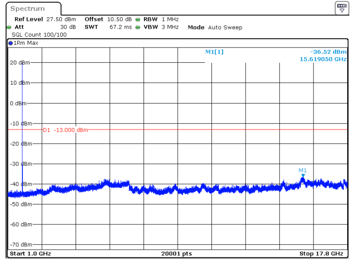
10MHz_15kHz_1715MHz_DFT-s-OFDM QPSK_RB1@0 -36.52 dBm
