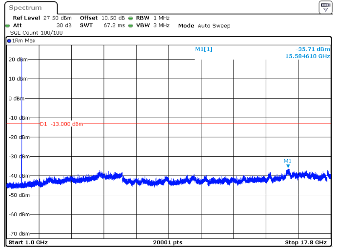
5MHz_15kHz_1777.5MHz_DFT-s-OFDM QPSK_RB1@24 -35.71 dBm
