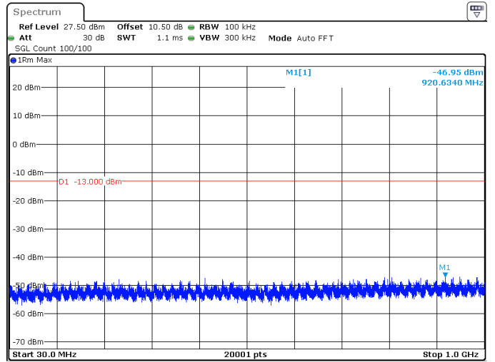
30MHz_15kHz_1745MHz_DFT-s-OFDM QPSK_RB1@0 -46.95 dBm
