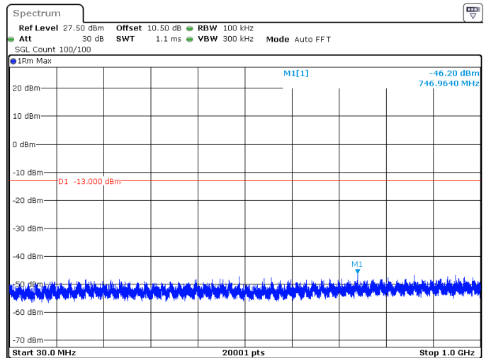
30MHz_15kHz_1745MHz_DFT-s-OFDM QPSK_RB160@0 -46.20 dBm
