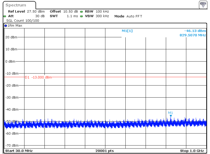
40MHz_15kHz_1745MHz_DFT-s-OFDM QPSK_RB1@0 -46.13 dBm
