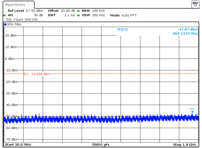
5MHz_15kHz_1712.5MHz_DFT-s-OFDM QPSK_RB1@24 -47.07 dBm
