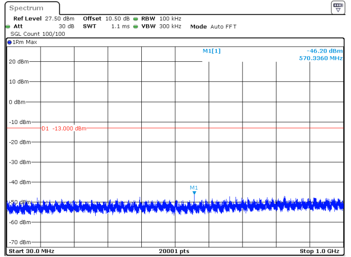
20MHz_15kHz_1770MHz_DFT-s-OFDM QPSK_RB1@105 -46.20 dBm
