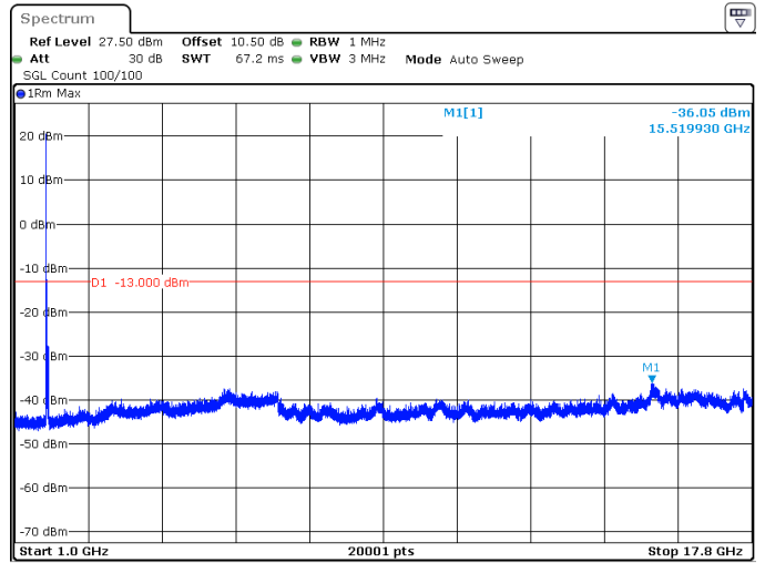
30MHz_15kHz_1725MHz_DFT-s-OFDM QPSK_RB1@0 -36.05 dBm
