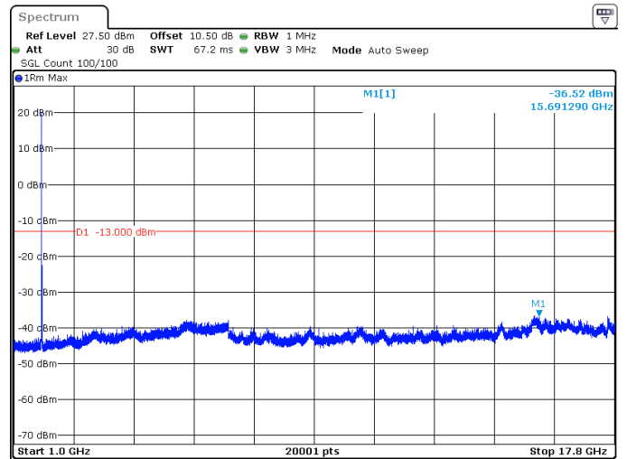
15MHz_15kHz_1772.5MHz_DFT-s-OFDM QPSK_RB1@0 -36.52 dBm
