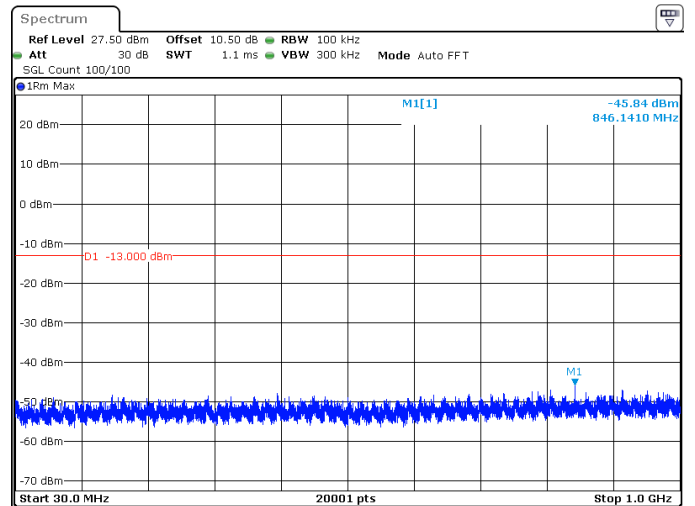
5MHz_15kHz_1745MHz_DFT-s-OFDM QPSK_RB25@0 -45.84 dBm
