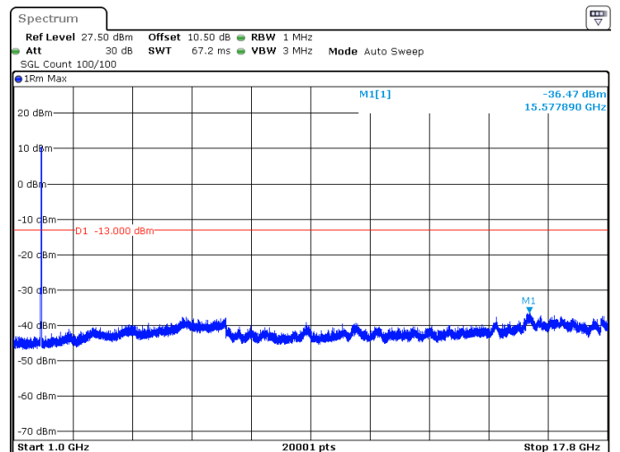
15MHz_15kHz_1772.5MHz_DFT-s-OFDM QPSK_RB75@0 -36.47 dBm
