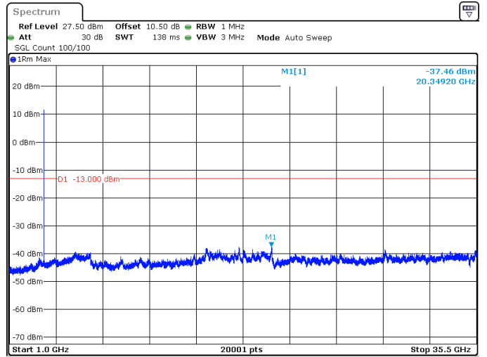
15MHz_30kHz_3542.5MHz_DFT-s-OFDM QPSK_RB1@0 -37.46 dBm
