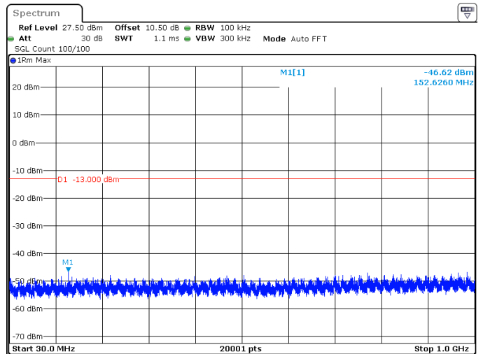
30MHz_15kHz_1725MHz_DFT-s-OFDM QPSK_RB160@0 -46.62 dBm
