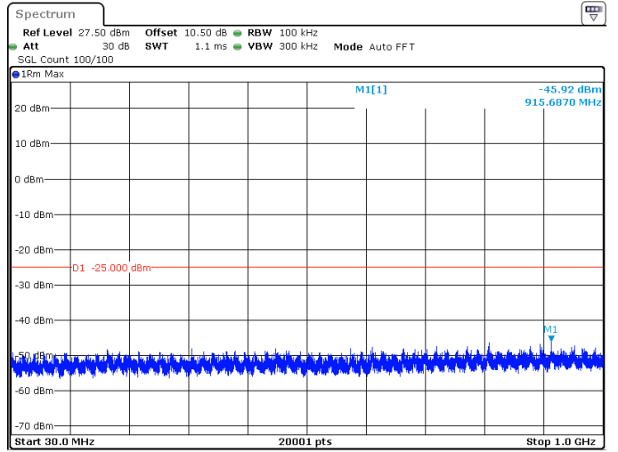
100MHz_30kHz_2546.01MHz_DFT-s-OFDM QPSK_RB1@272 -45.92 dBm
