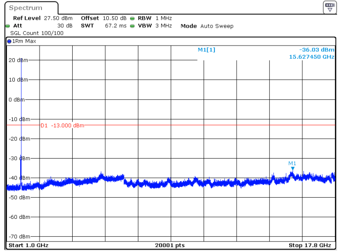
30MHz_15kHz_1725MHz_DFT-s-OFDM QPSK_RB1@159 -36.03 dBm
