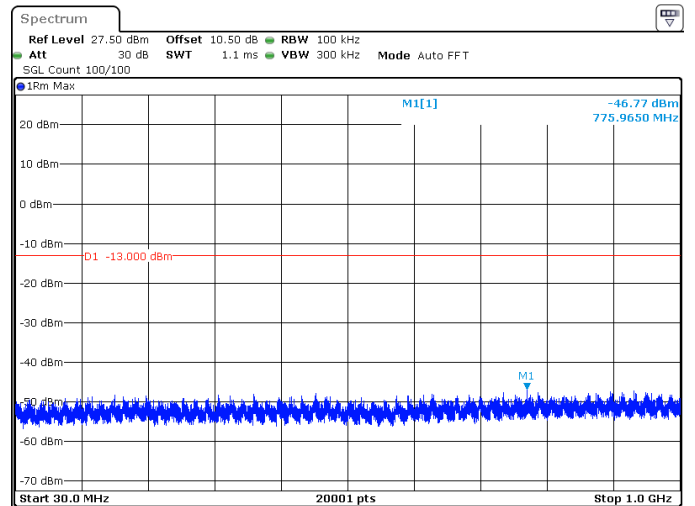
25MHz_15kHz_1745MHz_DFT-s-OFDM QPSK_RB128@0 -46.77 dBm
