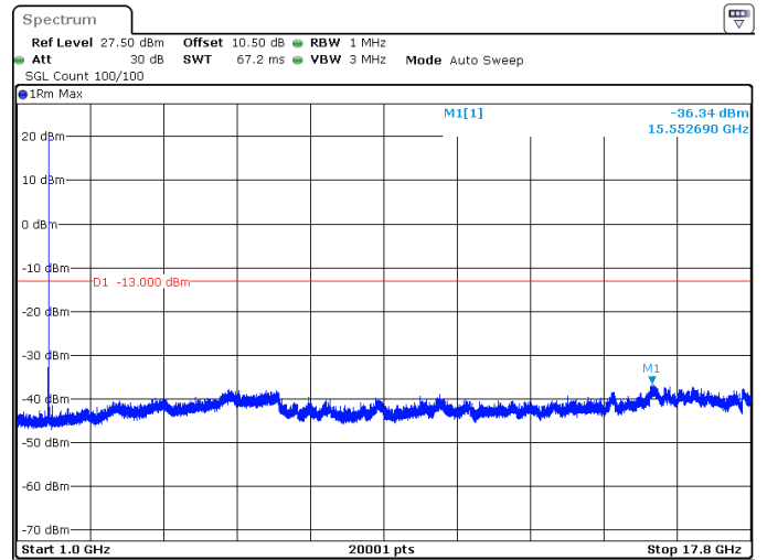
10MHz_15kHz_1715MHz_DFT-s-OFDM QPSK_RB1@51 -36.34 dBm
