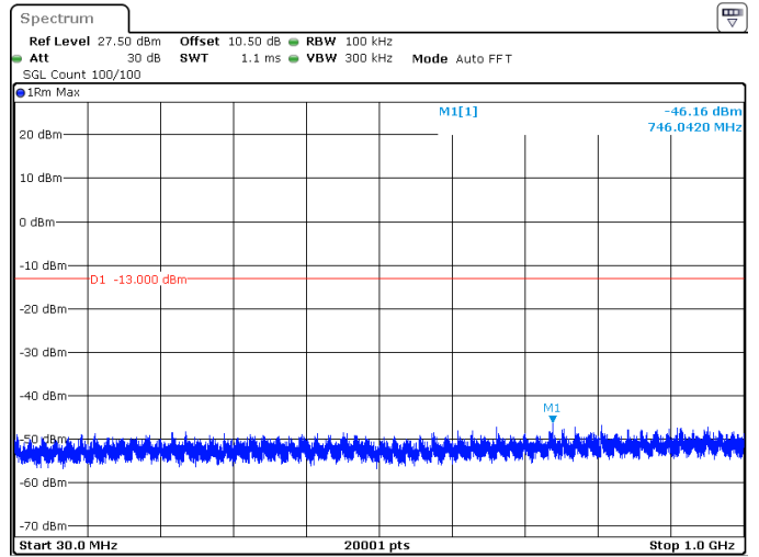
40MHz_15kHz_1760MHz_DFT-s-OFDM QPSK_RB1@0 -46.16 dBm
