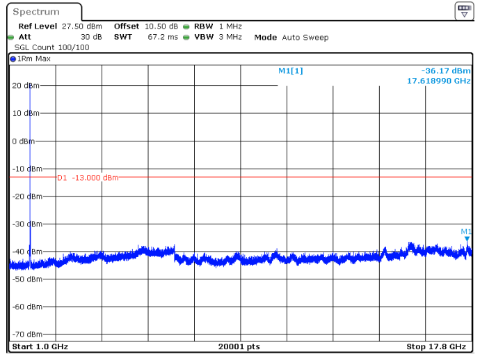
15MHz_15kHz_1745MHz_DFT-s-OFDM QPSK_RB1@0 -36.17 dBm
