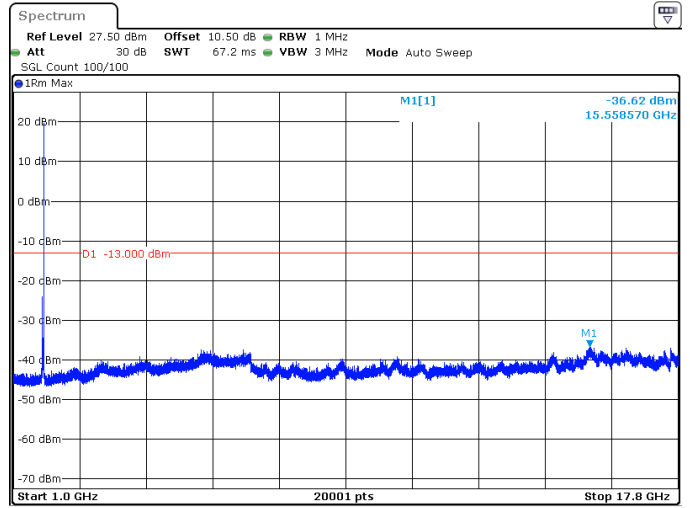
40MHz_15kHz_1745MHz_DFT-s-OFDM QPSK_RB1@215 -36.62 dBm
