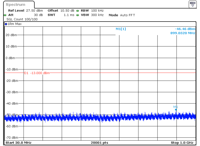
25MHz_15kHz_1722.5MHz_DFT-s-OFDM QPSK_RB1@132 -46.46 dBm
