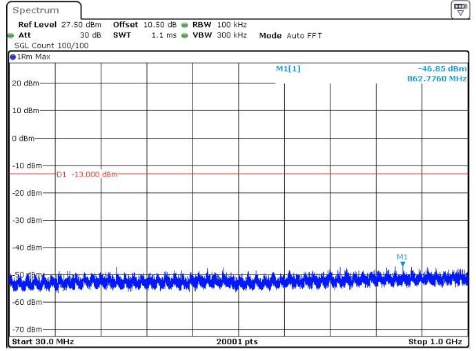
5MHz_15kHz_1712.5MHz_DFT-s-OFDM QPSK_RB1@0 -46.85 dBm
