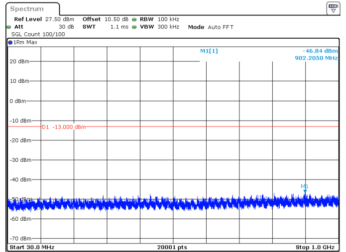
5MHz_15kHz_1745MHz_DFT-s-OFDM QPSK_RB1@24 -46.84 dBm
