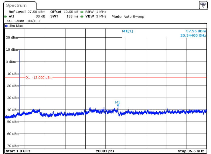
10MHz_30kHz_3545MHz_DFT-s-OFDM QPSK_RB1@23 -37.25 dBm
