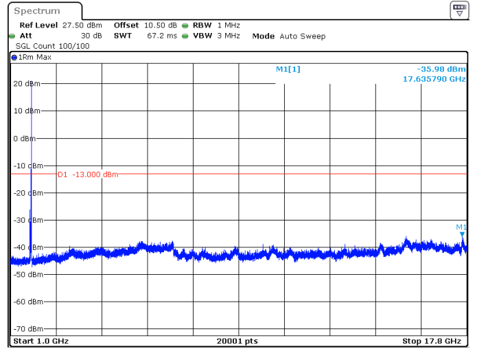
25MHz_15kHz_1745MHz_DFT-s-OFDM QPSK_RB1@132 -35.98 dBm
