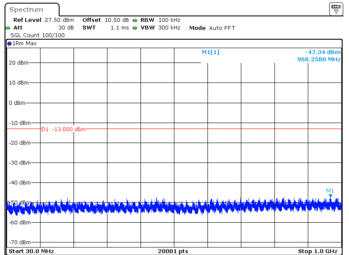
40MHz_15kHz_1730MHz_DFT-s-OFDM QPSK_RB216@0 -47.34 dBm
