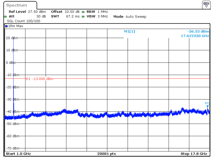
15MHz_15kHz_1717.5MHz_DFT-s-OFDM QPSK_RB1@0 -36.53 dBm
