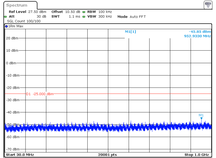
90MHz_30kHz_2592.99MHz_DFT-s-OFDM QPSK_RB1@0 -45.85 dBm
