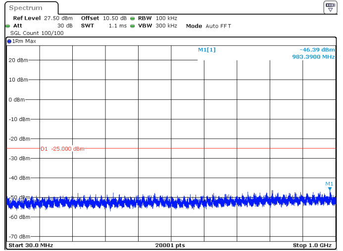
80MHz_30kHz_2592.99MHz_DFT-s-OFDM QPSK_RB1@216 -46.39 dBm
