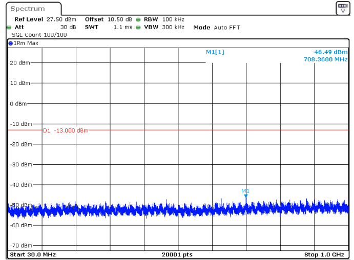
15MHz_30kHz_3457.5MHz_DFT-s-OFDM QPSK_RB1@0 -46.49 dBm
