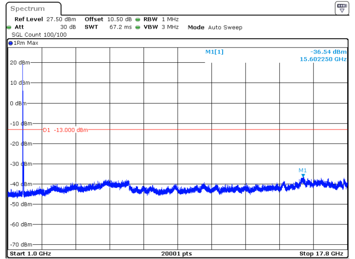
25MHz_15kHz_1745MHz_DFT-s-OFDM QPSK_RB1@0 -36.54 dBm
