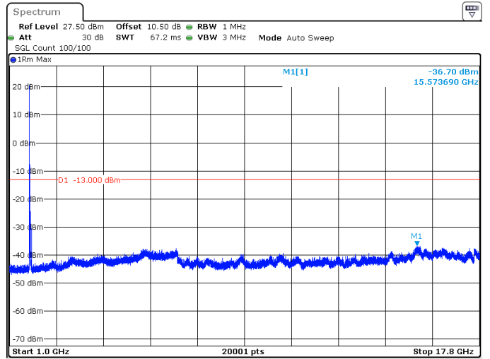
40MHz_15kHz_1730MHz_DFT-s-OFDM QPSK_RB1@0 -36.70 dBm
