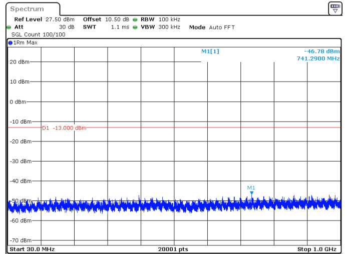
15MHz_30kHz_3500MHz_DFT-s-OFDM QPSK_RB1@37 -46.78 dBm
