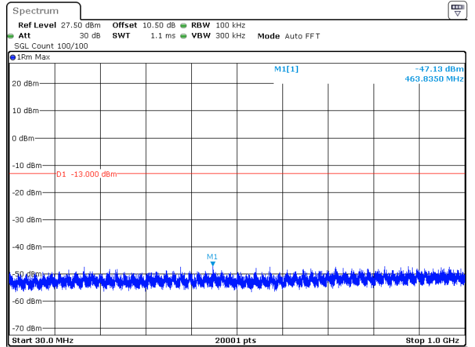
40MHz_15kHz_1730MHz_DFT-s-OFDM QPSK_RB1@215 -47.13 dBm
