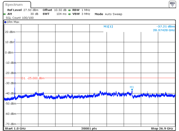
90MHz_30kHz_2592.99MHz_DFT-s-OFDM QPSK_RB1@244 -37.21 dBm
