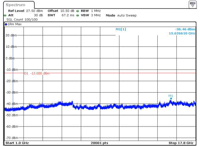
5MHz_15kHz_1745MHz_DFT-s-OFDM QPSK_RB1@0 -36.46 dBm
