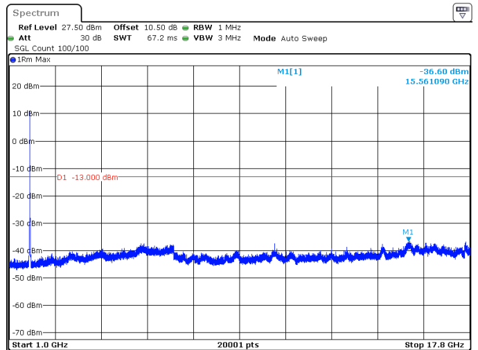
15MHz_15kHz_1745MHz_DFT-s-OFDM QPSK_RB75@0 -36.60 dBm
