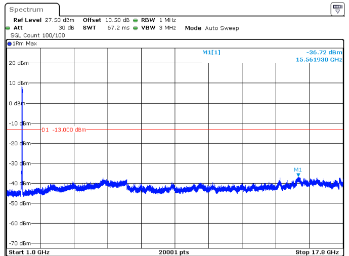
30MHz_15kHz_1765MHz_DFT-s-OFDM QPSK_RB160@0 -36.72 dBm
