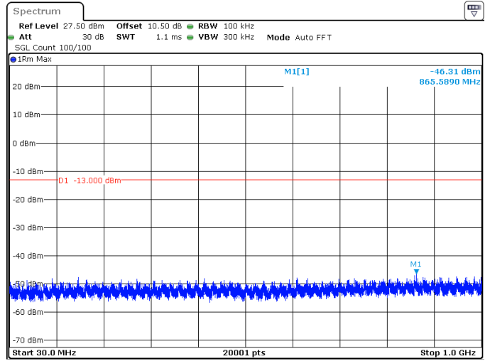
10MHz_15kHz_1775MHz_DFT-s-OFDM QPSK_RB1@51 -46.31 dBm
