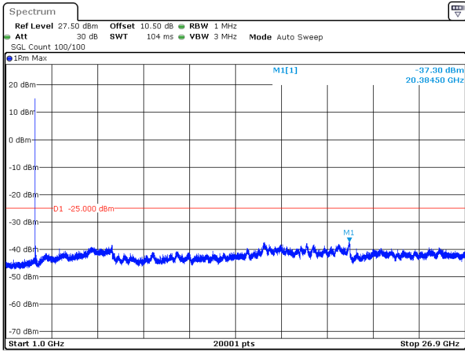
50MHz_15kHz_2664.99MHz_DFT-s-OFDM QPSK_RB1@0 -37.30 dBm
