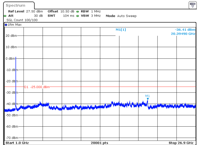
50MHz_30kHz_2521.02MHz_DFT-s-OFDM QPSK_RB128@0 -36.41 dBm
