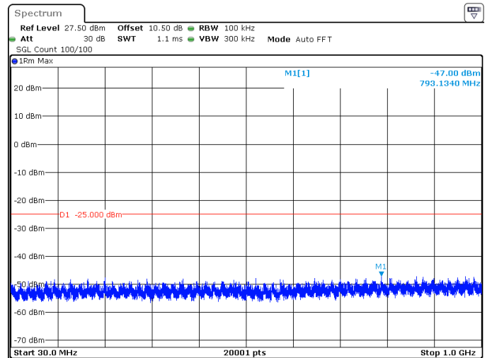
40MHz_30kHz_2592.99MHz_DFT-s-OFDM QPSK_RB100@0 -47.00 dBm
