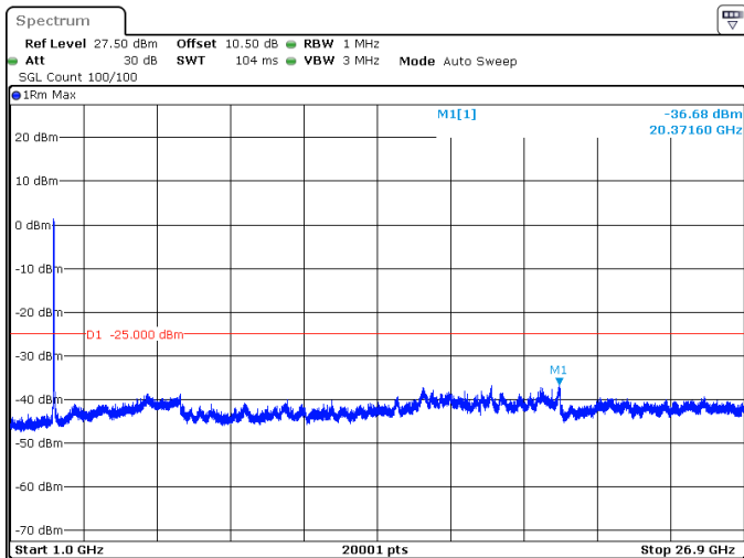
60MHz_30kHz_2526MHz_DFT-s-OFDM QPSK_RB162@0 -36.68 dBm
