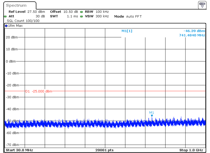
40MHz_30kHz_2592.99MHz_DFT-s-OFDM QPSK_RB1@105 -46.39 dBm
