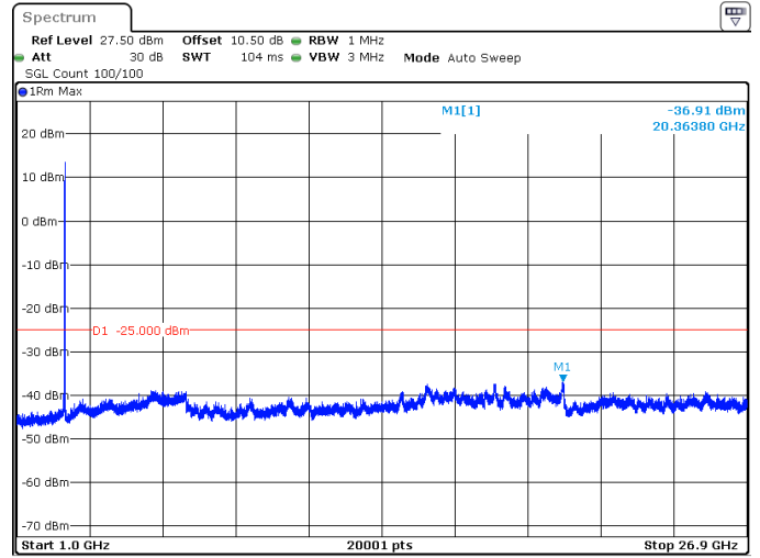
50MHz_30kHz_2664.99MHz_DFT-s-OFDM QPSK_RB1@132 -36.91 dBm
