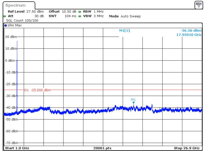
30MHz_15kHz_2674.995MHz_DFT-s-OFDM QPSK_RB1@159 -36.56 dBm
