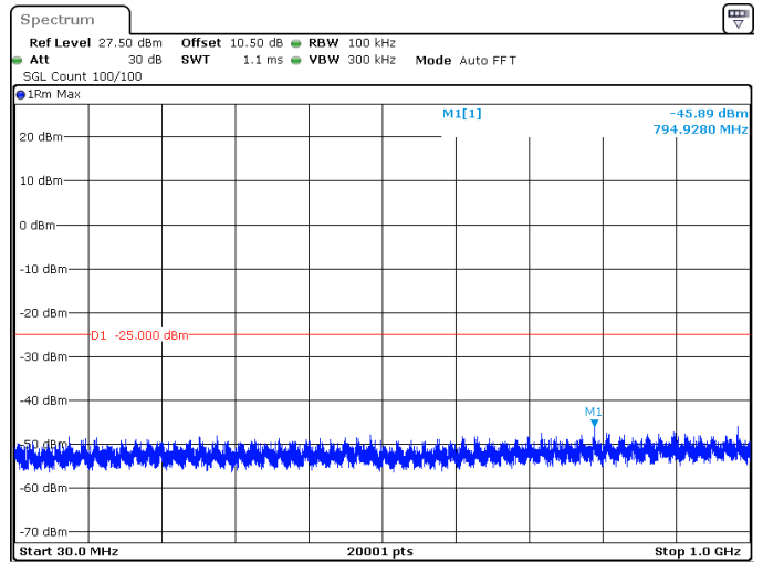
15MHz_15kHz_2503.5MHz_DFT-s-OFDM QPSK_RB1@78 -45.89 dBm
