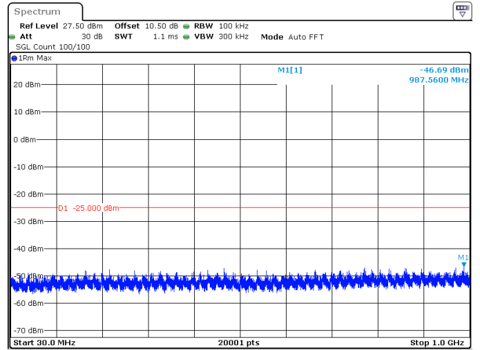
40MHz_30kHz_2592.99MHz_DFT-s-OFDM QPSK_RB1@0 -46.69 dBm
