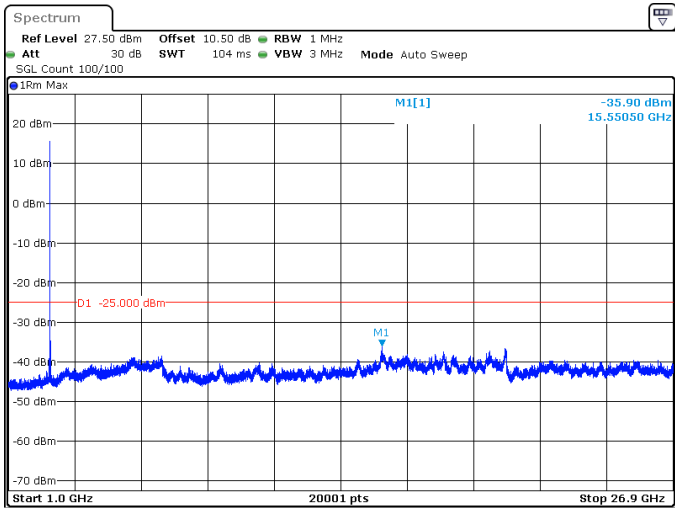
40MHz_15kHz_2593.005MHz_DFT-s-OFDM QPSK_RB1@215 -35.90 dBm
