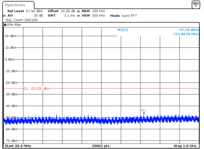
15MHz_15kHz_2593.005MHz_DFT-s-OFDM QPSK_RB1@0 -47.28 dBm
