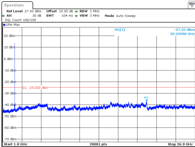
30MHz_30kHz_2592.99MHz_DFT-s-OFDM QPSK_RB1@77 -37.32 dBm
