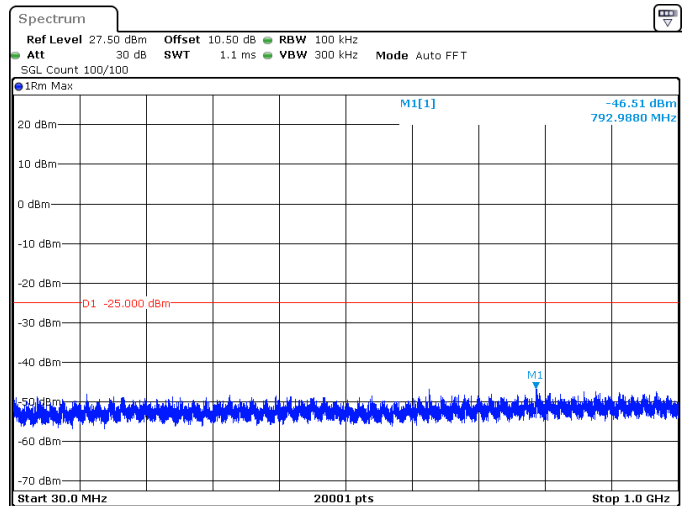
30MHz_15kHz_2511MHz_DFT-s-OFDM QPSK_RB160@0 -46.51 dBm
