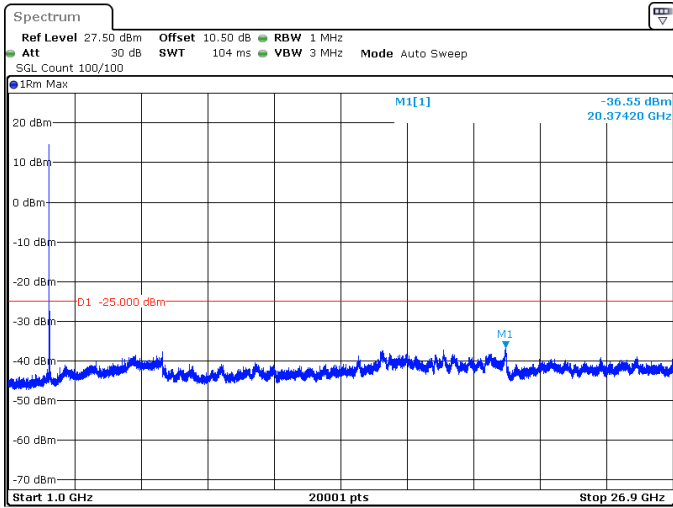
15MHz_30kHz_2592.99MHz_DFT-s-OFDM QPSK_RB1@0 -36.55 dBm
