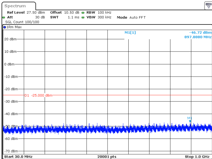
60MHz_30kHz_2592.99MHz_DFT-s-OFDM QPSK_RB162@0 -46.72 dBm
