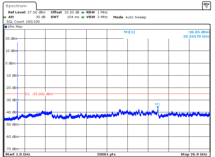
30MHz_15kHz_2674.995MHz_DFT-s-OFDM QPSK_RB1@0 -36.85 dBm
