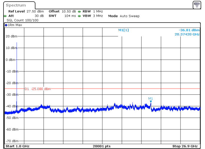
15MHz_15kHz_2593.005MHz_DFT-s-OFDM QPSK_RB1@78 -36.81 dBm
