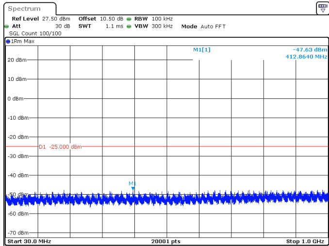
15MHz_15kHz_2593.005MHz_DFT-s-OFDM QPSK_RB1@78 -47.63 dBm
