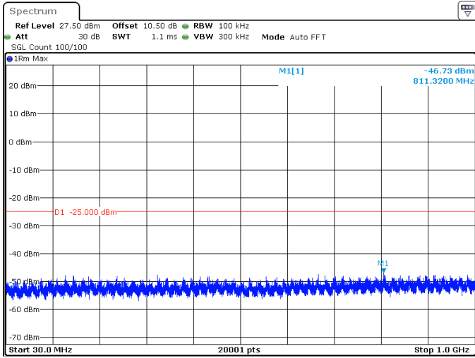
50MHz_30kHz_2521.02MHz_DFT-s-OFDM QPSK_RB1@132 -46.73 dBm
