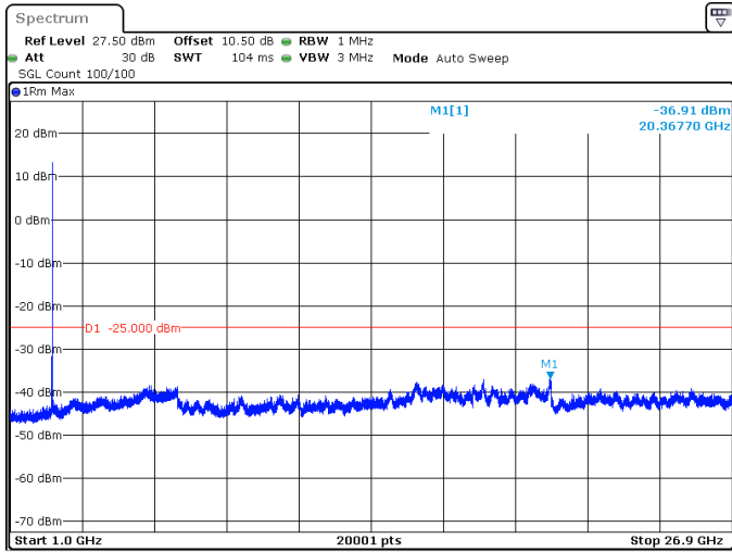
30MHz_15kHz_2511MHz_DFT-s-OFDM QPSK_RB1@0 -36.91 dBm
