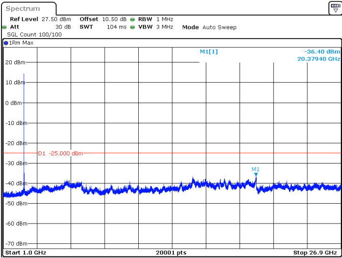
15MHz_15kHz_2593.005MHz_DFT-s-OFDM QPSK_RB1@0 -36.40 dBm
