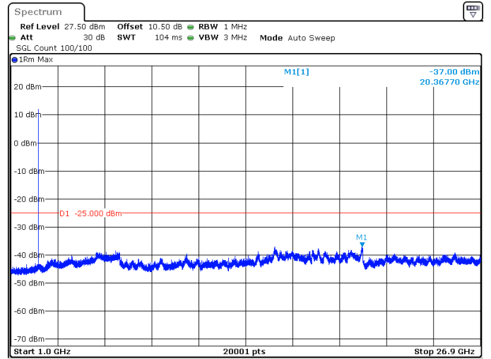
15MHz_30kHz_2503.5MHz_DFT-s-OFDM QPSK_RB1@0 -37.00 dBm
