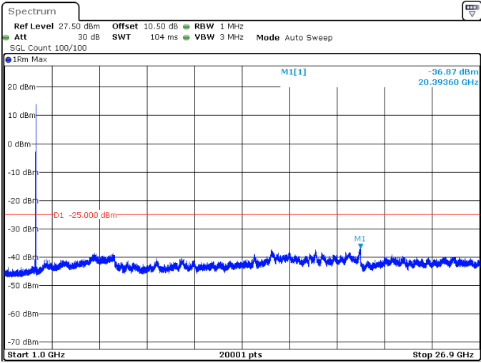
15MHz_15kHz_2682.495MHz_DFT-s-OFDM QPSK_RB1@78 -36.87 dBm
