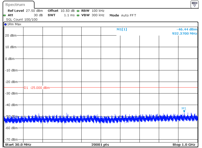
15MHz_30kHz_2682.48MHz_DFT-s-OFDM QPSK_RB1@37 -46.44 dBm
