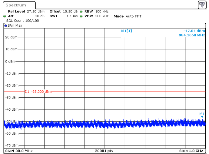
30MHz_15kHz_2511MHz_DFT-s-OFDM QPSK_RB1@0 -47.04 dBm
