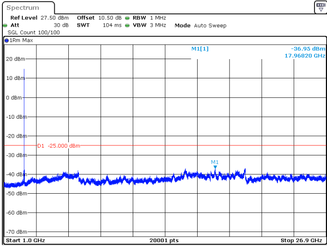
30MHz_15kHz_2593.005MHz_DFT-s-OFDM QPSK_RB1@159 -36.95 dBm
