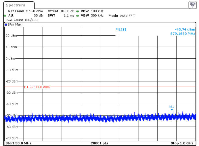
30MHz_30kHz_2592.99MHz_DFT-s-OFDM QPSK_RB1@77 -45.74 dBm
