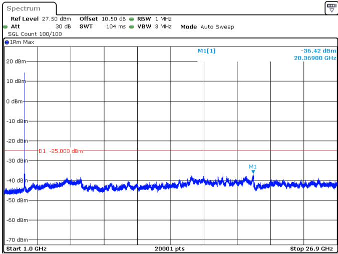
50MHz_15kHz_2593.005MHz_DFT-s-OFDM QPSK_RB1@0 -36.42 dBm
