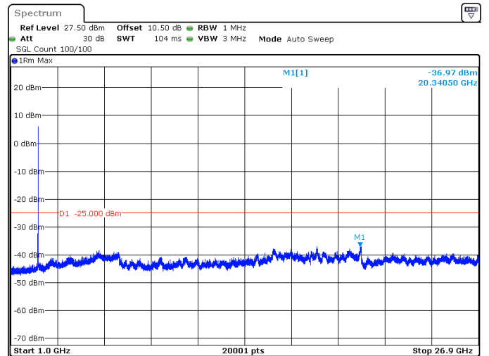
15MHz_30kHz_2503.5MHz_DFT-s-OFDM QPSK_RB36@0 -36.97 dBm
