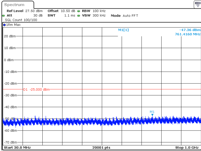
50MHz_30kHz_2664.99MHz_DFT-s-OFDM QPSK_RB1@132 -47.36 dBm
