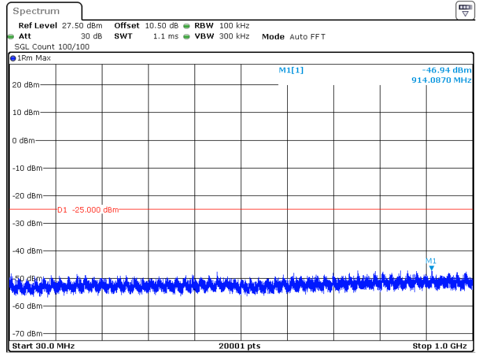
60MHz_30kHz_2526MHz_DFT-s-OFDM QPSK_RB1@161 -46.94 dBm
