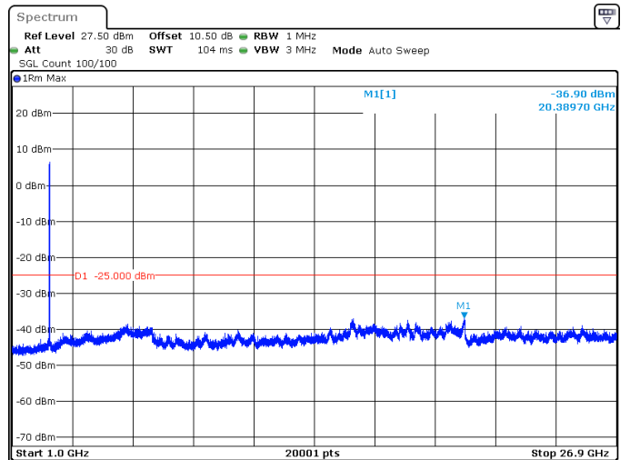
15MHz_30kHz_2592.99MHz_DFT-s-OFDM QPSK_RB36@0 -36.90 dBm
