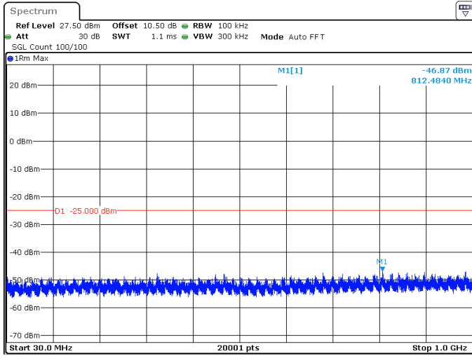
40MHz_30kHz_2516.01MHz_DFT-s-OFDM QPSK_RB1@105 -46.87 dBm
