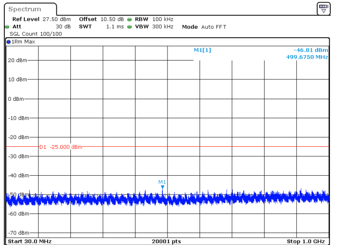
30MHz_15kHz_2593.005MHz_DFT-s-OFDM QPSK_RB160@0 -46.81 dBm
