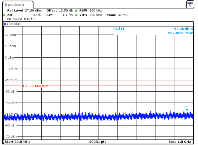
15MHz_15kHz_2682.495MHz_DFT-s-OFDM QPSK_RB1@78 -47.05 dBm
