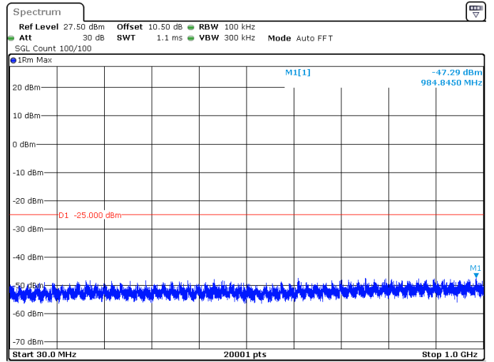
50MHz_15kHz_2664.99MHz_DFT-s-OFDM QPSK_RB1@0 -47.29 dBm
