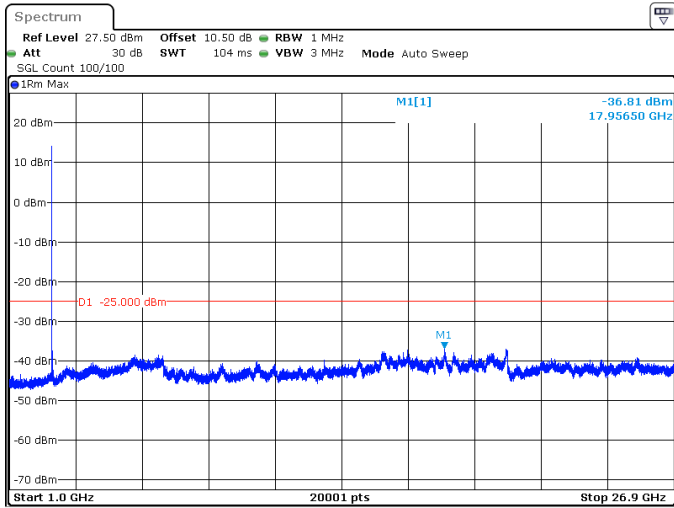
50MHz_30kHz_2664.99MHz_DFT-s-OFDM QPSK_RB1@0 -36.81 dBm
