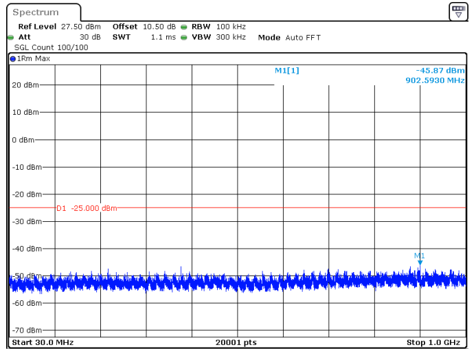
15MHz_30kHz_2592.99MHz_DFT-s-OFDM QPSK_RB1@37 -45.87 dBm
