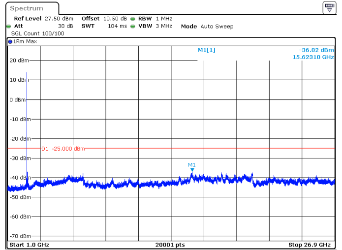
50MHz_30kHz_2521.02MHz_DFT-s-OFDM QPSK_RB1@0 -36.82 dBm
