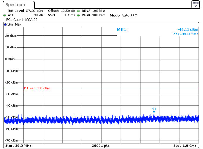
50MHz_15kHz_2664.99MHz_DFT-s-OFDM QPSK_RB1@269 -46.11 dBm
