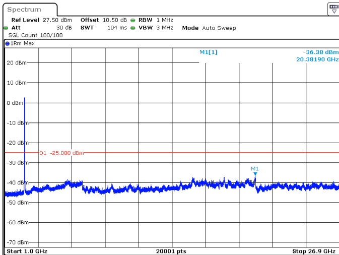
40MHz_30kHz_2516.01MHz_DFT-s-OFDM QPSK_RB100@0 -36.38 dBm
