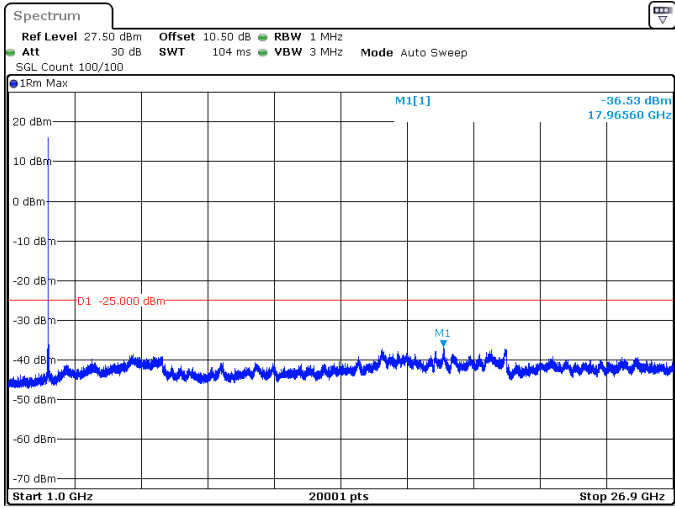
50MHz_15kHz_2521.005MHz_DFT-s-OFDM QPSK_RB1@269 -36.53 dBm
