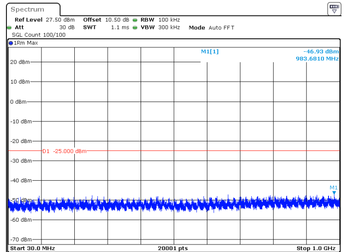
40MHz_30kHz_2516.01MHz_DFT-s-OFDM QPSK_RB100@0 -46.93 dBm
