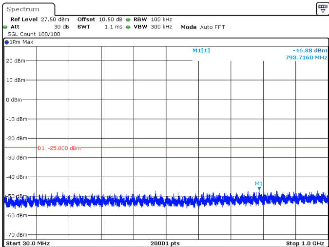
50MHz_15kHz_2593.005MHz_DFT-s-OFDM QPSK_RB270@0 -46.88 dBm
