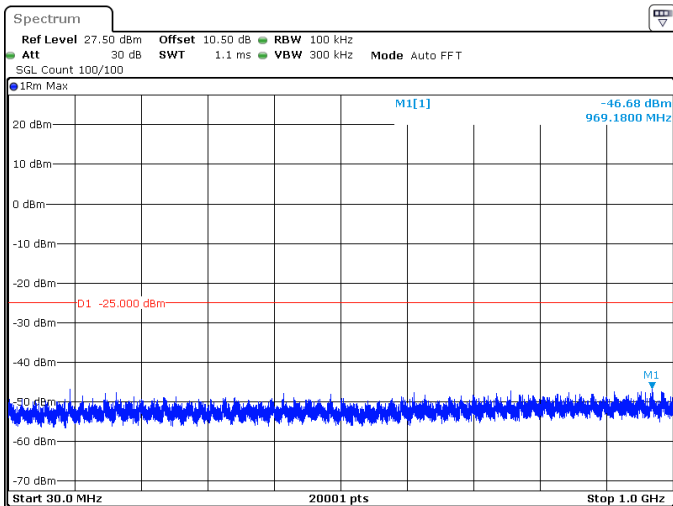
50MHz_30kHz_2521.02MHz_DFT-s-OFDM QPSK_RB128@0 -46.68 dBm
