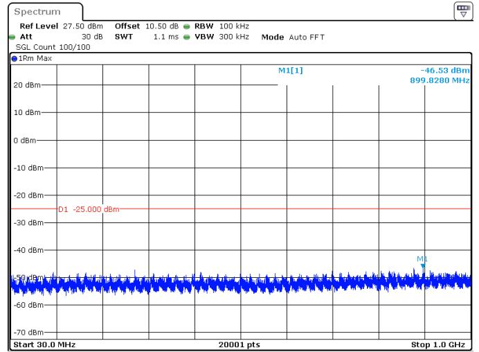
50MHz_30kHz_2664.99MHz_DFT-s-OFDM QPSK_RB1@0 -46.53 dBm
