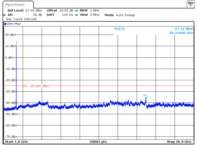
40MHz_30kHz_2670MHz_DFT-s-OFDM QPSK_RB1@105 -37.12 dBm
