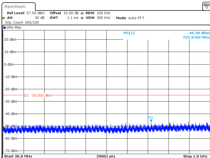
15MHz_15kHz_2503.5MHz_DFT-s-OFDM QPSK_RB75@0 -46.30 dBm
