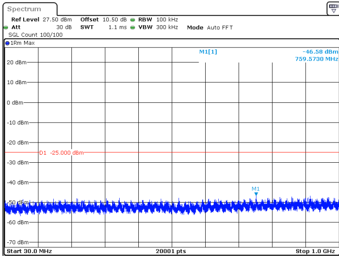
15MHz_30kHz_2503.5MHz_DFT-s-OFDM QPSK_RB1@37 -46.58 dBm
