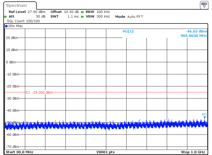
60MHz_30kHz_2592.99MHz_DFT-s-OFDM QPSK_RB1@161 -46.65 dBm
