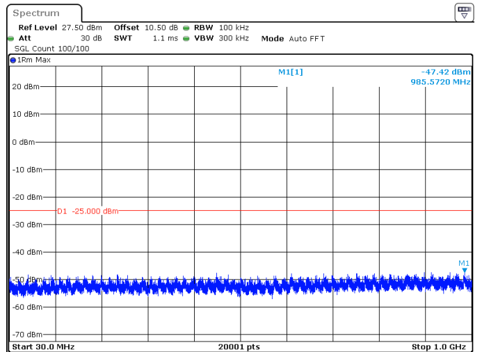
60MHz_30kHz_2526MHz_DFT-s-OFDM QPSK_RB162@0 -47.42 dBm
