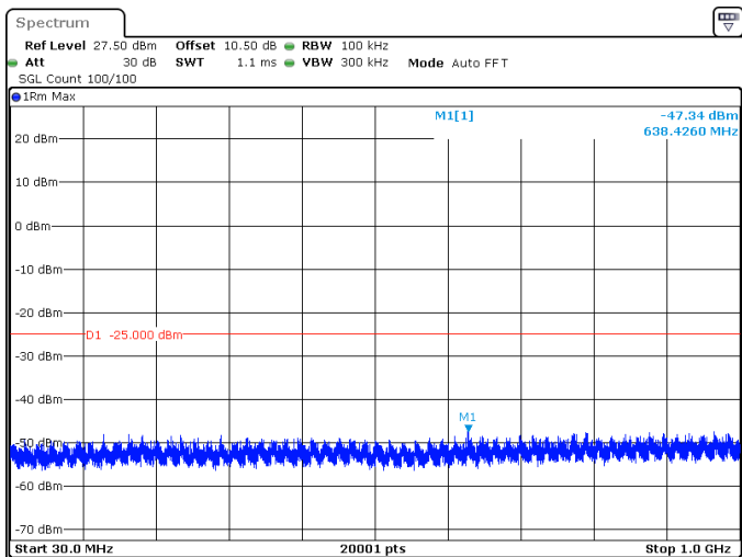
30MHz_15kHz_2674.995MHz_DFT-s-OFDM QPSK_RB160@0 -47.34 dBm
