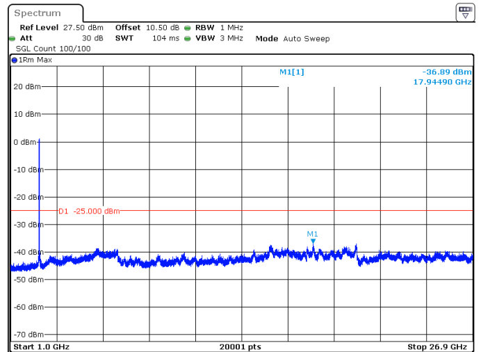
50MHz_30kHz_2592.99MHz_DFT-s-OFDM QPSK_RB128@0 -36.89 dBm
