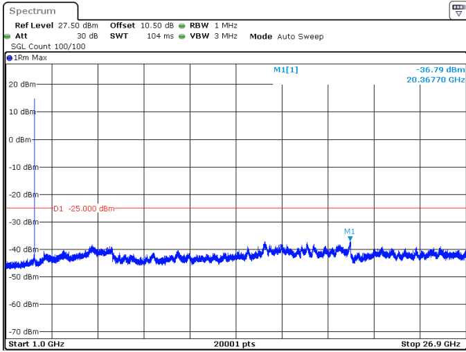
50MHz_30kHz_2592.99MHz_DFT-s-OFDM QPSK_RB1@132 -36.79 dBm
