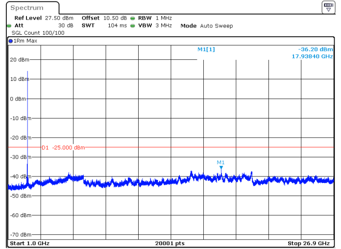
40MHz_30kHz_2516.01MHz_DFT-s-OFDM QPSK_RB1@105 -36.20 dBm
