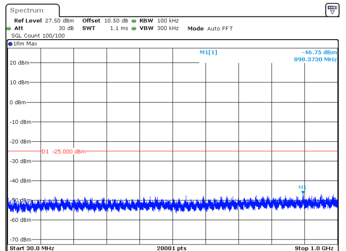
15MHz_15kHz_2593.005MHz_DFT-s-OFDM QPSK_RB75@0 -46.75 dBm
