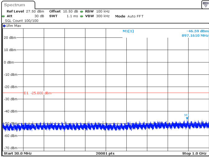
10MHz_30kHz_2592.99MHz_DFT-s-OFDM QPSK_RB1@23 -46.59 dBm
