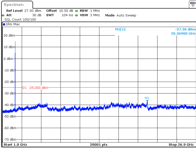
15MHz_30kHz_2682.48MHz_DFT-s-OFDM QPSK_RB1@37 -37.36 dBm
