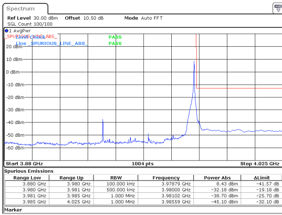
50MHz_30kHz_3955MHz_DFT-s-OFDM QPSK_RB1@132&-32.18 dBm
