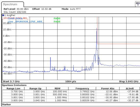
50MHz_15kHz_3775MHz_DFT-s-OFDM QPSK_RB1@269&-22.61 dBm
