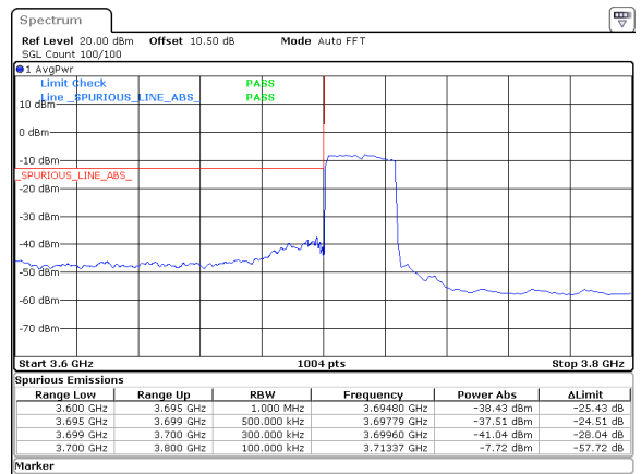
25MHz_15kHz_3712.5MHz_DFT-s-OFDM QPSK_RB128@0&-37.51 dBm
