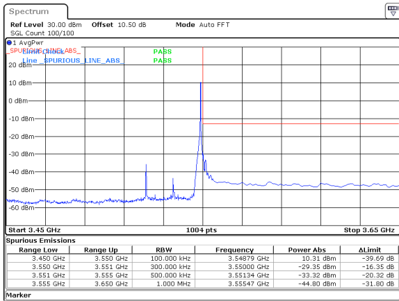
30MHz_30kHz_3535MHz_DFT-s-OFDM QPSK_RB1@77&-29.35 dBm
