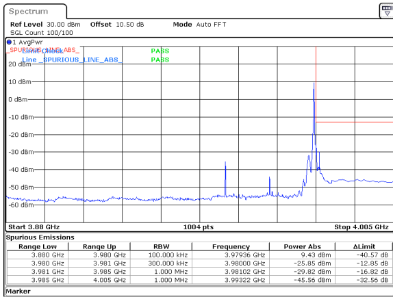
30MHz_15kHz_3965MHz_DFT-s-OFDM QPSK_RB1@159&-25.85 dBm
