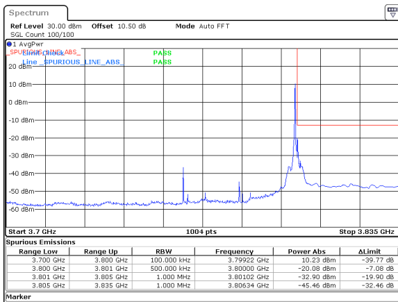
40MHz_15kHz_3780MHz_DFT-s-OFDM QPSK_RB1@215&-20.08 dBm
