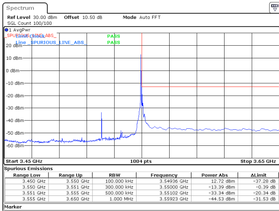
30MHz_15kHz_3535MHz_DFT-s-OFDM QPSK_RB1@159&-13.39 dBm
