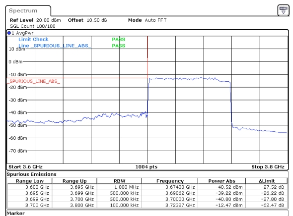
60MHz_30kHz_3730MHz_DFT-s-OFDM QPSK_RB162@0&-39.22 dBm
