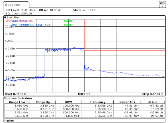
50MHz_15kHz_3525MHz_DFT-s-OFDM QPSK_RB270@0&-29.39 dBm
