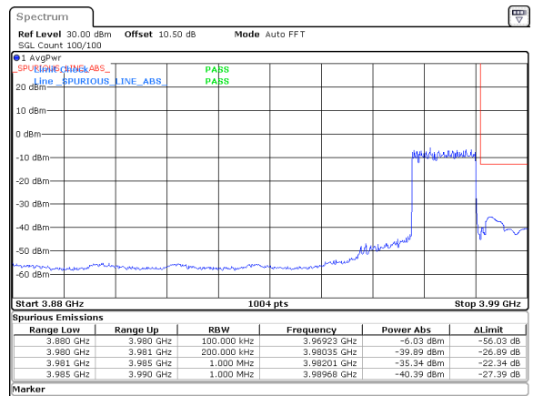
15MHz_15kHz_3972.5MHz_DFT-s-OFDM QPSK_RB75@0&-35.34 dBm
