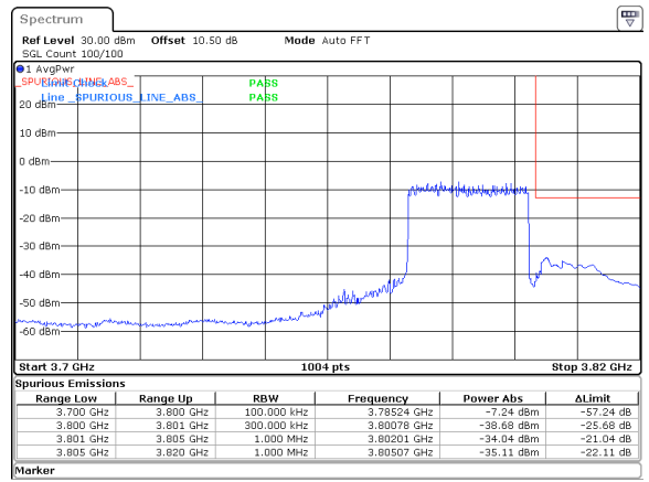
25MHz_15kHz_3787.5MHz_DFT-s-OFDM QPSK_RB128@0&-34.04 dBm
