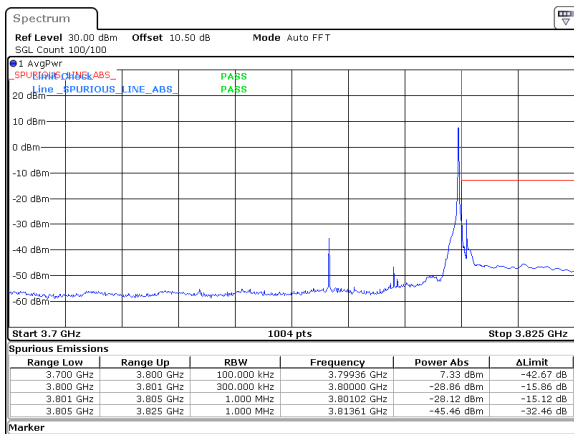
30MHz_15kHz_3785MHz_DFT-s-OFDM QPSK_RB1@159&-28.12 dBm
