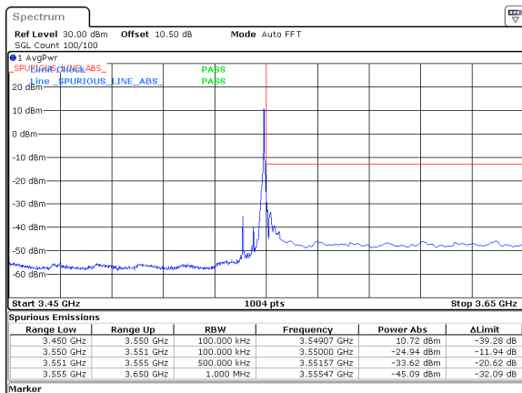
10MHz_30kHz_3545MHz_DFT-s-OFDM QPSK_RB1@23&-24.94 dBm
