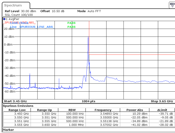
70MHz_30kHz_3515MHz_DFT-s-OFDM QPSK_RB1@188&-22.05 dBm
