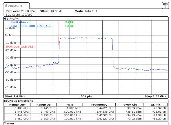
50MHz_15kHz_3475MHz_DFT-s-OFDM QPSK_RB270@0&-34.99 dBm
