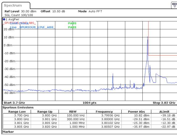
25MHz_15kHz_3787.5MHz_DFT-s-OFDM QPSK_RB1@132&-25.30 dBm
