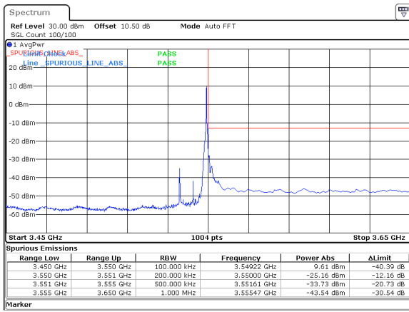
15MHz_30kHz_3542.5MHz_DFT-s-OFDM QPSK_RB1@37&-25.16 dBm
