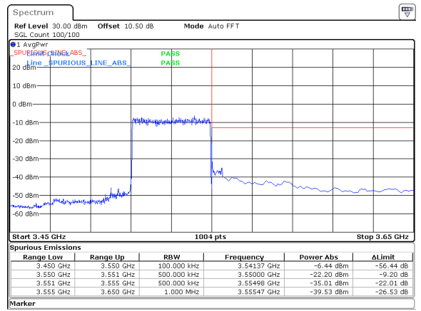
40MHz_15kHz_3530MHz_DFT-s-OFDM QPSK_RB216@0&-22.20 dBm
