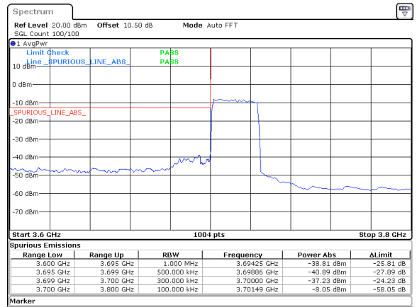
25MHz_30kHz_3712.5MHz_DFT-s-OFDM QPSK_RB64@0&-37.23 dBm
