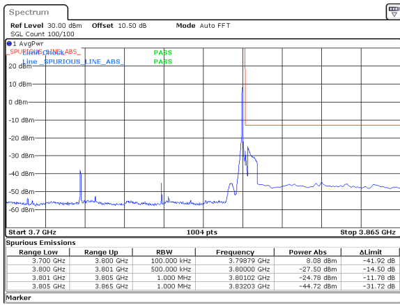
70MHz_30kHz_3765MHz_DFT-s-OFDM QPSK_RB1@188&-24.78 dBm
