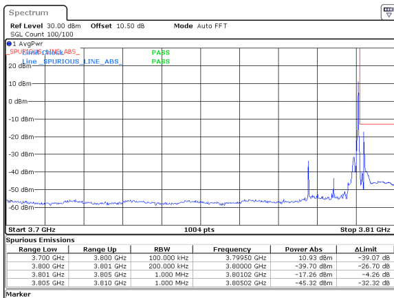
15MHz_15kHz_3792.5MHz_DFT-s-OFDM QPSK_RB1@78&-17.26 dBm
