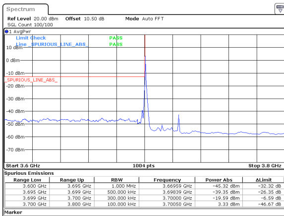
25MHz_15kHz_3712.5MHz_DFT-s-OFDM QPSK_RB1@0&-19.59 dBm
