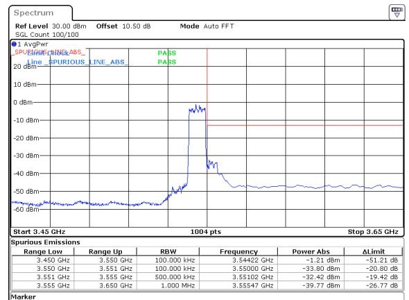
10MHz_30kHz_3545MHz_DFT-s-OFDM QPSK_RB24@0&-32.42 dBm
