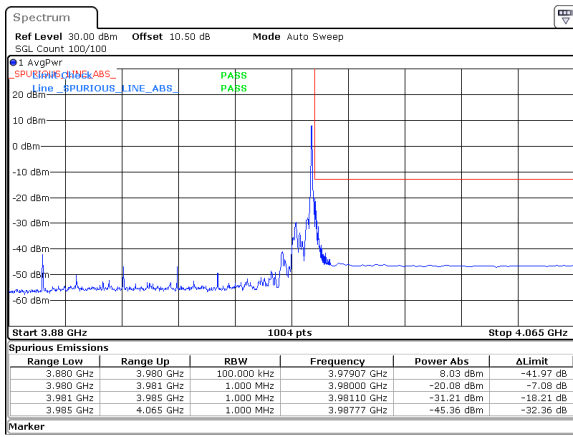
90MHz_30kHz_3935MHz_DFT-s-OFDM QPSK_RB1@244&-20.08 dBm
