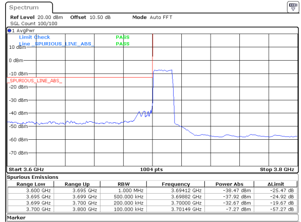
15MHz_15kHz_3707.5MHz_DFT-s-OFDM QPSK_RB75@0&-32.67 dBm
