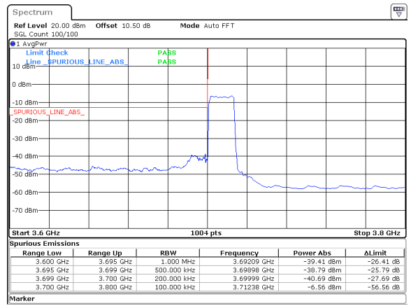
15MHz_30kHz_3707.5MHz_DFT-s-OFDM QPSK_RB36@0&-38.79 dBm
