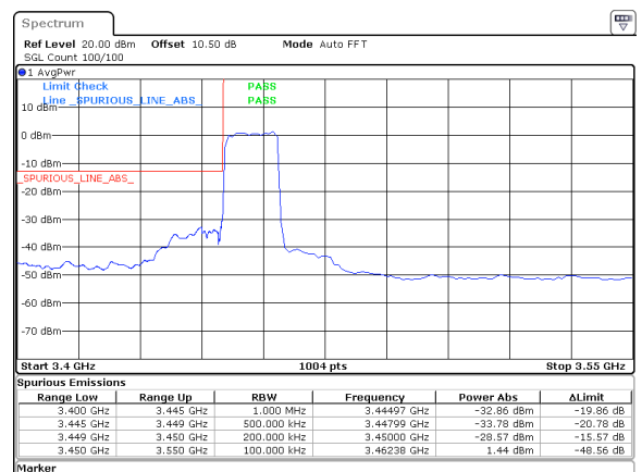
15MHz_30kHz_3457.5MHz_DFT-s-OFDM QPSK_RB36@0&-28.57 dBm
