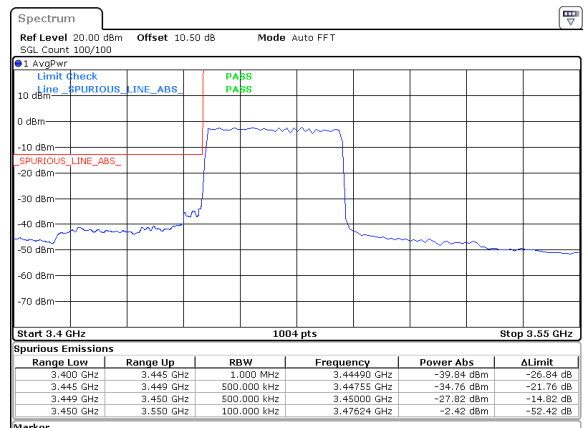
40MHz_30kHz_3470MHz_DFT-s-OFDM QPSK_RB100@0&-27.82 dBm
