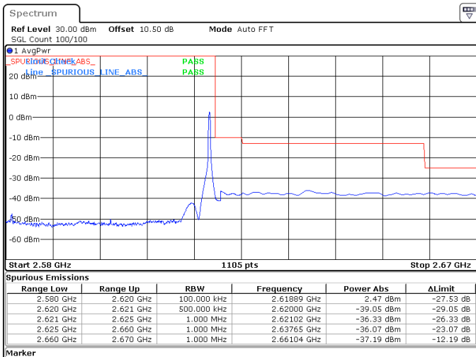
40MHz_30kHz_2600MHz_DFT-s-OFDM QPSK_RB1@105 -37.19 dBm
