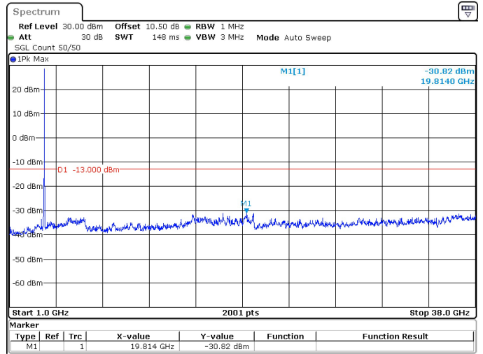
60MHz_30kHz_3750MHz_DFT-s-OFDM QPSK_RB1@161 -30.82 dBm
