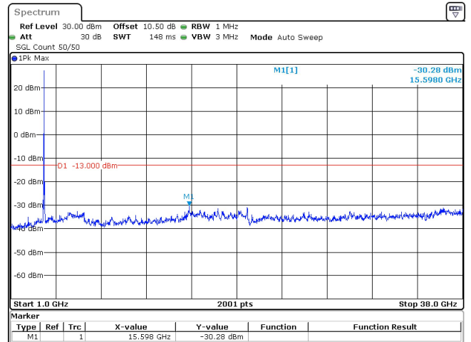
70MHz_30kHz_3735MHz_DFT-s-OFDM QPSK_RB1@0 -30.28 dBm
