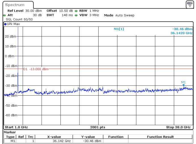
70MHz_30kHz_3735MHz_DFT-s-OFDM QPSK_RB1@188 -30.46 dBm
