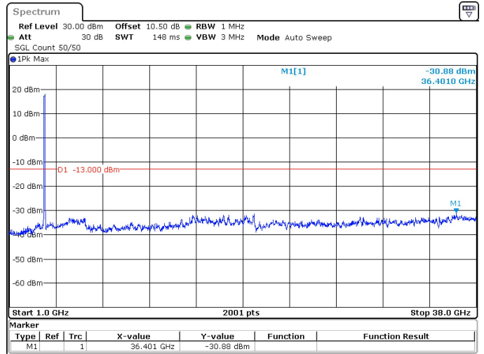
50MHz_30kHz_3775MHz_DFT-s-OFDM QPSK_RB128@0 -30.88 dBm
