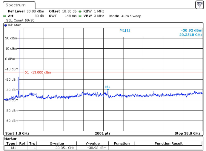
50MHz_30kHz_3775MHz_DFT-s-OFDM QPSK_RB1@132 -30.92 dBm
