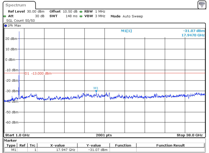
50MHz_30kHz_3750MHz_DFT-s-OFDM QPSK_RB1@132 -31.07 dBm
