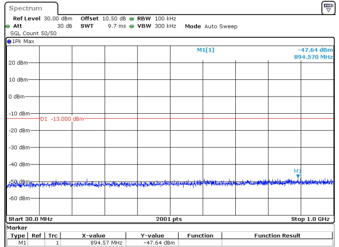
50MHz_15kHz_3775MHz_DFT-s-OFDM QPSK_RB270@0 -47.64 dBm
