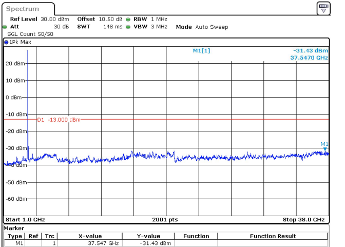
50MHz_30kHz_3750MHz_DFT-s-OFDM QPSK_RB1@0 -31.43 dBm
