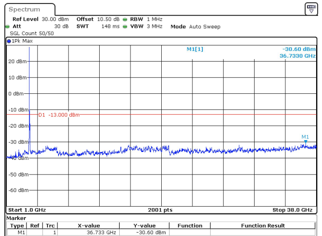
50MHz_15kHz_3775MHz_DFT-s-OFDM QPSK_RB1@0 -30.60 dBm
