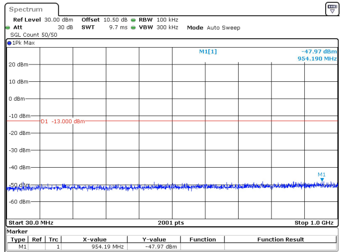
50MHz_15kHz_3750MHz_DFT-s-OFDM QPSK_RB1@269 -47.97 dBm
