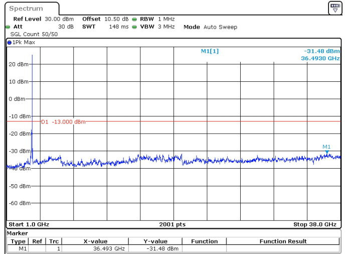
50MHz_15kHz_3775MHz_DFT-s-OFDM QPSK_RB1@269 -31.48 dBm
