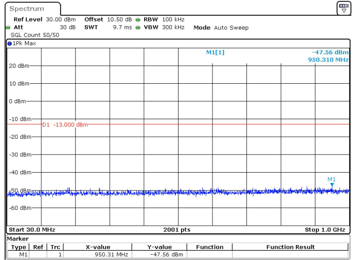
50MHz_30kHz_3725MHz_DFT-s-OFDM QPSK_RB1@132 -47.56 dBm
