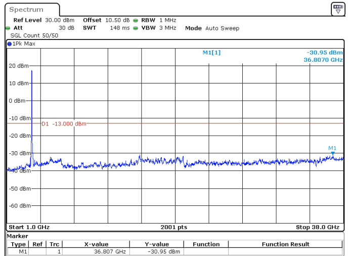
50MHz_15kHz_3750MHz_DFT-s-OFDM QPSK_RB270@0 -30.95 dBm
