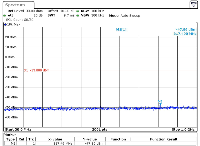
50MHz_30kHz_3725MHz_DFT-s-OFDM QPSK_RB128@0 -47.86 dBm
