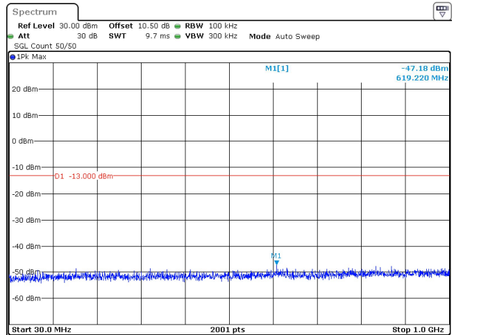
30MHz_15kHz_3715MHz_DFT-s-OFDM QPSK_RB1@0 -47.18 dBm
