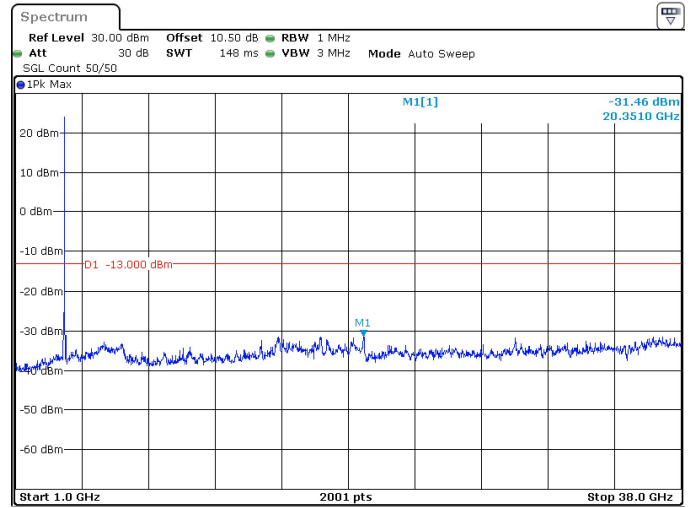
30MHz_15kHz_3715MHz_DFT-s-OFDM QPSK_RB1@159 -31.46 dBm
