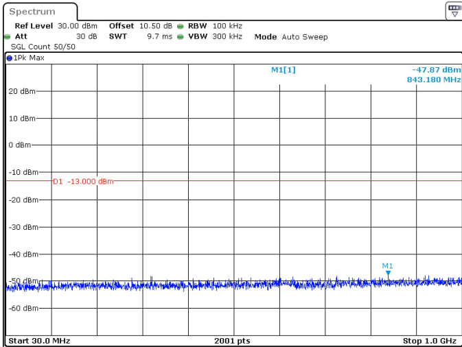
30MHz_15kHz_3715MHz_DFT-s-OFDM QPSK_RB160@0 -47.87 dBm
