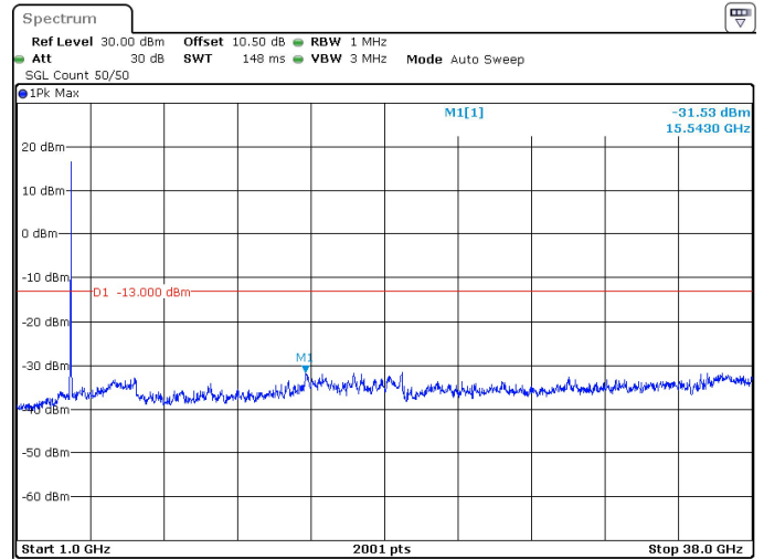
30MHz_15kHz_3715MHz_DFT-s-OFDM QPSK_RB160@0 -31.53 dBm
