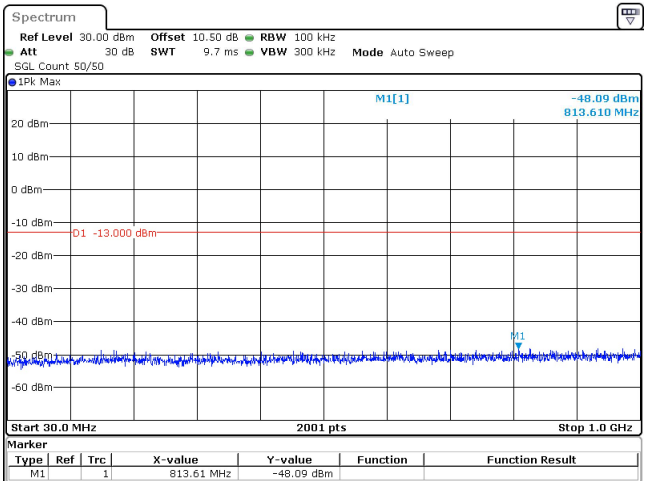
25MHz_30kHz_3787.5MHz_DFT-s-OFDM QPSK_RB1@0 -48.09 dBm
