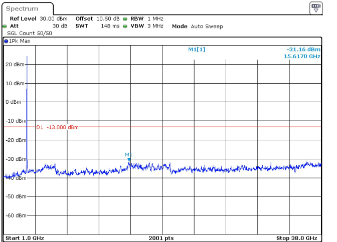
30MHz_15kHz_3715MHz_DFT-s-OFDM QPSK_RB1@0 -31.16 dBm
