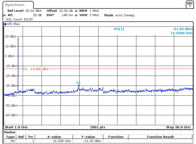
25MHz_30kHz_3787.5MHz_DFT-s-OFDM QPSK_RB64@0 -31.03 dBm
