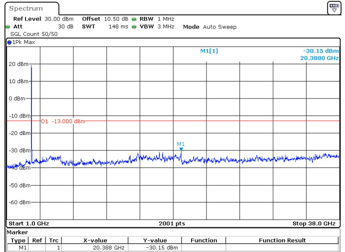
25MHz_30kHz_3750MHz_DFT-s-OFDM QPSK_RB64@0 -30.15 dBm
