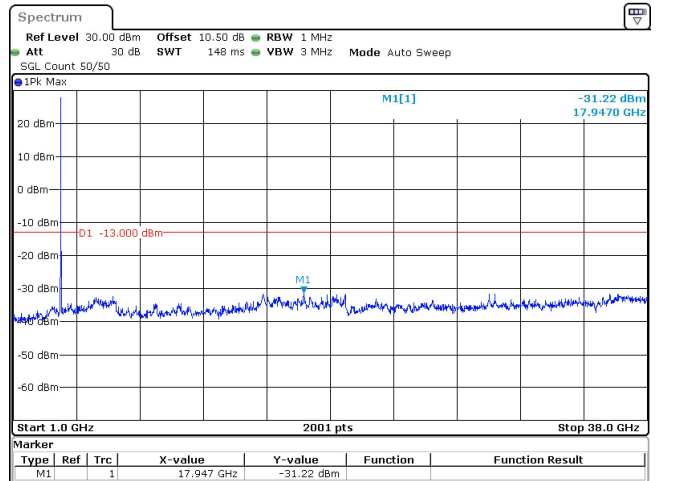
25MHz_30kHz_3787.5MHz_DFT-s-OFDM QPSK_RB1@0 -31.22 dBm
