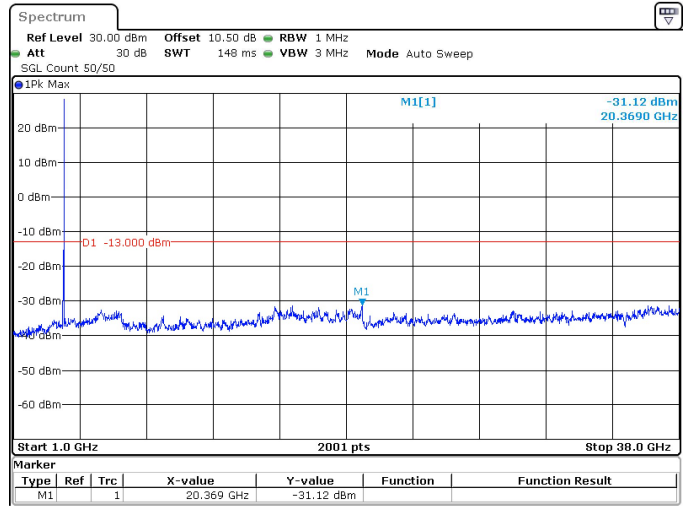
25MHz_30kHz_3787.5MHz_DFT-s-OFDM QPSK_RB1@64 -31.12 dBm
