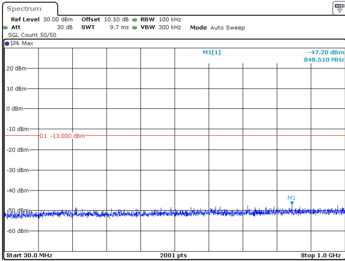
30MHz_15kHz_3715MHz_DFT-s-OFDM QPSK_RB1@159 -47.20 dBm
