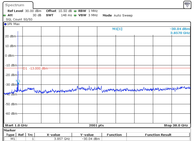
25MHz_15kHz_3787.5MHz_DFT-s-OFDM QPSK_RB1@0 -30.04 dBm
