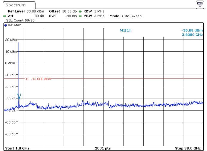
25MHz_15kHz_3750MHz_DFT-s-OFDM QPSK_RB128@0 -30.09 dBm
