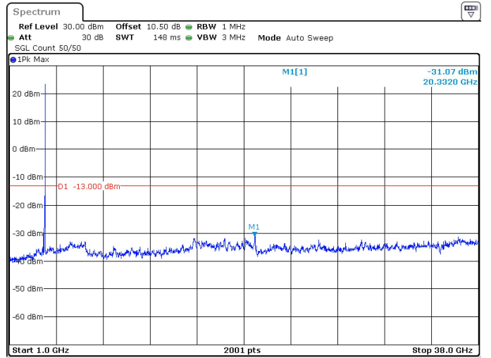
25MHz_15kHz_3787.5MHz_DFT-s-OFDM QPSK_RB1@132 -31.07 dBm
