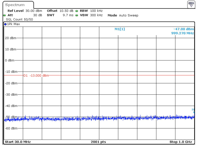
25MHz_15kHz_3750MHz_DFT-s-OFDM QPSK_RB1@132 -47.00 dBm
