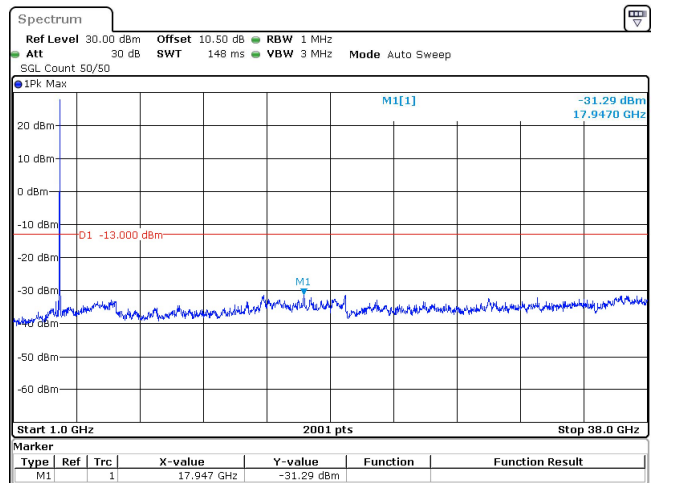
25MHz_30kHz_3712.5MHz_DFT-s-OFDM QPSK_RB1@0 -31.29 dBm
