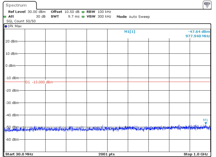
25MHz_15kHz_3787.5MHz_DFT-s-OFDM QPSK_RB128@0 -47.64 dBm
