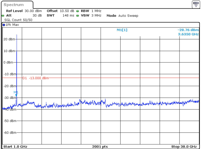
25MHz_15kHz_3712.5MHz_DFT-s-OFDM QPSK_RB1@0 -28.76 dBm
