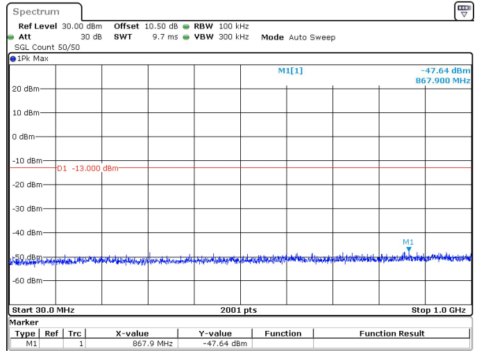
15MHz_30kHz_3792.5MHz_DFT-s-OFDM QPSK_RB36@0 -47.64 dBm
