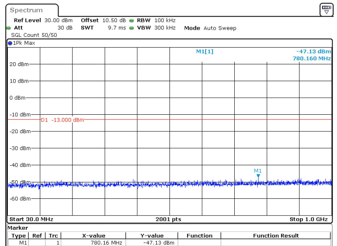
15MHz_30kHz_3750MHz_DFT-s-OFDM QPSK_RB36@0 -47.13 dBm
