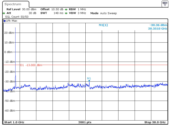
25MHz_15kHz_3712.5MHz_DFT-s-OFDM QPSK_RB1@132 -30.36 dBm
