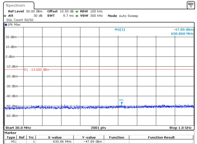
15MHz_30kHz_3750MHz_DFT-s-OFDM QPSK_RB1@37 -47.89 dBm
