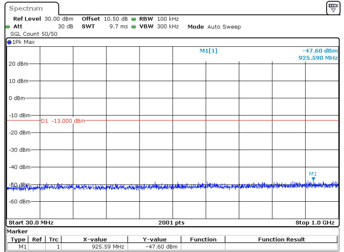
15MHz_30kHz_3792.5MHz_DFT-s-OFDM QPSK_RB1@37 -47.60 dBm
