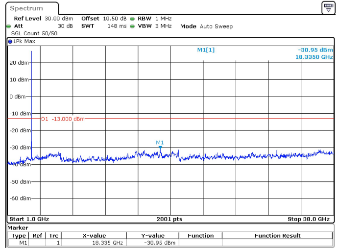
15MHz_30kHz_3707.5MHz_DFT-s-OFDM QPSK_RB1@37 -30.95 dBm
