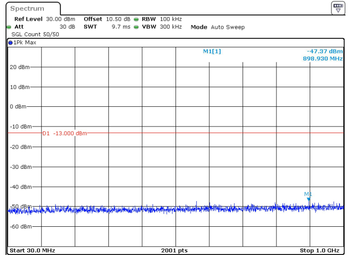
15MHz_15kHz_3750MHz_DFT-s-OFDM QPSK_RB75@0 -47.37 dBm
