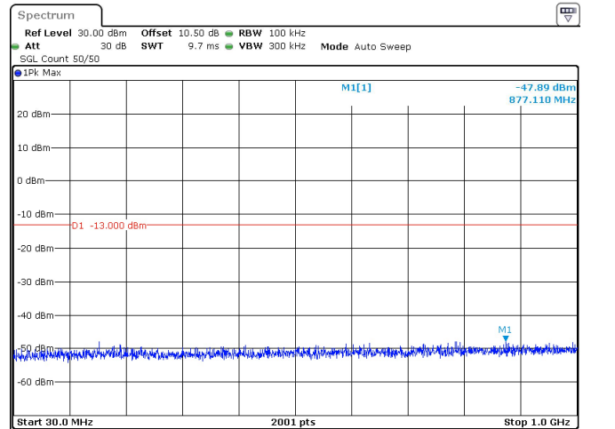
15MHz_15kHz_3792.5MHz_DFT-s-OFDM QPSK_RB1@0 -47.89 dBm
