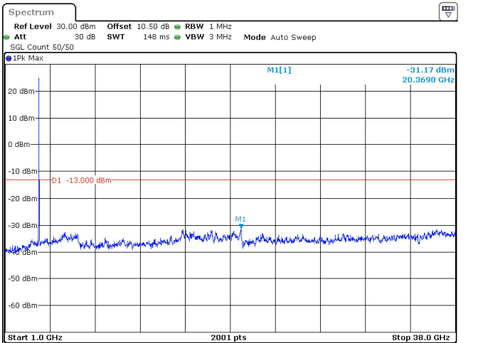
15MHz_15kHz_3792.5MHz_DFT-s-OFDM QPSK_RB1@0 -31.17 dBm
