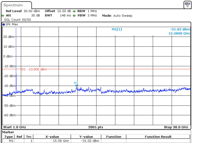
15MHz_30kHz_3750MHz_DFT-s-OFDM QPSK_RB1@0 -31.02 dBm
