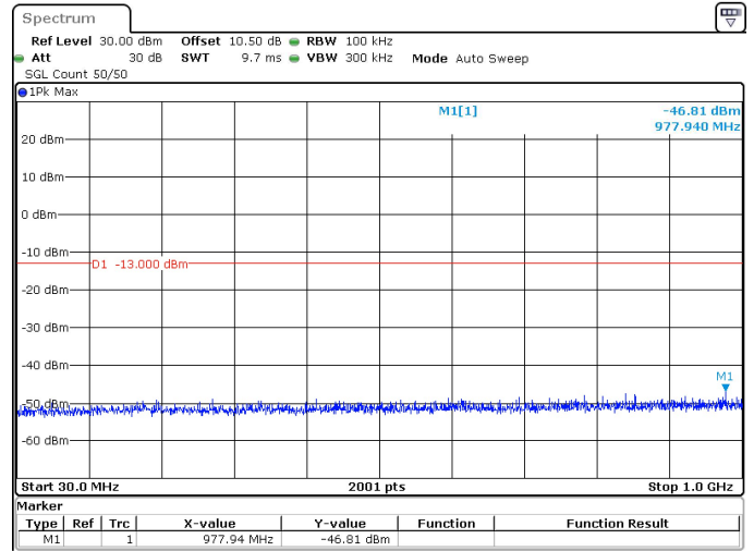
15MHz_30kHz_3707.5MHz_DFT-s-OFDM QPSK_RB36@0 -46.81 dBm
