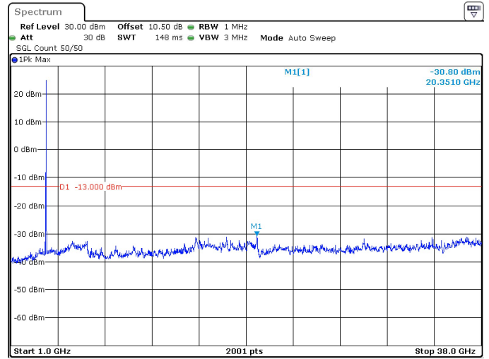
15MHz_15kHz_3750MHz_DFT-s-OFDM QPSK_RB1@78 -30.80 dBm
