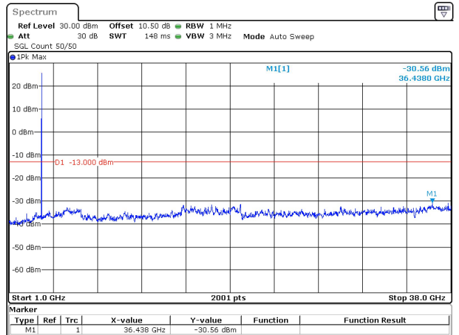
15MHz_30kHz_3707.5MHz_DFT-s-OFDM QPSK_RB1@0 -30.56 dBm
