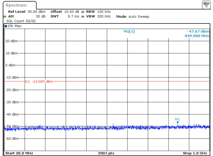
15MHz_15kHz_3792.5MHz_DFT-s-OFDM QPSK_RB75@0 -47.67 dBm
