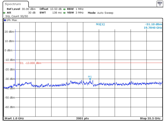
60MHz_30kHz_3520MHz_DFT-s-OFDM QPSK_RB1@161 -31.10 dBm
