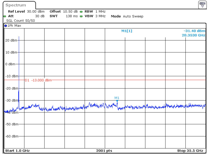
70MHz_30kHz_3500MHz_DFT-s-OFDM QPSK_RB1@188 -31.40 dBm
