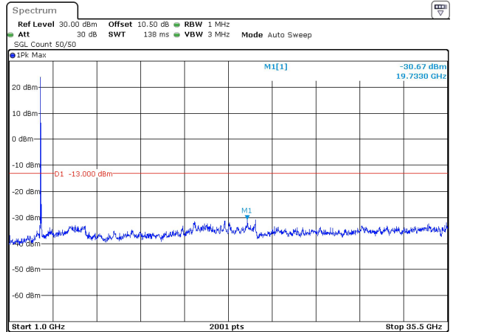
70MHz_30kHz_3515MHz_DFT-s-OFDM QPSK_RB1@0 -30.67 dBm
