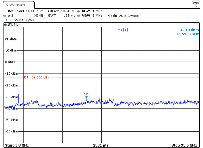
50MHz_30kHz_3525MHz_DFT-s-OFDM QPSK_RB128@0 -31.18 dBm
