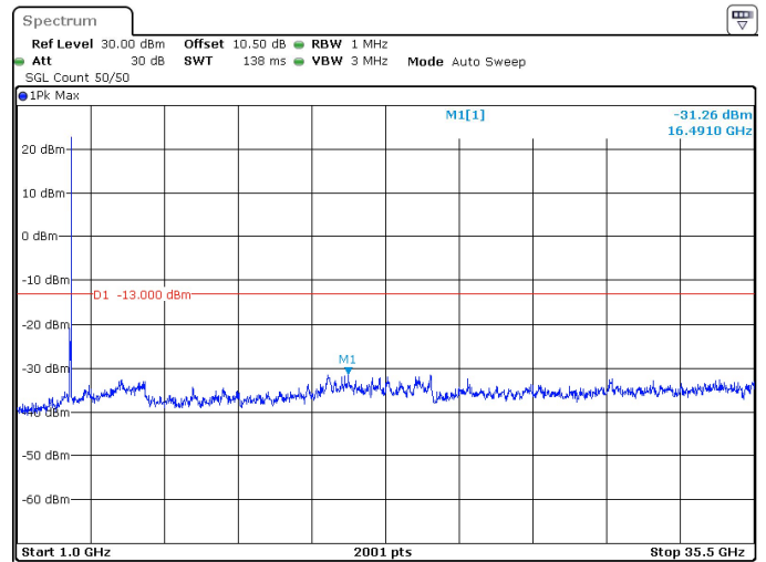
60MHz_30kHz_3500MHz_DFT-s-OFDM QPSK_RB1@161 -31.26 dBm
