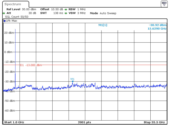
50MHz_30kHz_3525MHz_DFT-s-OFDM QPSK_RB1@132 -30.92 dBm
