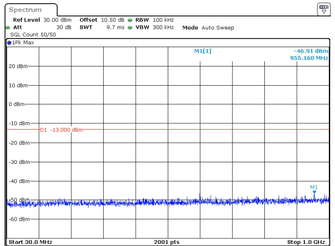
50MHz_30kHz_3525MHz_DFT-s-OFDM QPSK_RB1@0 -46.91 dBm
