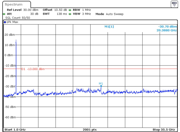
50MHz_30kHz_3500MHz_DFT-s-OFDM QPSK_RB128@0 -30.70 dBm
