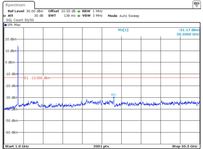
50MHz_30kHz_3475MHz_DFT-s-OFDM QPSK_RB128@0 -31.17 dBm
