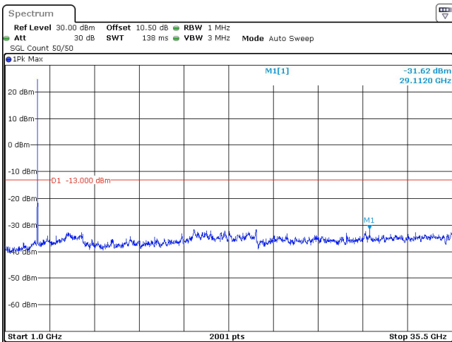
50MHz_30kHz_3525MHz_DFT-s-OFDM QPSK_RB1@0 -31.62 dBm
