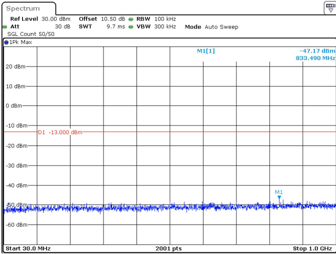
40MHz_30kHz_3530MHz_DFT-s-OFDM QPSK_RB1@105 -47.17 dBm
