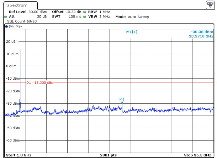
40MHz_30kHz_3530MHz_DFT-s-OFDM QPSK_RB100@0 -30.38 dBm
