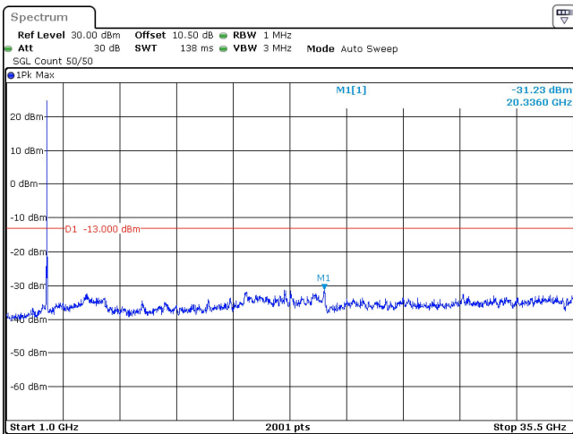
50MHz_30kHz_3475MHz_DFT-s-OFDM QPSK_RB1@0 -31.23 dBm
