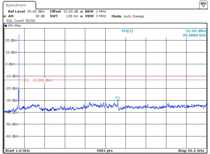
50MHz_30kHz_3500MHz_DFT-s-OFDM QPSK_RB1@132 -31.05 dBm
