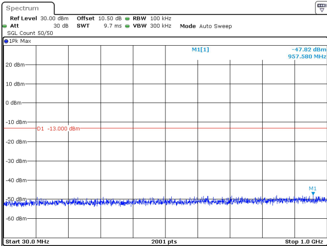
50MHz_30kHz_3475MHz_DFT-s-OFDM QPSK_RB128@0 -47.82 dBm
