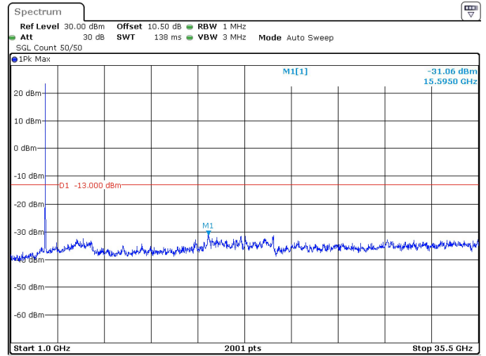
40MHz_30kHz_3530MHz_DFT-s-OFDM QPSK_RB1@105 -31.06 dBm
