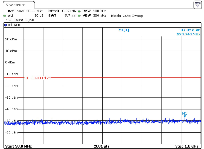
50MHz_30kHz_3475MHz_DFT-s-OFDM QPSK_RB1@132 -47.32 dBm
