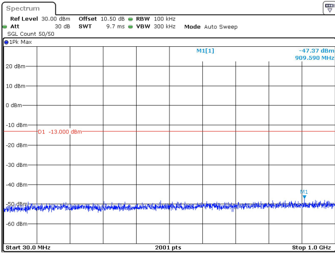
50MHz_30kHz_3500MHz_DFT-s-OFDM QPSK_RB1@132 -47.37 dBm
