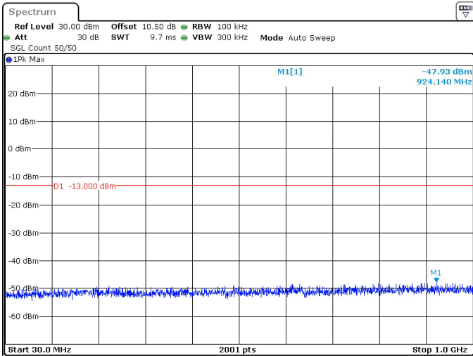
50MHz_30kHz_3500MHz_DFT-s-OFDM QPSK_RB128@0 -47.93 dBm
