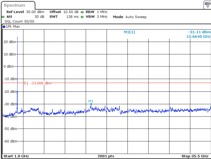
50MHz_30kHz_3475MHz_DFT-s-OFDM QPSK_RB1@132 -31.11 dBm
