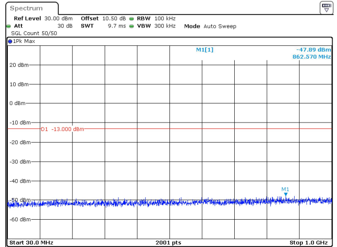
40MHz_30kHz_3500MHz_DFT-s-OFDM QPSK_RB100@0 -47.89 dBm
