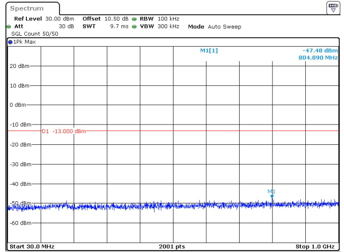
40MHz_30kHz_3500MHz_DFT-s-OFDM QPSK_RB1@105 -47.48 dBm
