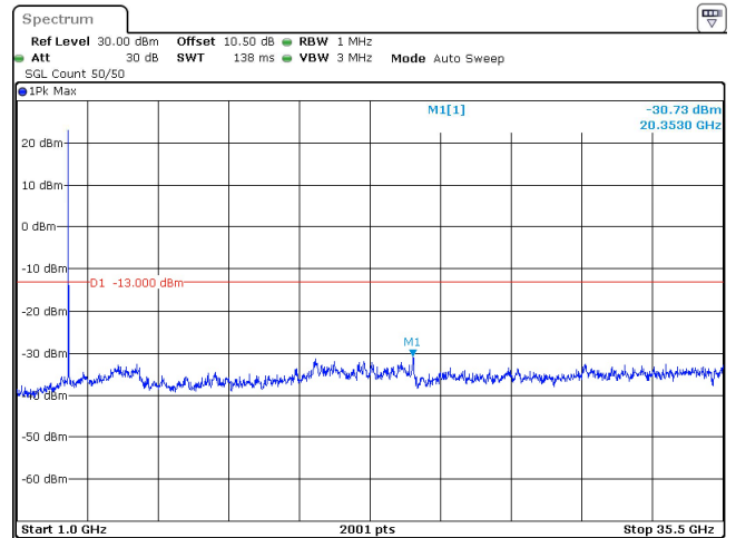
40MHz_30kHz_3530MHz_DFT-s-OFDM QPSK_RB1@0 -30.73 dBm
