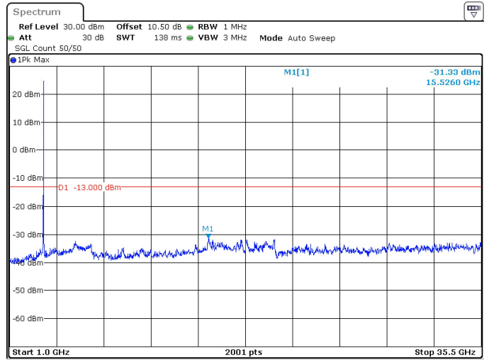
40MHz_30kHz_3470MHz_DFT-s-OFDM QPSK_RB1@105 -31.33 dBm
