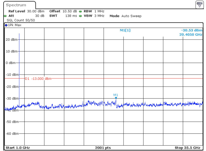
15MHz_30kHz_3542.5MHz_DFT-s-OFDM QPSK_RB1@37 -30.53 dBm
