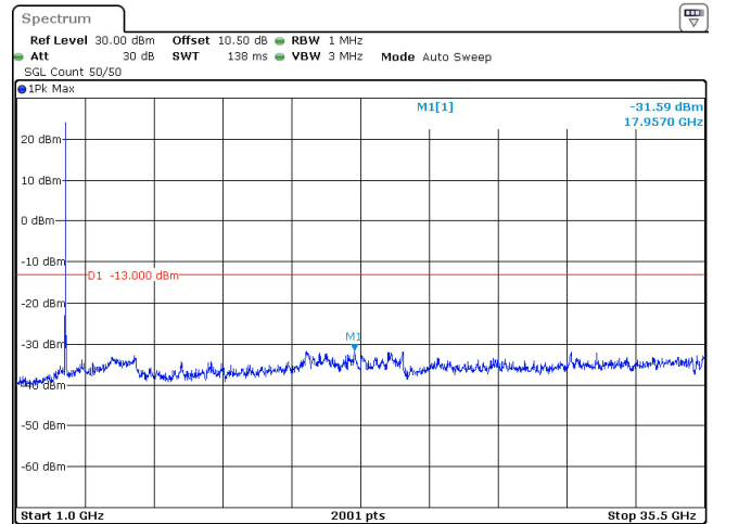
25MHz_30kHz_3462.5MHz_DFT-s-OFDM QPSK_RB1@0 -31.59 dBm
