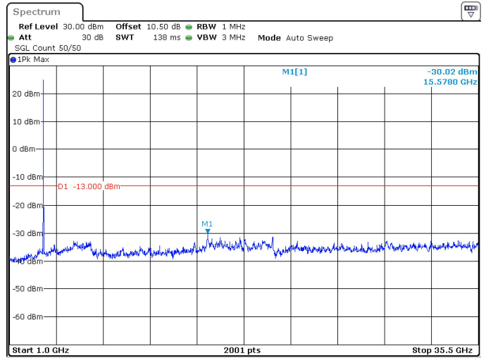
25MHz_30kHz_3500MHz_DFT-s-OFDM QPSK_RB1@64 -30.02 dBm
