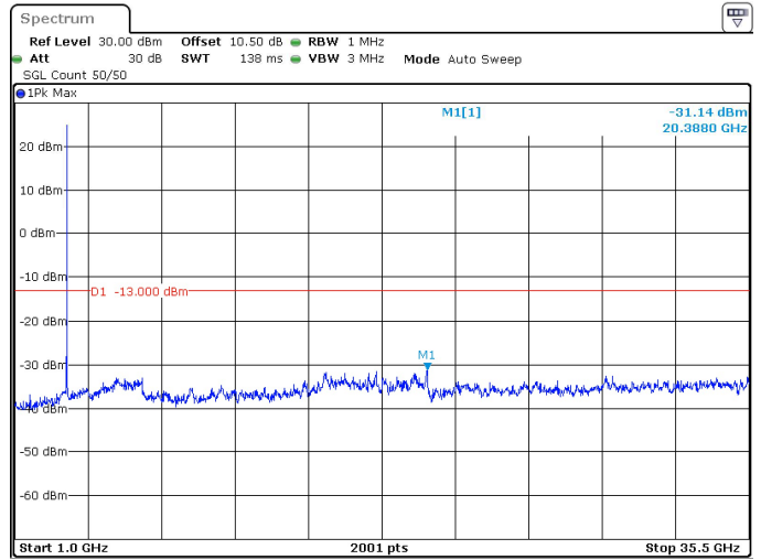
25MHz_30kHz_3462.5MHz_DFT-s-OFDM QPSK_RB1@64 -31.14 dBm
