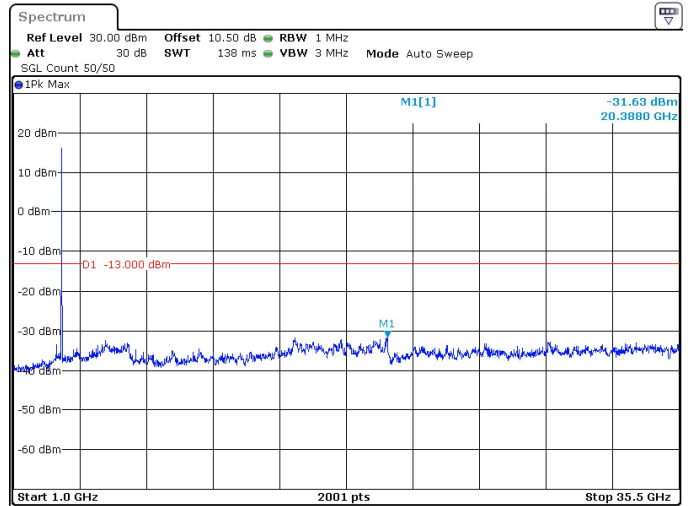
25MHz_30kHz_3500MHz_DFT-s-OFDM QPSK_RB64@0 -31.63 dBm
