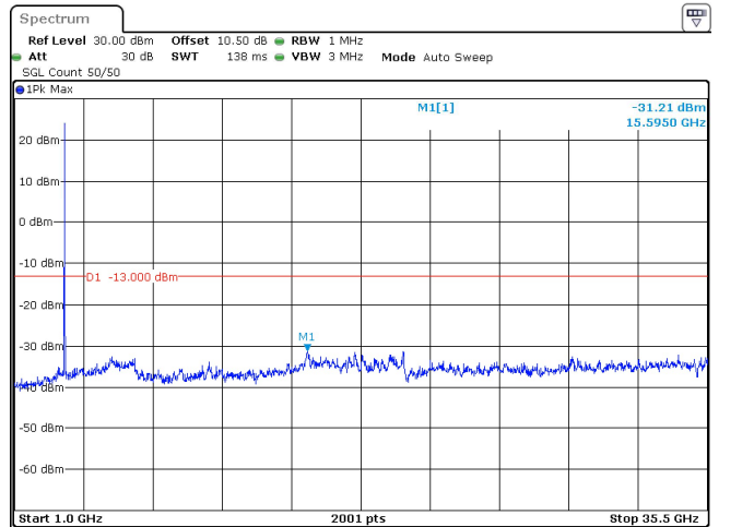
25MHz_30kHz_3500MHz_DFT-s-OFDM QPSK_RB1@0 -31.21 dBm
