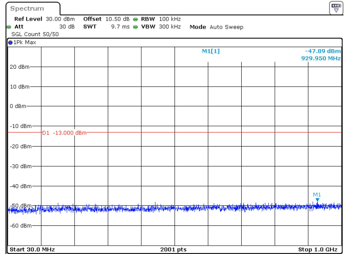
15MHz_30kHz_3542.5MHz_DFT-s-OFDM QPSK_RB36@0 -47.89 dBm
