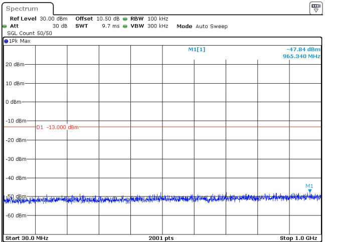
25MHz_30kHz_3462.5MHz_DFT-s-OFDM QPSK_RB1@0 -47.84 dBm
