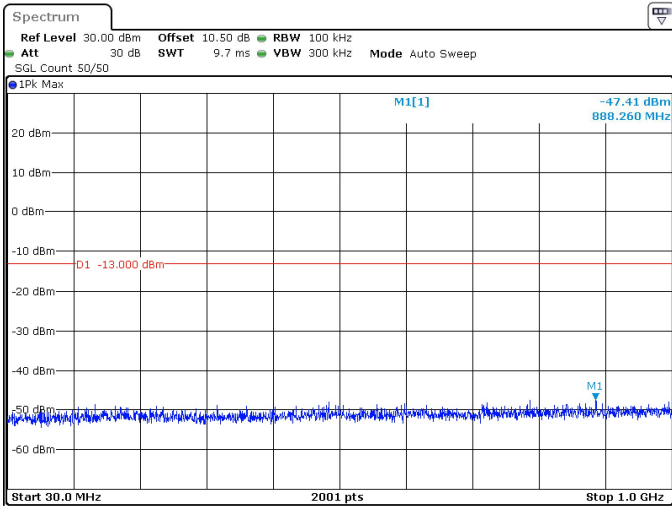
25MHz_30kHz_3462.5MHz_DFT-s-OFDM QPSK_RB64@0 -47.41 dBm
