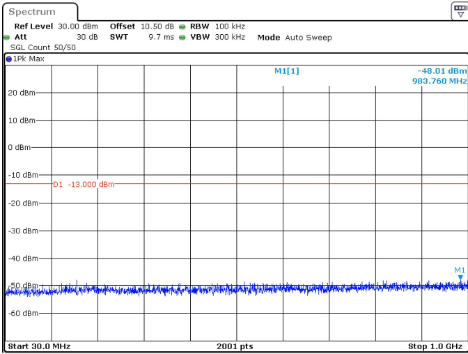
15MHz_30kHz_3542.5MHz_DFT-s-OFDM QPSK_RB1@37 -48.01 dBm
