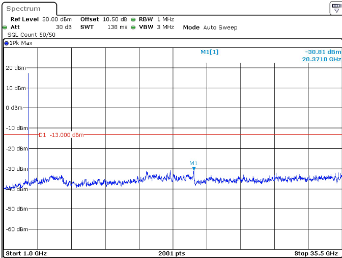
15MHz_30kHz_3542.5MHz_DFT-s-OFDM QPSK_RB36@0 -30.81 dBm
