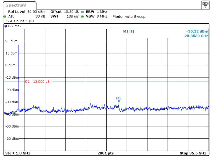
25MHz_30kHz_3462.5MHz_DFT-s-OFDM QPSK_RB64@0 -30.32 dBm
