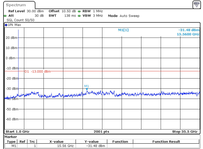
15MHz_30kHz_3457.5MHz_DFT-s-OFDM QPSK_RB1@37 -31.48 dBm
