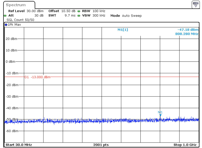
15MHz_30kHz_3500MHz_DFT-s-OFDM QPSK_RB1@37 -47.18 dBm
