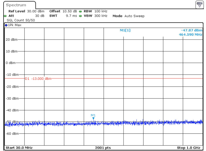
15MHz_30kHz_3457.5MHz_DFT-s-OFDM QPSK_RB1@0 -47.87 dBm
