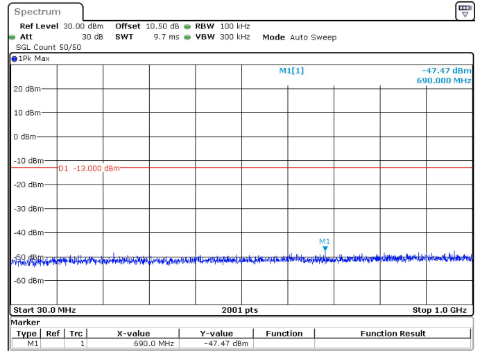
15MHz_30kHz_3457.5MHz_DFT-s-OFDM QPSK_RB1@0 -47.47 dBm
