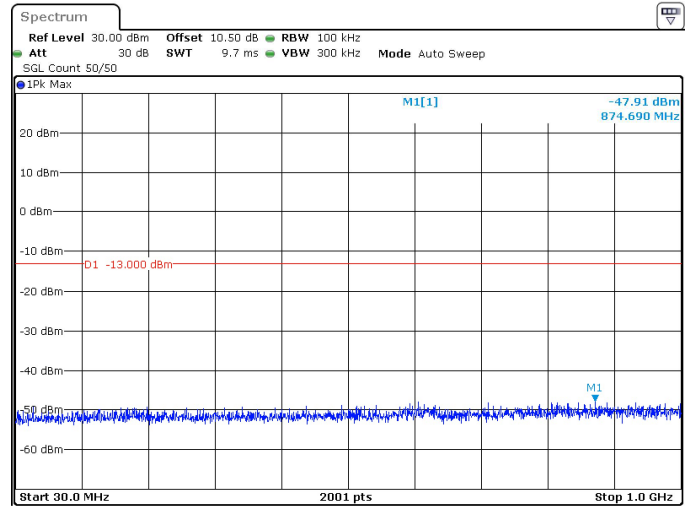
15MHz_30kHz_3457.5MHz_DFT-s-OFDM QPSK_RB36@0 -47.91 dBm
