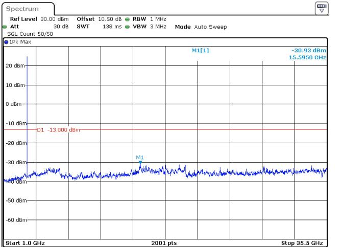
15MHz_30kHz_3500MHz_DFT-s-OFDM QPSK_RB1@0 -30.93 dBm
