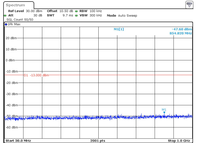
15MHz_30kHz_3457.5MHz_DFT-s-OFDM QPSK_RB1@37 -47.60 dBm
