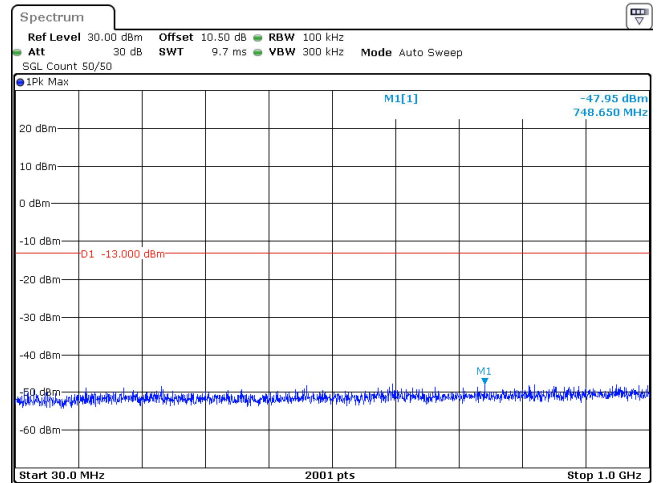
15MHz_30kHz_3542.5MHz_DFT-s-OFDM QPSK_RB1@0 -47.95 dBm
