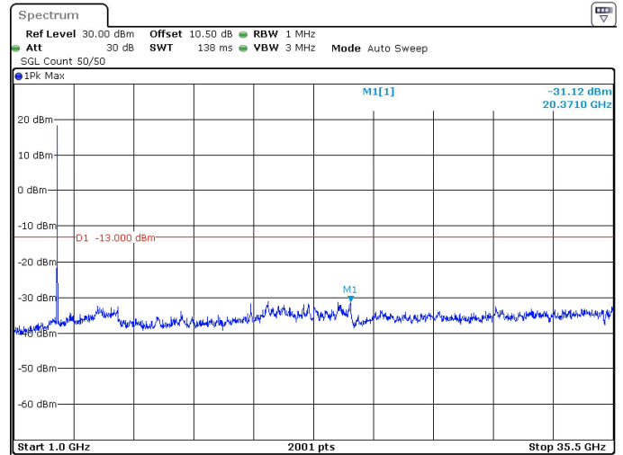
15MHz_30kHz_3500MHz_DFT-s-OFDM QPSK_RB36@0 -31.12 dBm
