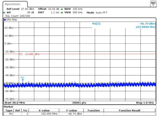
60MHz_30kHz_3840MHz_DFT-s-OFDM QPSK_RB162@0 -46.74 dBm
