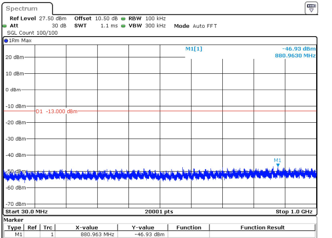
60MHz_30kHz_3730MHz_DFT-s-OFDM QPSK_RB1@161 -46.93 dBm
