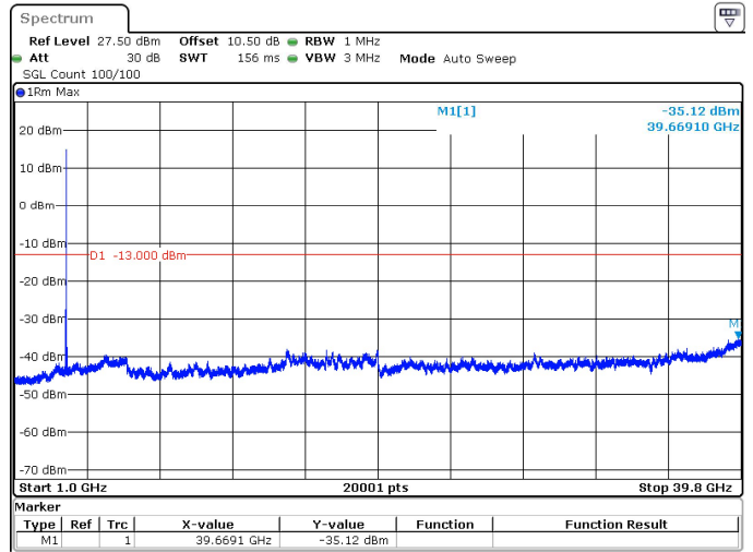
60MHz_30kHz_3730MHz_DFT-s-OFDM QPSK_RB1@161 -35.12 dBm
