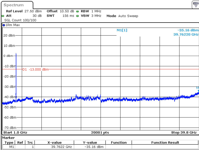
60MHz_30kHz_3730MHz_DFT-s-OFDM QPSK_RB162@0 -35.16 dBm
