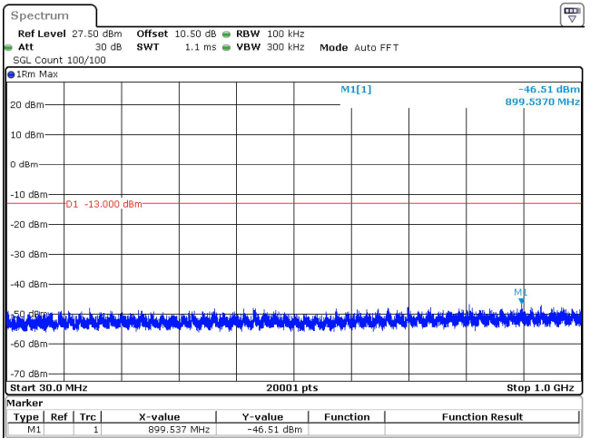
60MHz_30kHz_3840MHz_DFT-s-OFDM QPSK_RB1@161 -46.51 dBm
