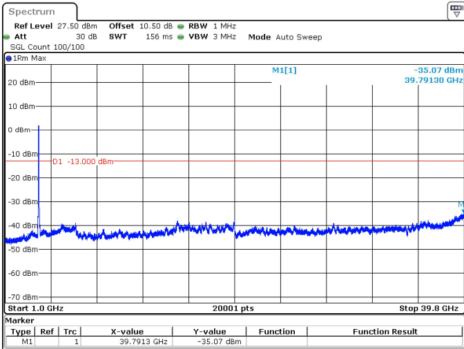
60MHz_30kHz_3840MHz_DFT-s-OFDM QPSK_RB162@0 -35.07 dBm
