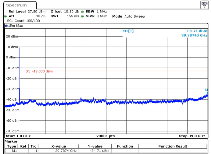
60MHz_30kHz_3840MHz_DFT-s-OFDM QPSK_RB1@161 -34.71 dBm
