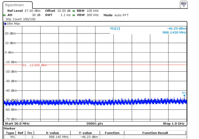
60MHz_30kHz_3730MHz_DFT-s-OFDM QPSK_RB162@0 -46.23 dBm
