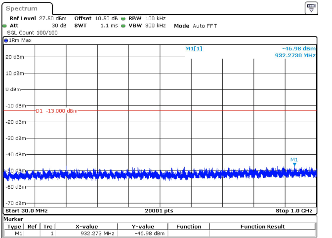
50MHz_15kHz_3840MHz_DFT-s-OFDM QPSK_RB1@269 -46.98 dBm
