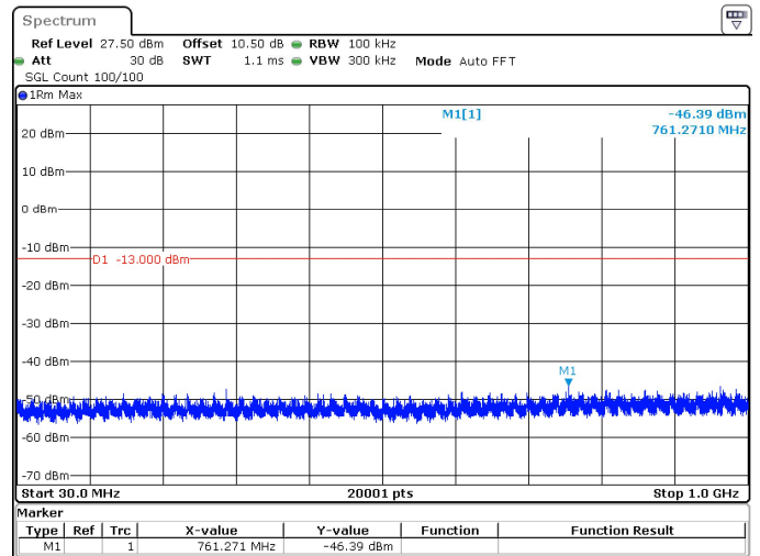
50MHz_15kHz_3725MHz_DFT-s-OFDM QPSK_RB1@0 -46.39 dBm
