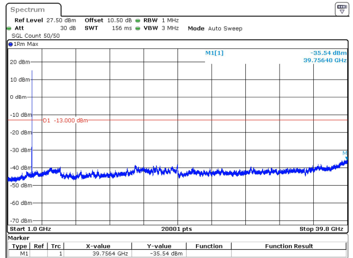
50MHz_15kHz_3725MHz_DFT-s-OFDM QPSK_RB1@269 -35.54 dBm
