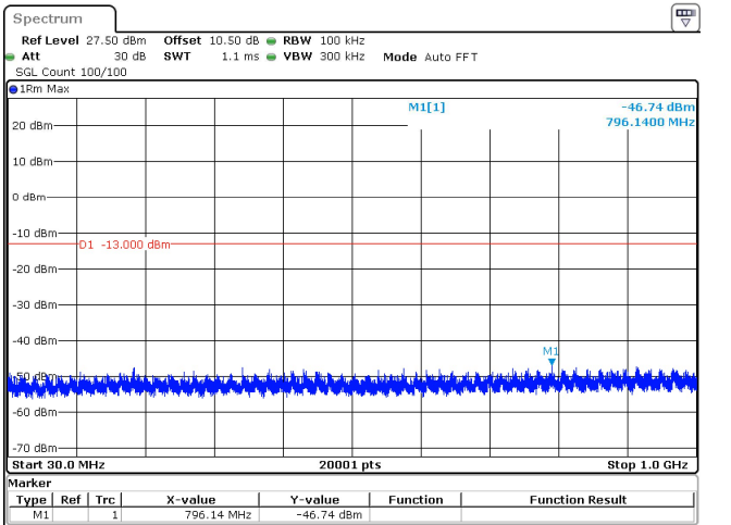
50MHz_15kHz_3955MHz_DFT-s-OFDM QPSK_RB1@269 -46.74 dBm
