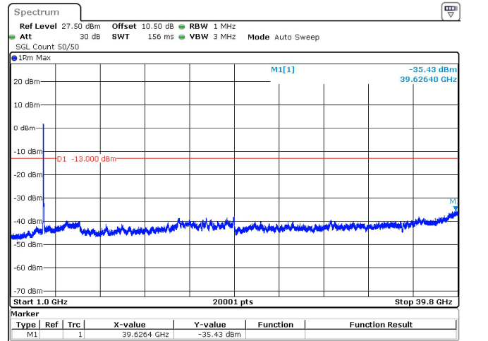
50MHz_15kHz_3840MHz_DFT-s-OFDM QPSK_RB270@0 -35.43 dBm
