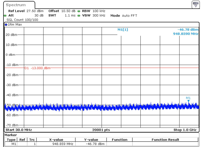
40MHz_15kHz_3840MHz_DFT-s-OFDM QPSK_RB1@215 -46.78 dBm
