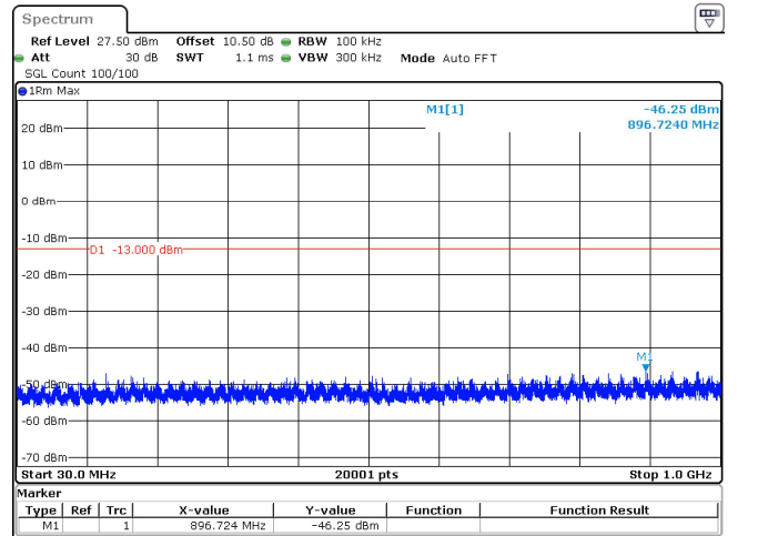
40MHz_15kHz_3840MHz_DFT-s-OFDM QPSK_RB216@0 -46.25 dBm
