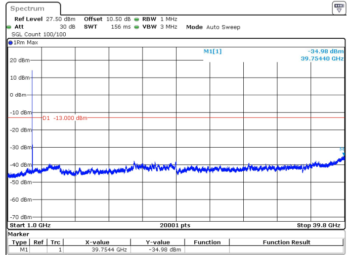
40MHz_15kHz_3840MHz_DFT-s-OFDM QPSK_RB1@0 -34.98 dBm
