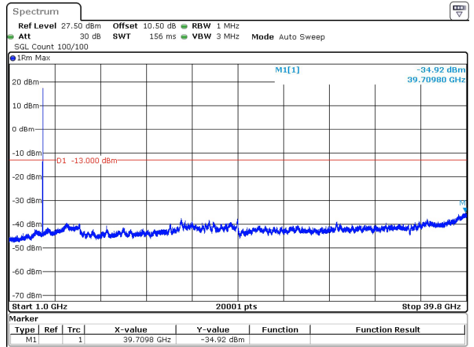
30MHz_15kHz_3840MHz_DFT-s-OFDM QPSK_RB1@0 -34.92 dBm
