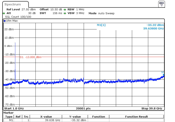
30MHz_15kHz_3840MHz_DFT-s-OFDM QPSK_RB160@0 -35.32 dBm
