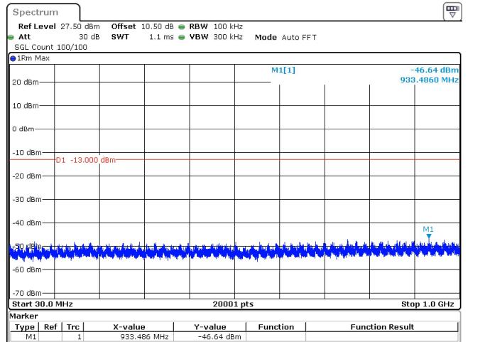
30MHz_15kHz_3715MHz_DFT-s-OFDM QPSK_RB160@0 -46.64 dBm
