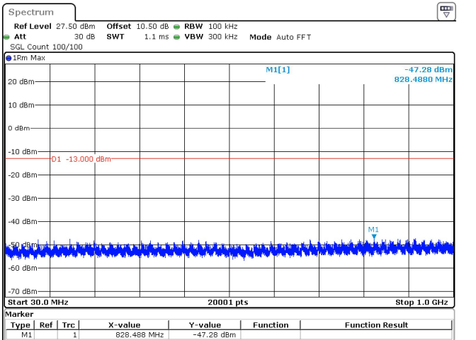
30MHz_15kHz_3715MHz_DFT-s-OFDM QPSK_RB1@159 -47.28 dBm
