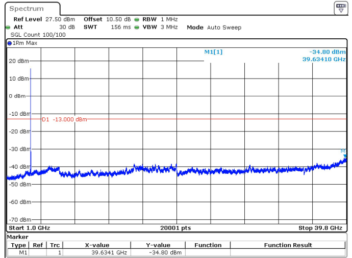
30MHz_15kHz_3715MHz_DFT-s-OFDM QPSK_RB1@0 -34.80 dBm
