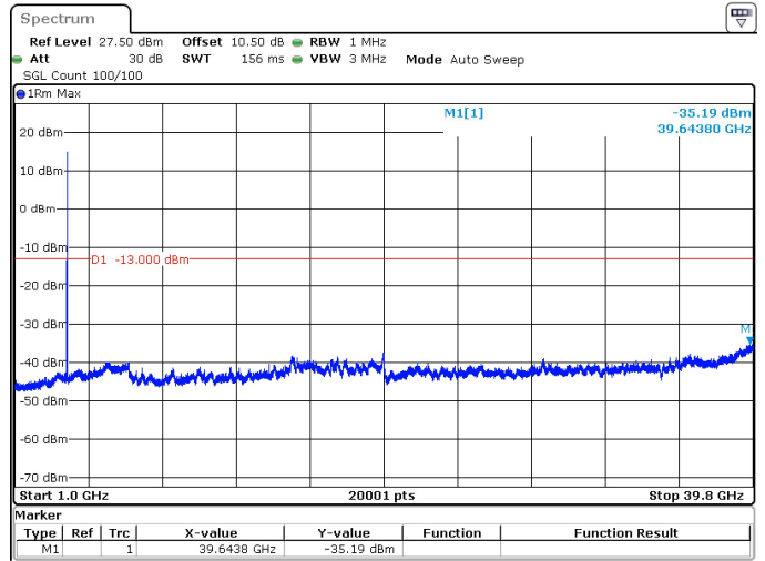
30MHz_15kHz_3715MHz_DFT-s-OFDM QPSK_RB1@159 -35.19 dBm
