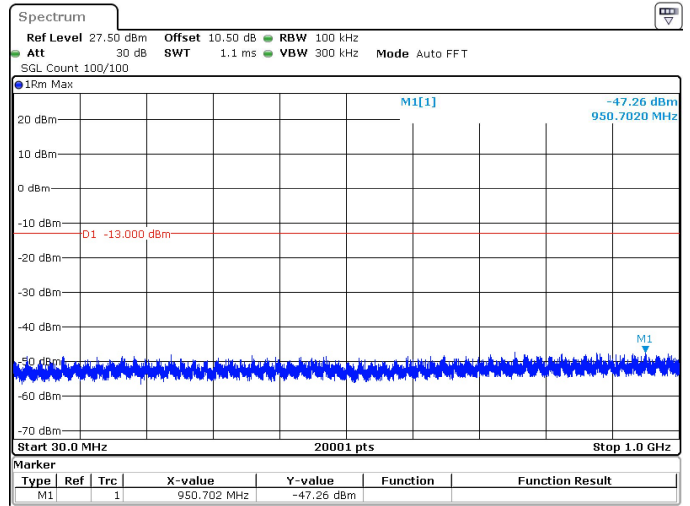
30MHz_15kHz_3840MHz_DFT-s-OFDM QPSK_RB1@159 -47.26 dBm
