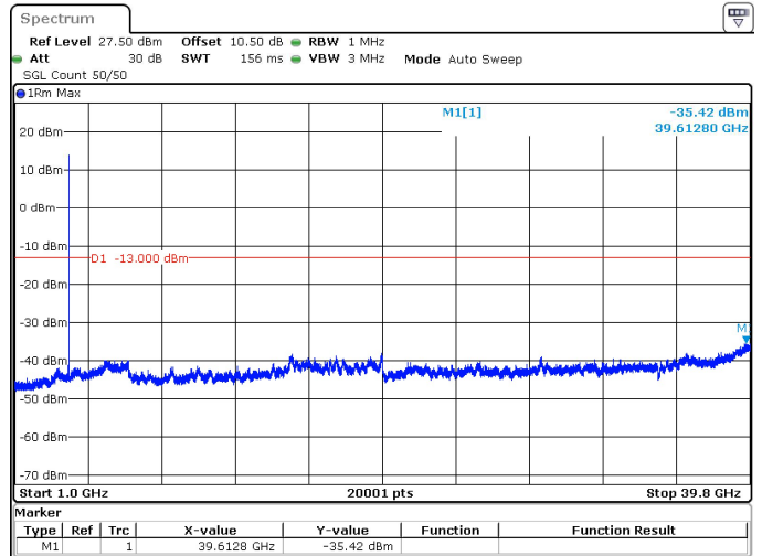
20MHz_30kHz_3840MHz_DFT-s-OFDM QPSK_RB1@50 -35.42 dBm
