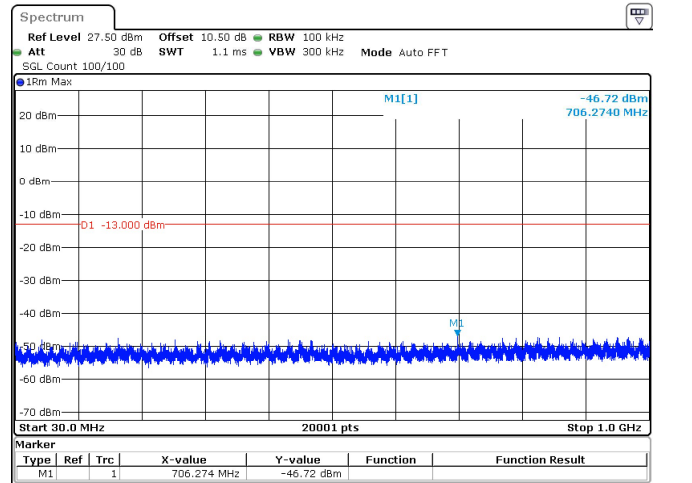
20MHz_15kHz_3840MHz_DFT-s-OFDM QPSK_RB100@0 -46.72 dBm
