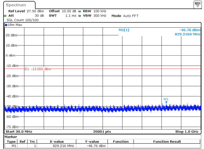
20MHz_15kHz_3840MHz_DFT-s-OFDM QPSK_RB1@0 -46.76 dBm
