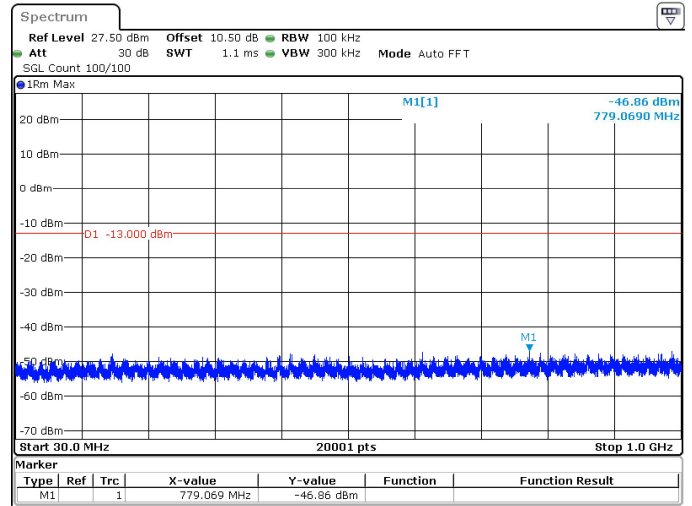
20MHz_15kHz_3840MHz_DFT-s-OFDM QPSK_RB1@105 -46.86 dBm
