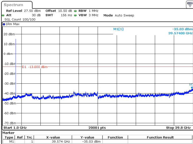
15MHz_15kHz_3707.5MHz_DFT-s-OFDM QPSK_RB1@0 -35.03 dBm
