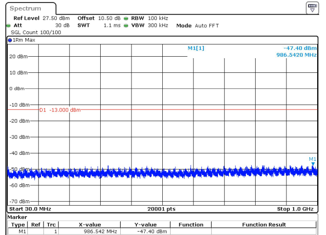
15MHz_15kHz_3972.5MHz_DFT-s-OFDM QPSK_RB75@0 -47.40 dBm
