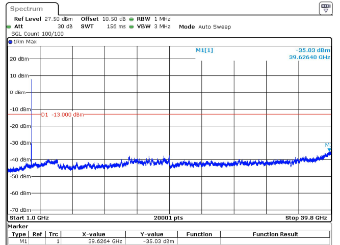
15MHz_15kHz_3840MHz_DFT-s-OFDM QPSK_RB75@0 -35.03 dBm
