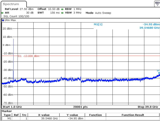
15MHz_15kHz_3840MHz_DFT-s-OFDM QPSK_RB1@0 -34.95 dBm
