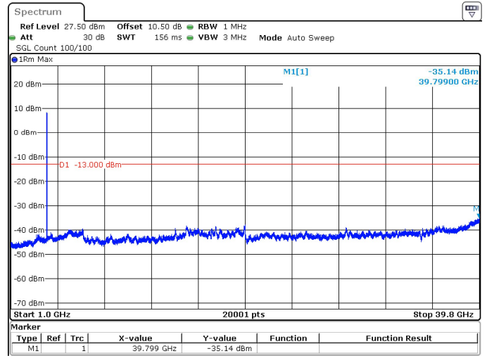
15MHz_15kHz_3972.5MHz_DFT-s-OFDM QPSK_RB1@0 -35.14 dBm
