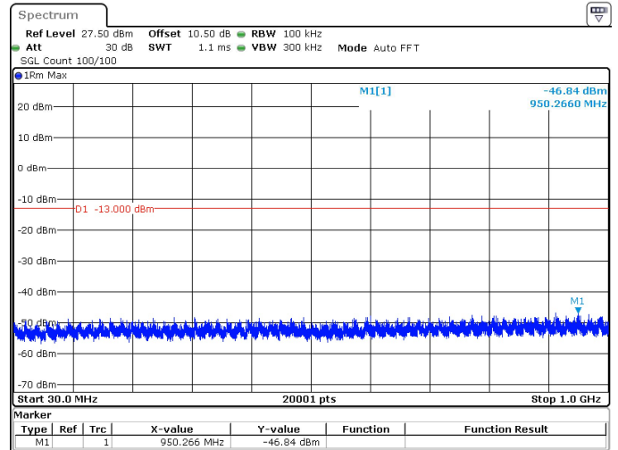
15MHz_15kHz_3972.5MHz_DFT-s-OFDM QPSK_RB1@78 -46.84 dBm
