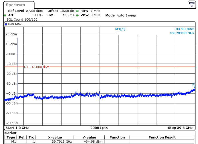
15MHz_15kHz_3707.5MHz_DFT-s-OFDM QPSK_RB1@78 -34.98 dBm
