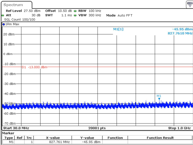
15MHz_15kHz_3840MHz_DFT-s-OFDM QPSK_RB75@0 -45.95 dBm
