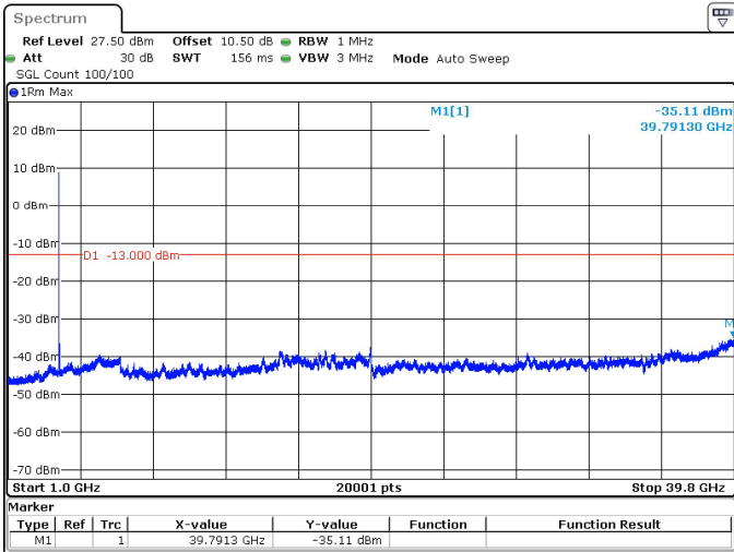
15MHz_15kHz_3707.5MHz_DFT-s-OFDM QPSK_RB75@0 -35.11 dBm
