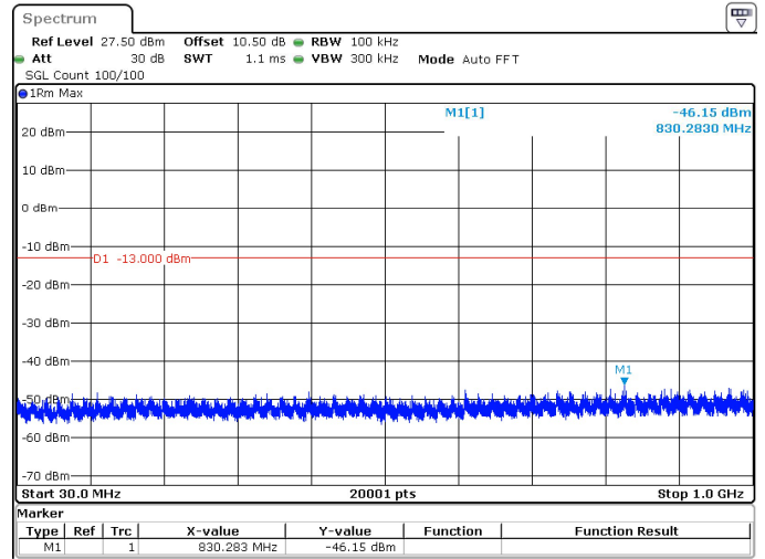
15MHz_15kHz_3707.5MHz_DFT-s-OFDM QPSK_RB1@0 -46.15 dBm
