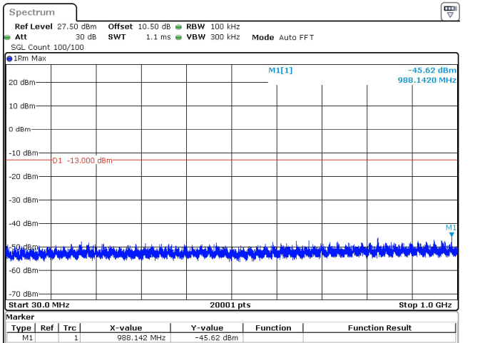
15MHz_15kHz_3707.5MHz_DFT-s-OFDM QPSK_RB1@78 -45.62 dBm
