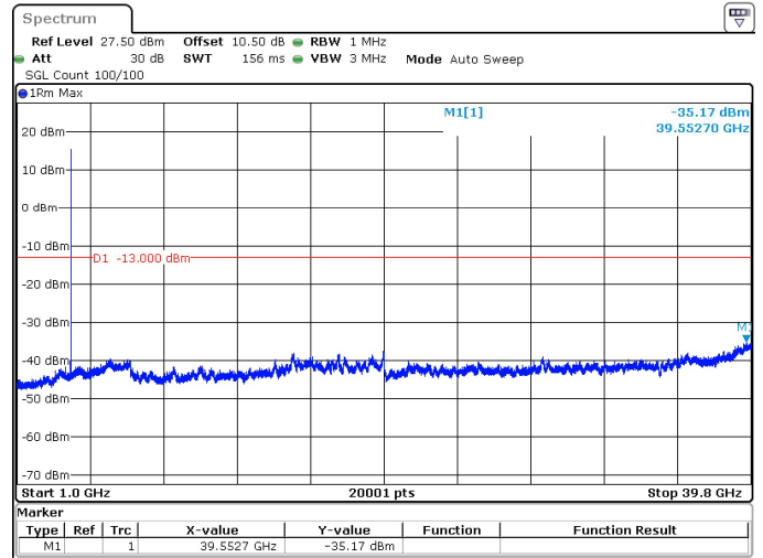
15MHz_15kHz_3840MHz_DFT-s-OFDM QPSK_RB1@78 -35.17 dBm
