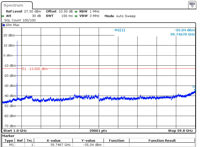
15MHz_15kHz_3972.5MHz_DFT-s-OFDM QPSK_RB1@78 -35.04 dBm
