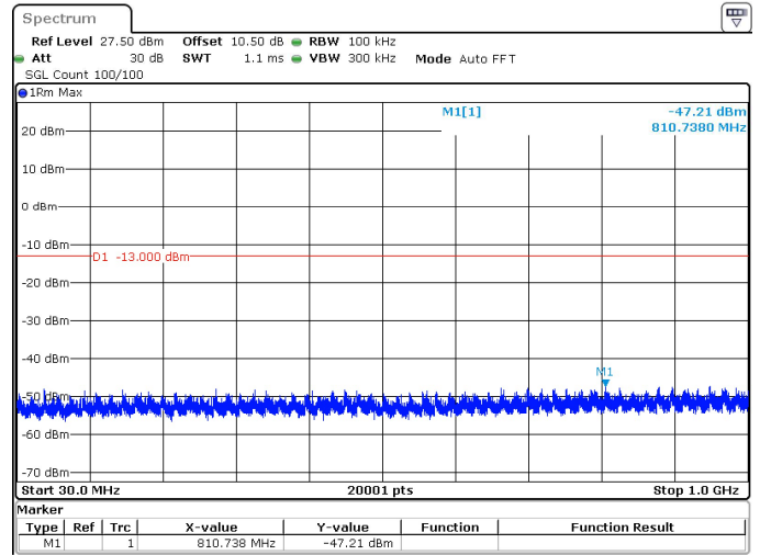
15MHz_15kHz_3840MHz_DFT-s-OFDM QPSK_RB1@0 -47.21 dBm
