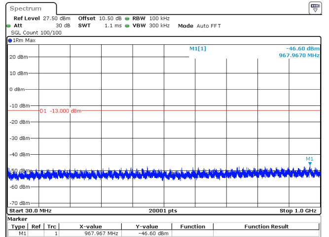
15MHz_15kHz_3707.5MHz_DFT-s-OFDM QPSK_RB75@0 -46.60 dBm
