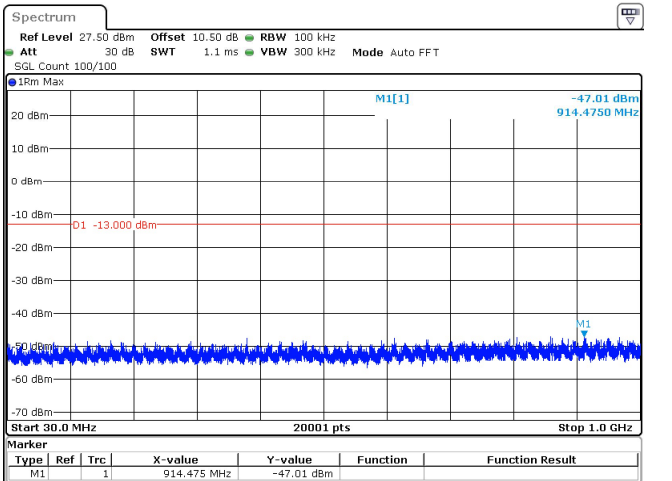
15MHz_15kHz_3840MHz_DFT-s-OFDM QPSK_RB1@78 -47.01 dBm
