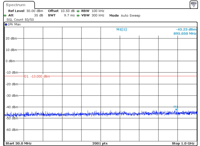
90MHz_30kHz_3505MHz_DFT-s-OFDM QPSK_RB1@244 -43.23 dBm
