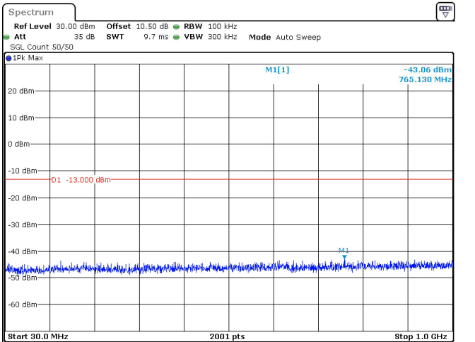
50MHz_30kHz_3500MHz_DFT-s-OFDM QPSK_RB1@132 -43.06 dBm
