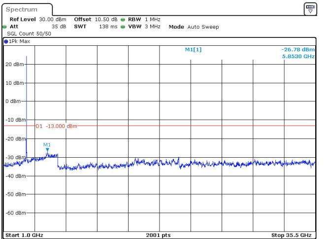
50MHz_30kHz_3525MHz_DFT-s-OFDM QPSK_RB1@132 -26.78 dBm
