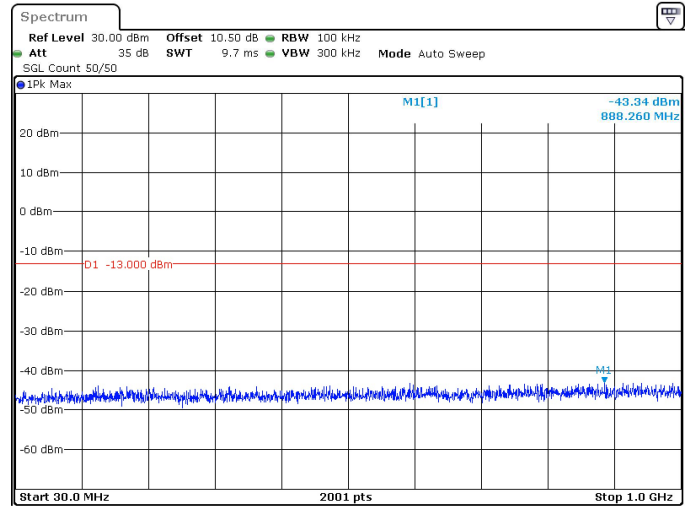
50MHz_15kHz_3500MHz_DFT-s-OFDM QPSK_RB1@269 -43.34 dBm
