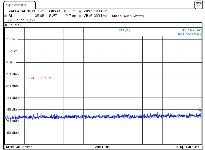
50MHz_15kHz_3525MHz_DFT-s-OFDM QPSK_RB1@0 -42.15 dBm
