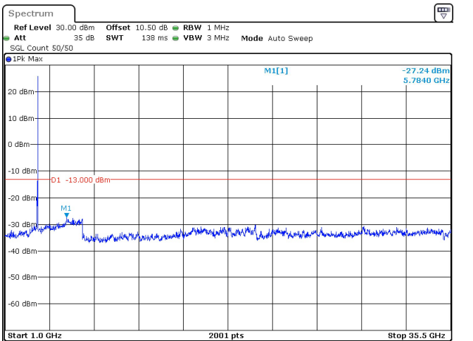
50MHz_15kHz_3500MHz_DFT-s-OFDM QPSK_RB1@269 -27.24 dBm
