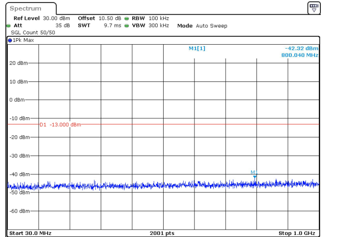
50MHz_15kHz_3525MHz_DFT-s-OFDM QPSK_RB270@0 -42.32 dBm
