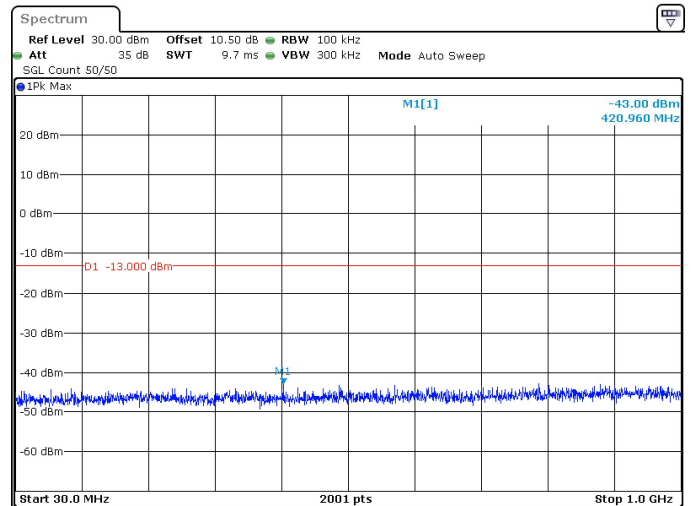
50MHz_30kHz_3475MHz_DFT-s-OFDM QPSK_RB1@132 -43.00 dBm
