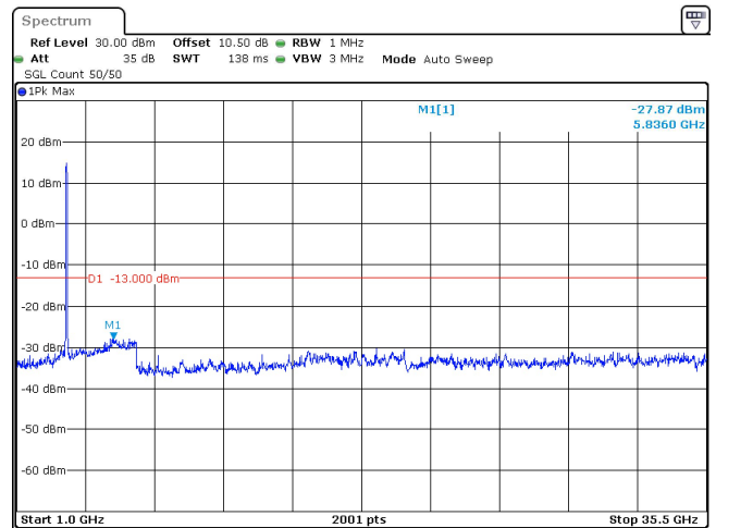
50MHz_15kHz_3500MHz_DFT-s-OFDM QPSK_RB270@0 -27.87 dBm
