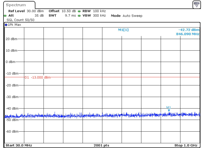
50MHz_15kHz_3525MHz_DFT-s-OFDM QPSK_RB1@269 -42.72 dBm
