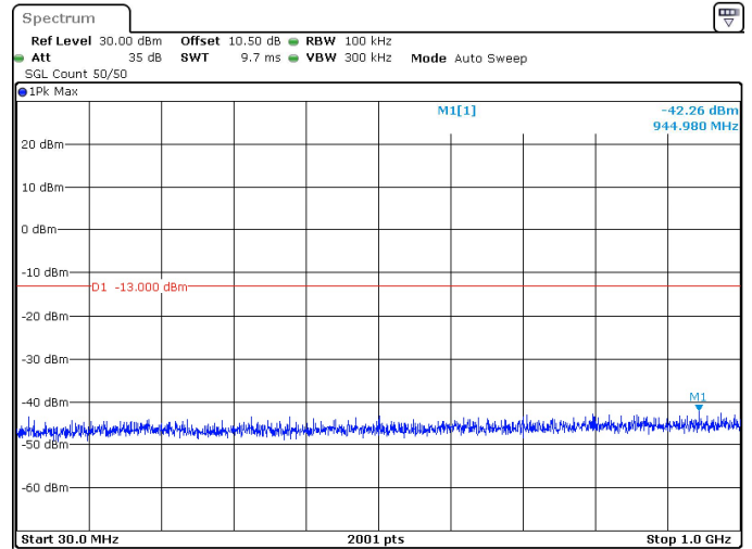
50MHz_30kHz_3475MHz_DFT-s-OFDM QPSK_RB1@0 -42.26 dBm
