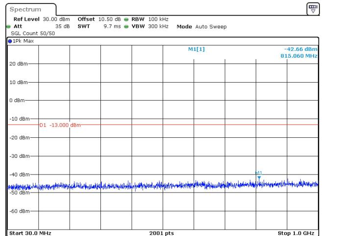
50MHz_30kHz_3475MHz_DFT-s-OFDM QPSK_RB128@0 -42.66 dBm
