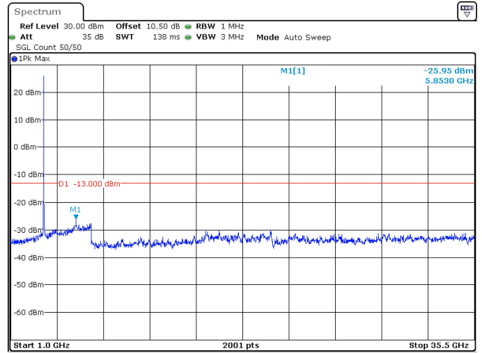
50MHz_15kHz_3475MHz_DFT-s-OFDM QPSK_RB1@0 -25.95 dBm
