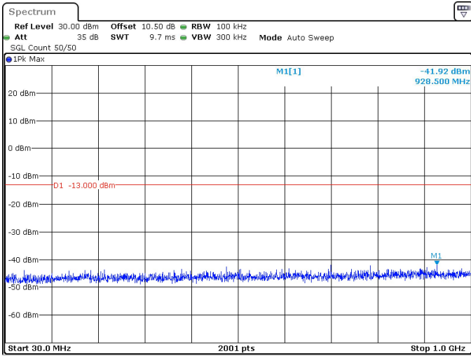
40MHz_30kHz_3500MHz_DFT-s-OFDM QPSK_RB100@0 -41.92 dBm
