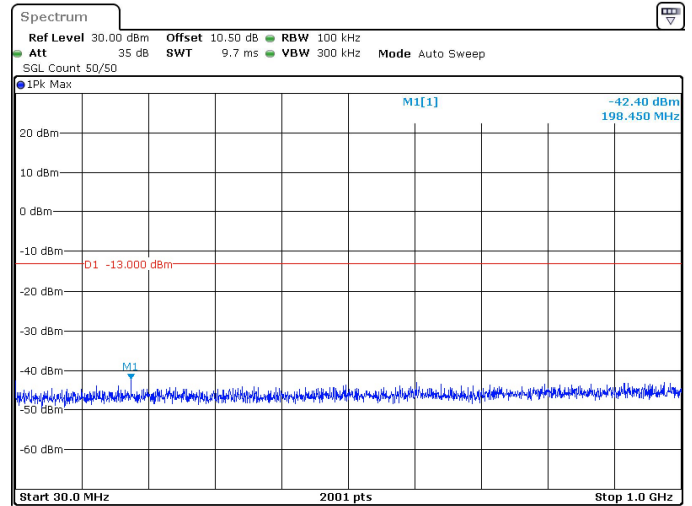
40MHz_30kHz_3530MHz_DFT-s-OFDM QPSK_RB1@105 -42.40 dBm
