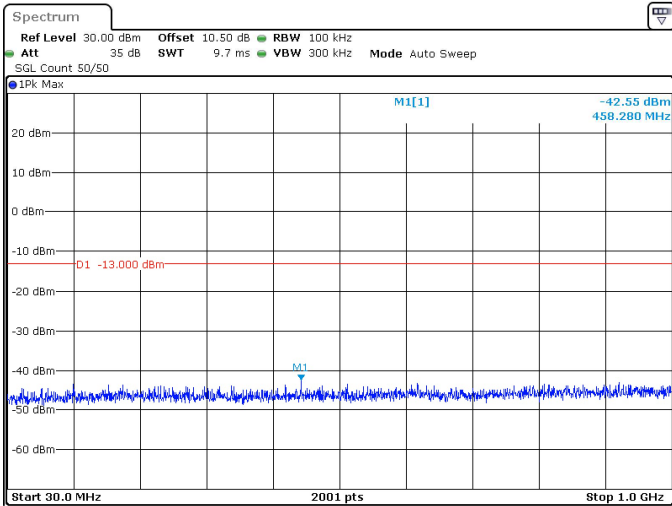
50MHz_15kHz_3475MHz_DFT-s-OFDM QPSK_RB1@0 -42.55 dBm
