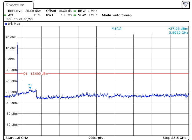
40MHz_30kHz_3500MHz_DFT-s-OFDM QPSK_RB100@0 -27.03 dBm
