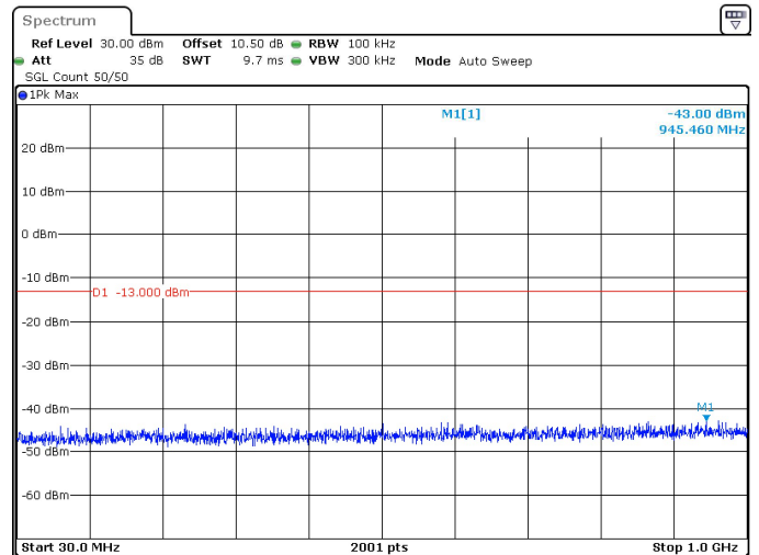
40MHz_30kHz_3500MHz_DFT-s-OFDM QPSK_RB1@105 -43.00 dBm
