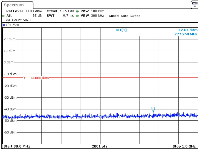
40MHz_30kHz_3470MHz_DFT-s-OFDM QPSK_RB100@0 -42.84 dBm
