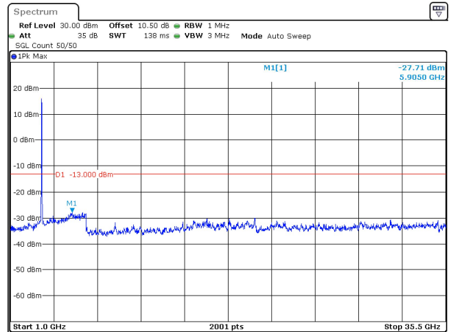
50MHz_15kHz_3475MHz_DFT-s-OFDM QPSK_RB270@0 -27.71 dBm
