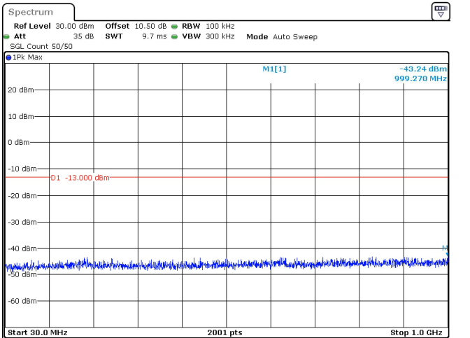
50MHz_15kHz_3475MHz_DFT-s-OFDM QPSK_RB1@269 -43.24 dBm
