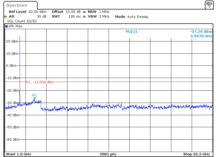
50MHz_15kHz_3475MHz_DFT-s-OFDM QPSK_RB1@269 -27.29 dBm
