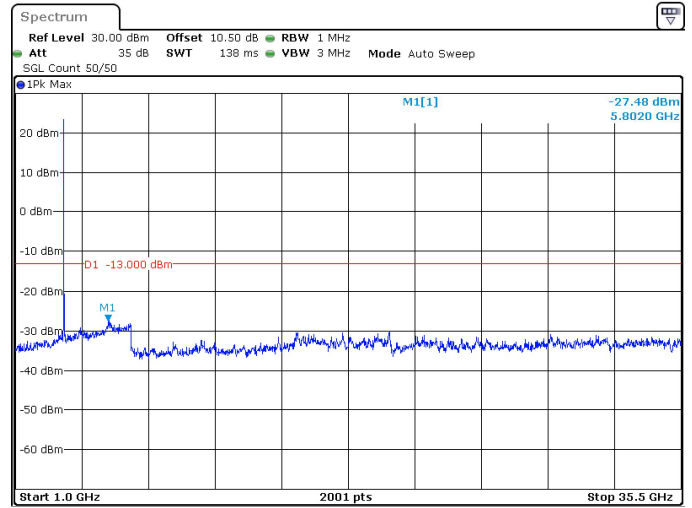
40MHz_15kHz_3530MHz_DFT-s-OFDM QPSK_RB1@0 -27.48 dBm
