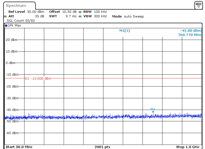
40MHz_15kHz_3500MHz_DFT-s-OFDM QPSK_RB1@215 -42.80 dBm
