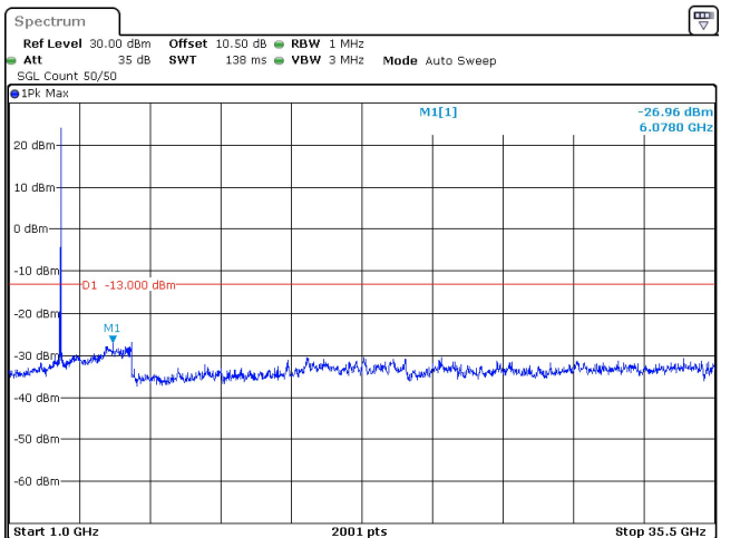
40MHz_15kHz_3500MHz_DFT-s-OFDM QPSK_RB1@215 -26.96 dBm
