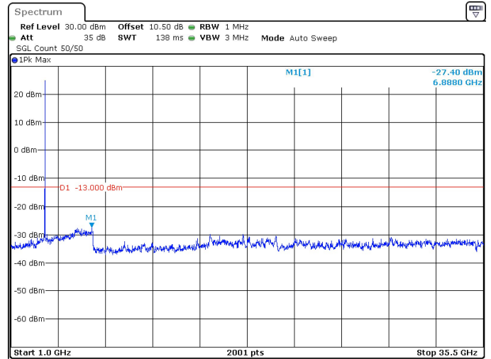
40MHz_30kHz_3470MHz_DFT-s-OFDM QPSK_RB1@105 -27.40 dBm
