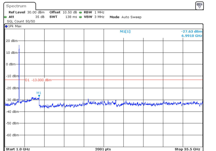
40MHz_15kHz_3500MHz_DFT-s-OFDM QPSK_RB216@0 -27.63 dBm
