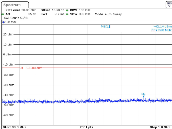
40MHz_15kHz_3500MHz_DFT-s-OFDM QPSK_RB1@0 -42.14 dBm
