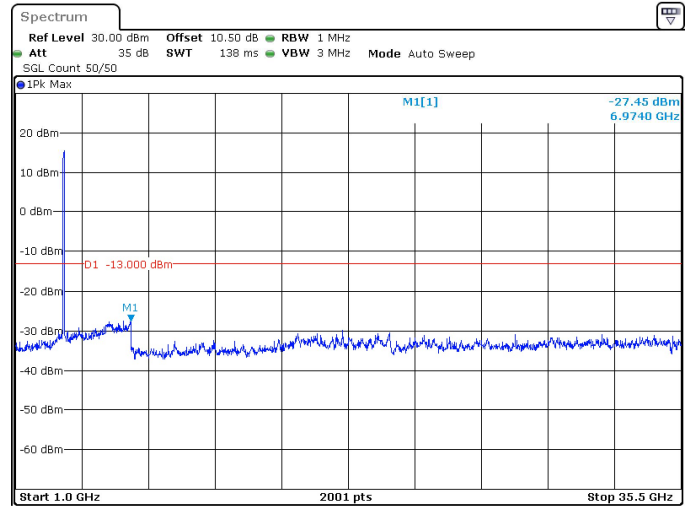
40MHz_15kHz_3500MHz_DFT-s-OFDM QPSK_RB1@0 -27.45 dBm
