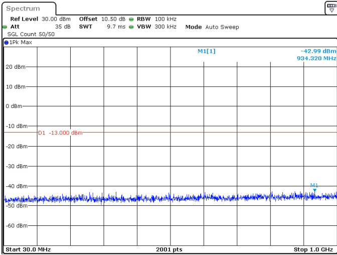
30MHz_15kHz_3535MHz_DFT-s-OFDM QPSK_RB160@0 -42.99 dBm
