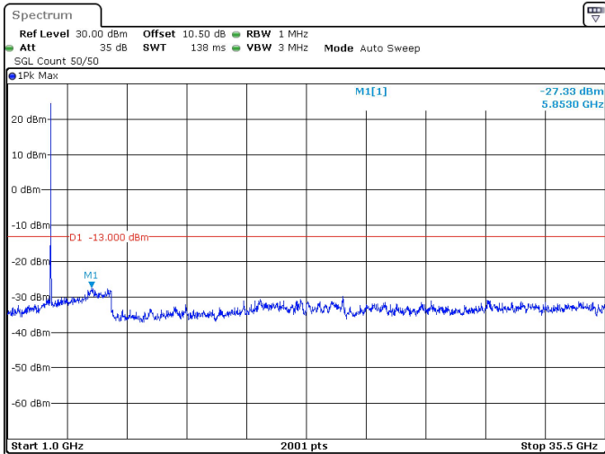
30MHz_15kHz_3500MHz_DFT-s-OFDM QPSK_RB1@0 -27.33 dBm
