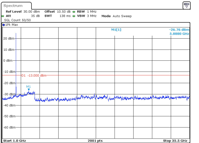
30MHz_15kHz_3535MHz_DFT-s-OFDM QPSK_RB1@159 -26.76 dBm
