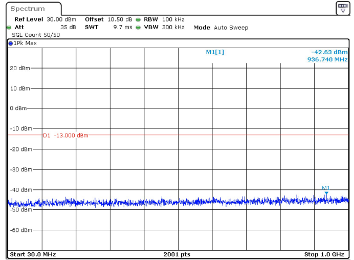
30MHz_15kHz_3500MHz_DFT-s-OFDM QPSK_RB1@0 -42.63 dBm
