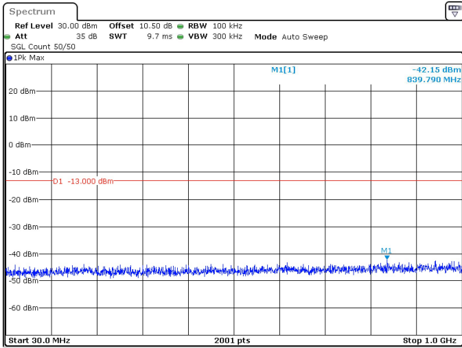
30MHz_15kHz_3465MHz_DFT-s-OFDM QPSK_RB160@0 -42.15 dBm
