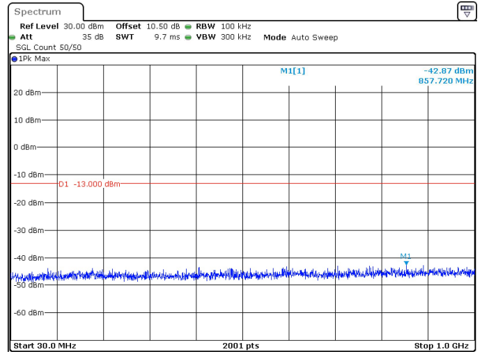
30MHz_15kHz_3535MHz_DFT-s-OFDM QPSK_RB1@159 -42.87 dBm
