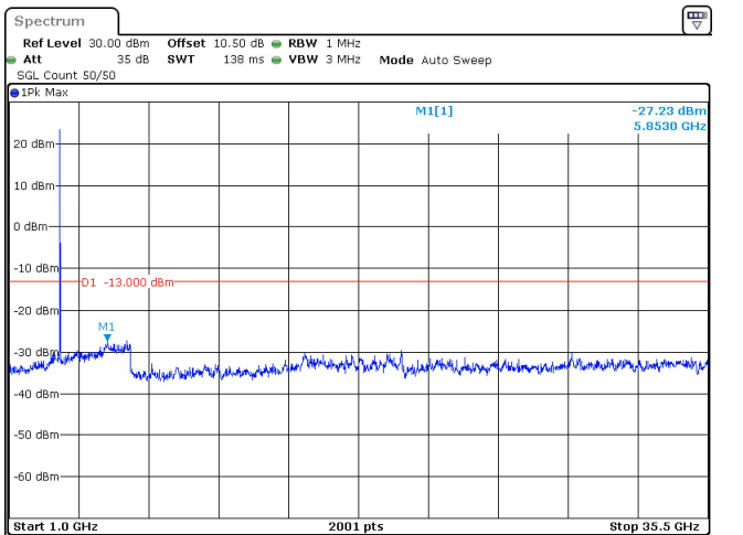
30MHz_15kHz_3500MHz_DFT-s-OFDM QPSK_RB1@159 -27.23 dBm
