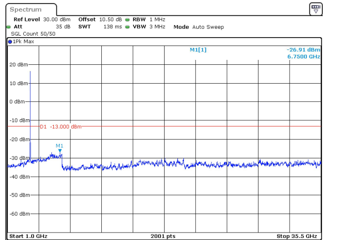
30MHz_15kHz_3500MHz_DFT-s-OFDM QPSK_RB160@0 -26.91 dBm
