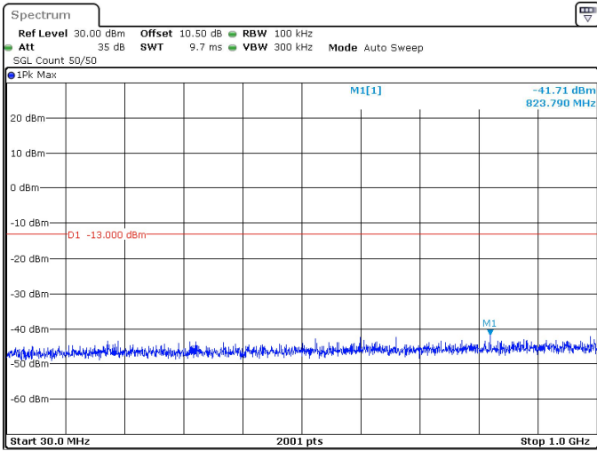
30MHz_15kHz_3500MHz_DFT-s-OFDM QPSK_RB160@0 -41.71 dBm
