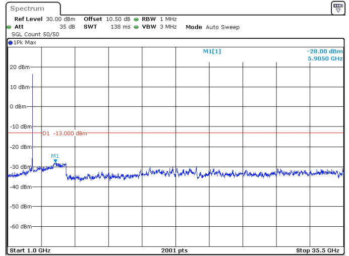
20MHz_15kHz_3540MHz_DFT-s-OFDM QPSK_RB1@0 -28.00 dBm
