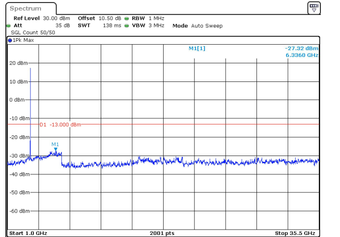
20MHz_15kHz_3540MHz_DFT-s-OFDM QPSK_RB100@0 -27.32 dBm
