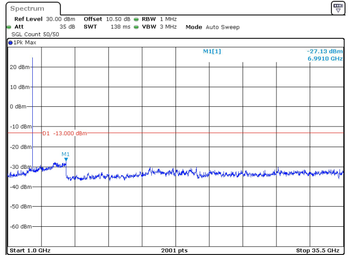
20MHz_15kHz_3540MHz_DFT-s-OFDM QPSK_RB1@105 -27.13 dBm
