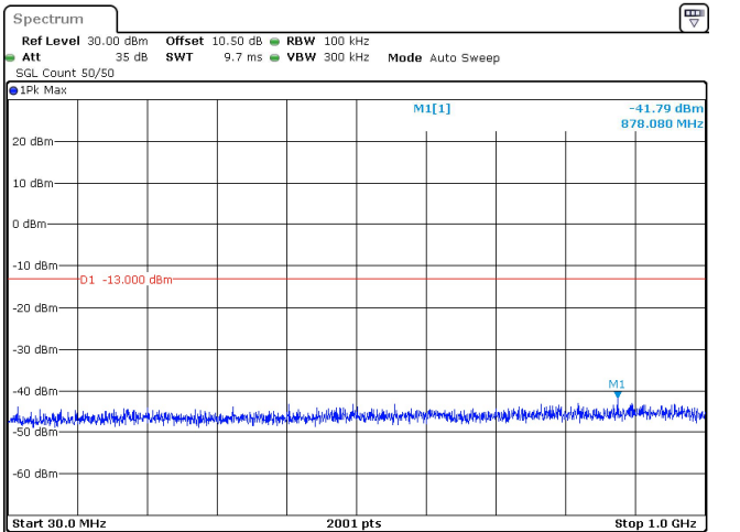
20MHz_15kHz_3540MHz_DFT-s-OFDM QPSK_RB1@105 -41.79 dBm
