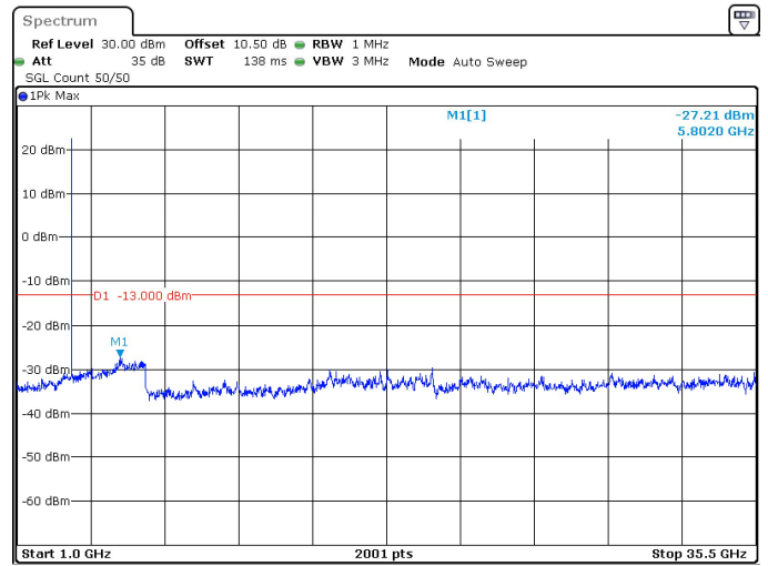
15MHz_30kHz_3542.5MHz_DFT-s-OFDM QPSK_RB1@0 -27.21 dBm
