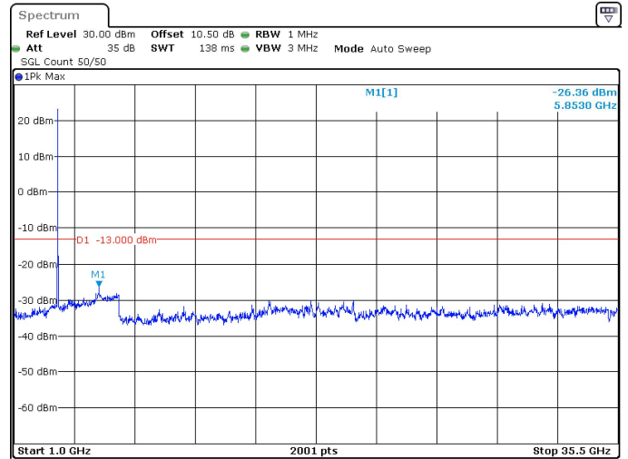
15MHz_30kHz_3500MHz_DFT-s-OFDM QPSK_RB1@37 -26.36 dBm
