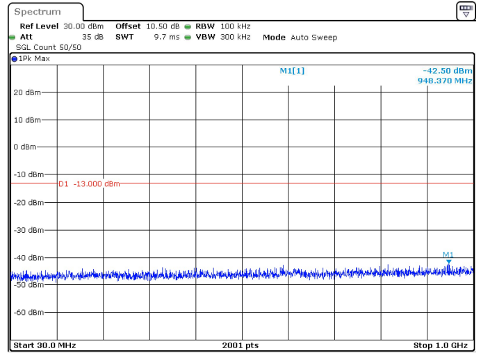
15MHz_30kHz_3500MHz_DFT-s-OFDM QPSK_RB1@0 -42.50 dBm
