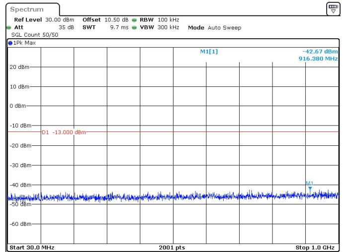
15MHz_30kHz_3542.5MHz_DFT-s-OFDM QPSK_RB1@37 -42.67 dBm
