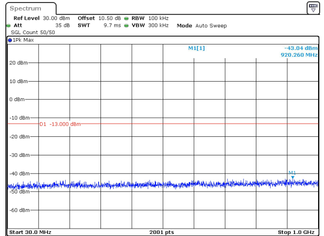
15MHz_30kHz_3500MHz_DFT-s-OFDM QPSK_RB36@0 -43.04 dBm
