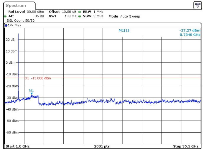
15MHz_15kHz_3457.5MHz_DFT-s-OFDM QPSK_RB1@0 -27.27 dBm
