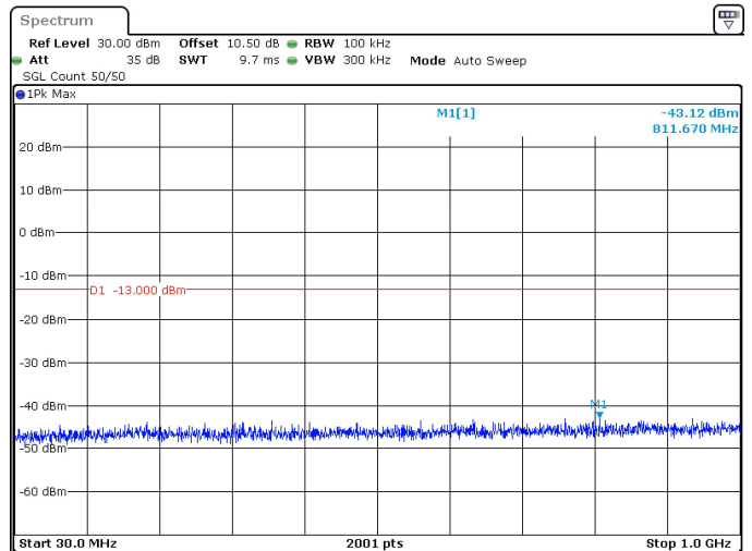
10MHz_30kHz_3545MHz_DFT-s-OFDM QPSK_RB1@23 -43.12 dBm
