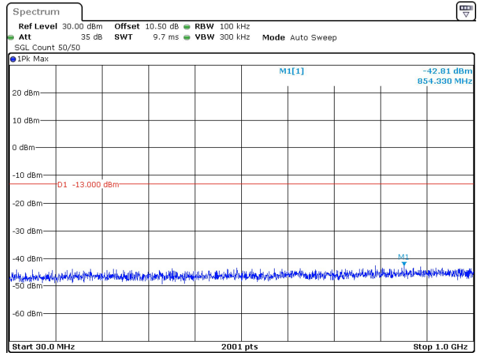
10MHz_30kHz_3545MHz_DFT-s-OFDM QPSK_RB1@0 -42.81 dBm
