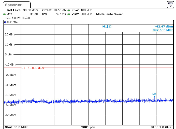
15MHz_15kHz_3457.5MHz_DFT-s-OFDM QPSK_RB1@78 -42.47 dBm
