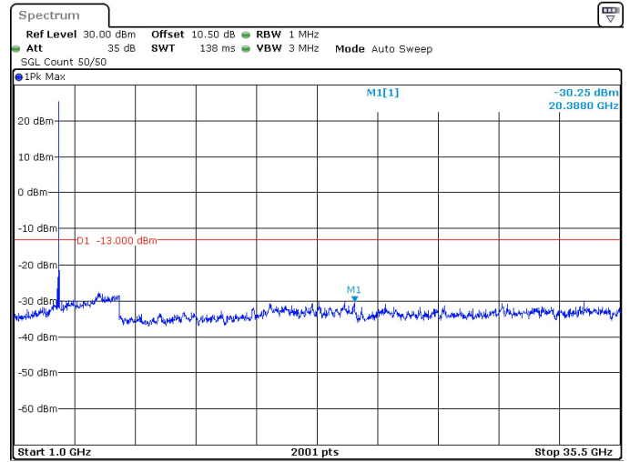
10MHz_15kHz_3545MHz_DFT-s-OFDM QPSK_RB1@0 -30.25 dBm
