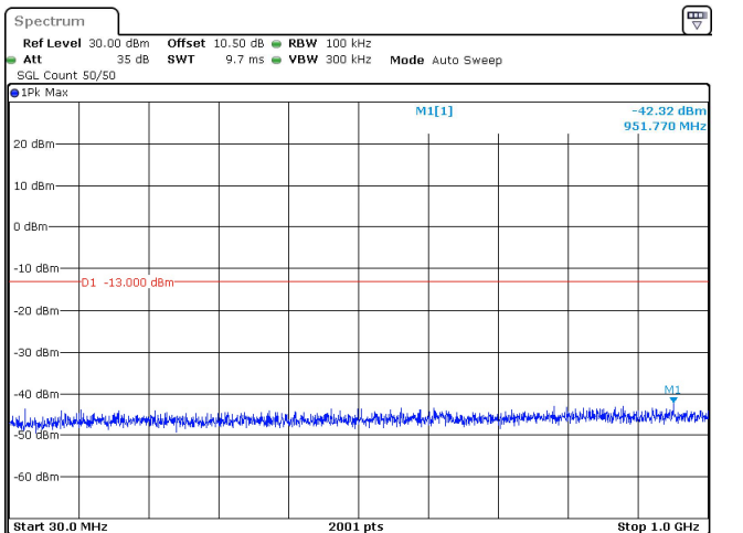
10MHz_15kHz_3500MHz_DFT-s-OFDM QPSK_RB1@51 -42.32 dBm
