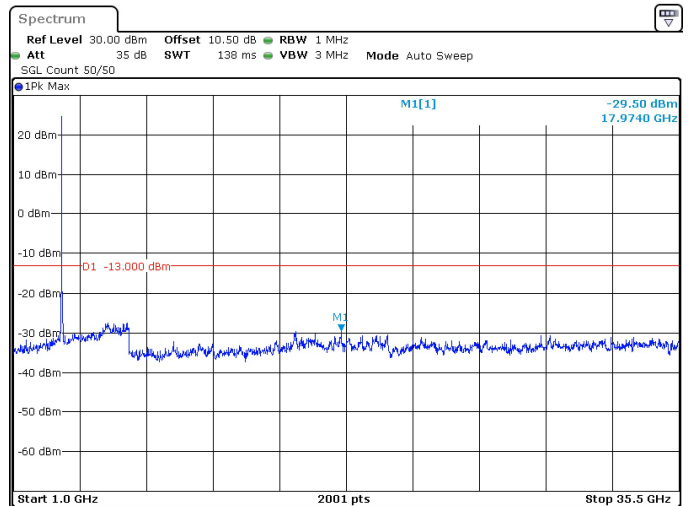
10MHz_15kHz_3500MHz_DFT-s-OFDM QPSK_RB1@51 -29.50 dBm
