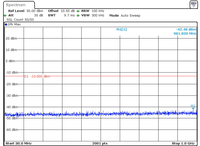
10MHz_15kHz_3545MHz_DFT-s-OFDM QPSK_RB1@51 -42.48 dBm
