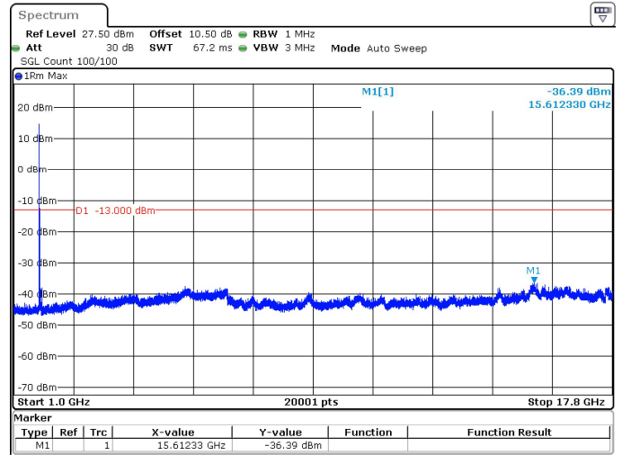
40MHz_15kHz_1730MHz_DFT-s-OFDM QPSK_RB1@0 -36.39 dBm
