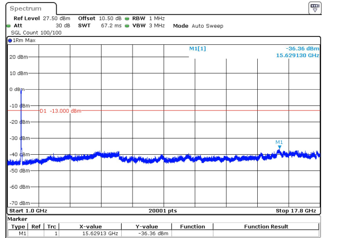
40MHz_15kHz_1730MHz_DFT-s-OFDM QPSK_RB216@0 -36.36 dBm
