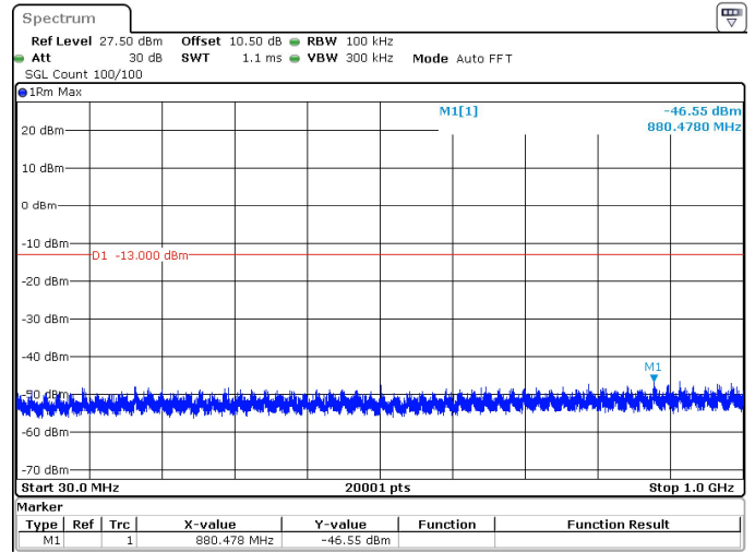
40MHz_15kHz_1730MHz_DFT-s-OFDM QPSK_RB1@215 -46.55 dBm
