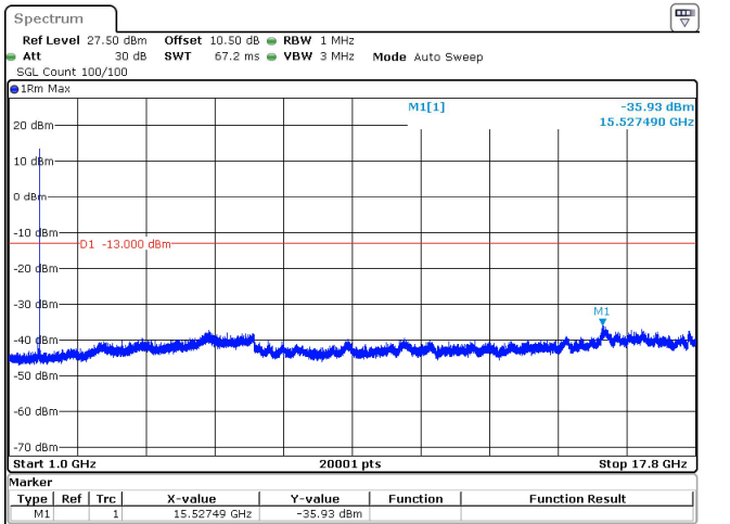
40MHz_15kHz_1730MHz_DFT-s-OFDM QPSK_RB1@215 -35.93 dBm
