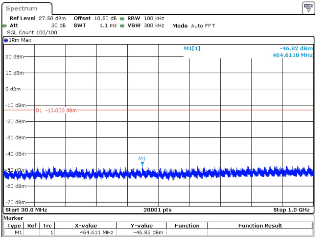
10MHz_15kHz_1745MHz_DFT-s-OFDM QPSK_RB1@51 -46.82 dBm
