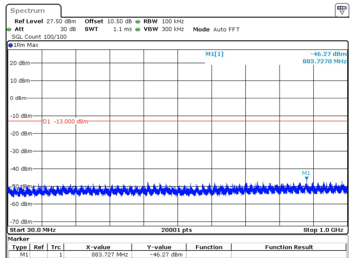
15MHz_15kHz_1717.5MHz_DFT-s-OFDM QPSK_RB1@78 -46.27 dBm
