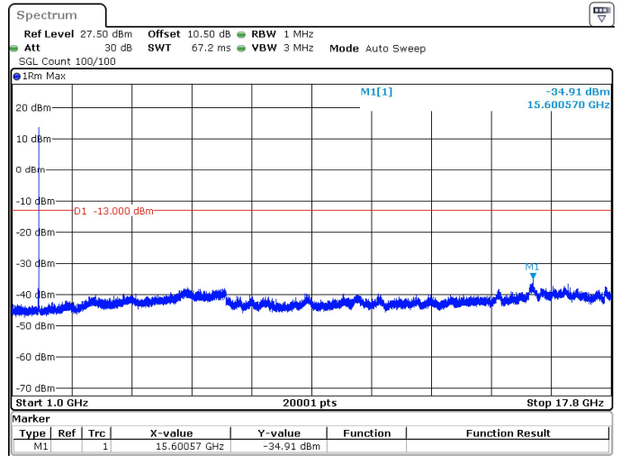
10MHz_15kHz_1745MHz_DFT-s-OFDM QPSK_RB1@51 -34.91 dBm
