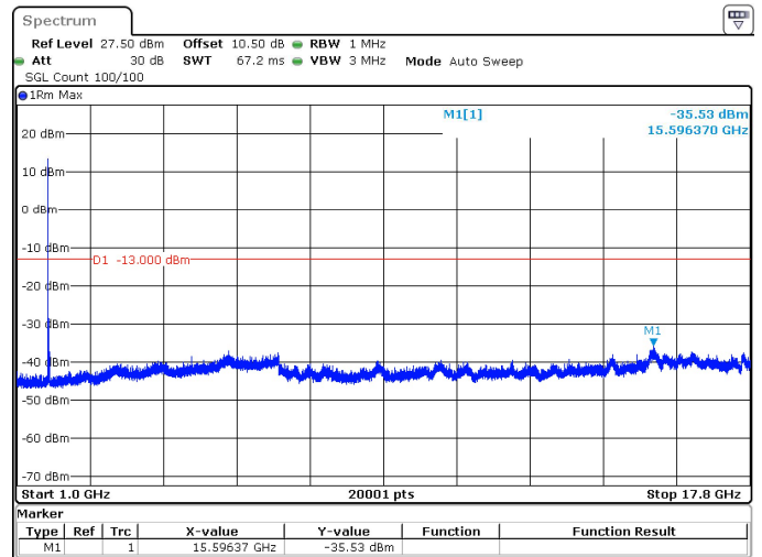
15MHz_15kHz_1717.5MHz_DFT-s-OFDM QPSK_RB1@0 -35.53 dBm
