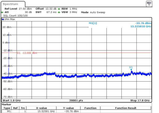
10MHz_15kHz_1775MHz_DFT-s-OFDM QPSK_RB1@51 -35.76 dBm
