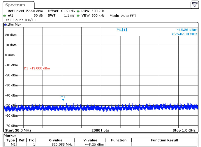
10MHz_15kHz_1775MHz_DFT-s-OFDM QPSK_RB1@51 -45.26 dBm
