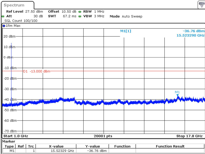
10MHz_15kHz_1745MHz_DFT-s-OFDM QPSK_RB1@0 -36.76 dBm
