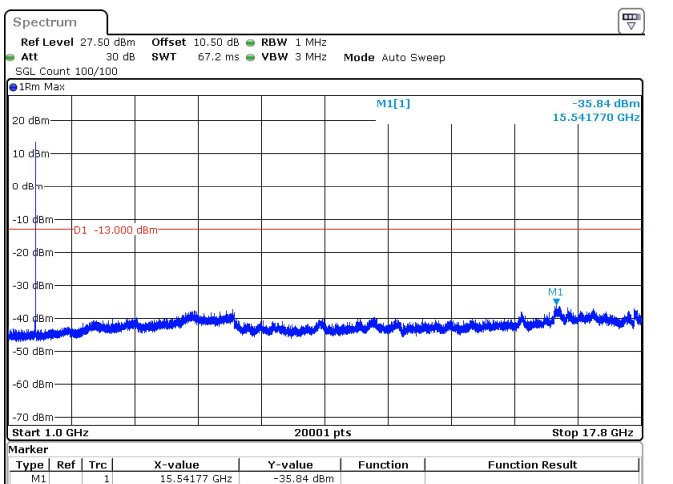
15MHz_15kHz_1717.5MHz_DFT-s-OFDM QPSK_RB1@78 -35.84 dBm
