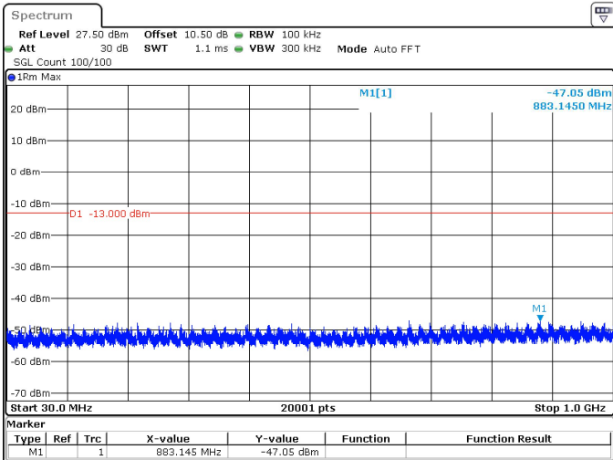
5MHz_15kHz_1745MHz_DFT-s-OFDM QPSK_RB1@0 -47.05 dBm
