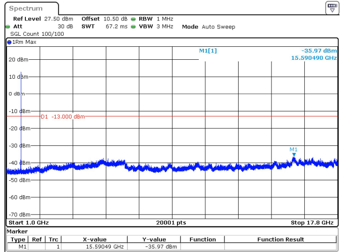
10MHz_15kHz_1715MHz_DFT-s-OFDM QPSK_RB1@51 -35.97 dBm
