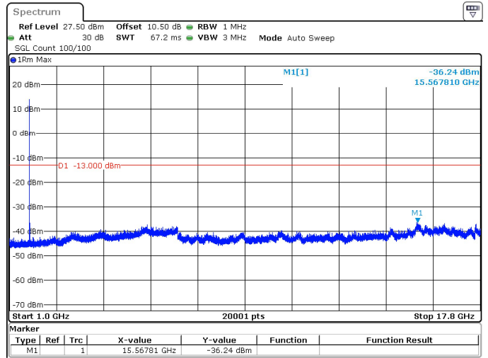
10MHz_15kHz_1715MHz_DFT-s-OFDM QPSK_RB1@0 -36.24 dBm
