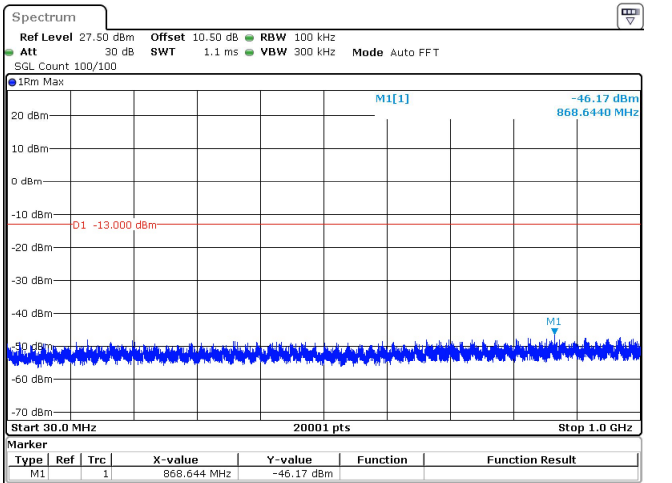
10MHz_15kHz_1715MHz_DFT-s-OFDM QPSK_RB1@51 -46.17 dBm
