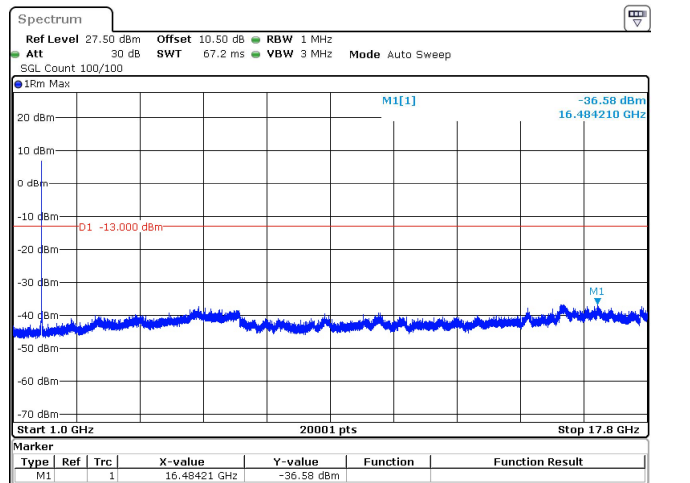
5MHz_15kHz_1745MHz_DFT-s-OFDM QPSK_RB25@0 -36.58 dBm
