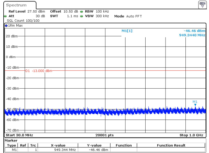
5MHz_15kHz_1777.5MHz_DFT-s-OFDM QPSK_RB1@24 -46.46 dBm
