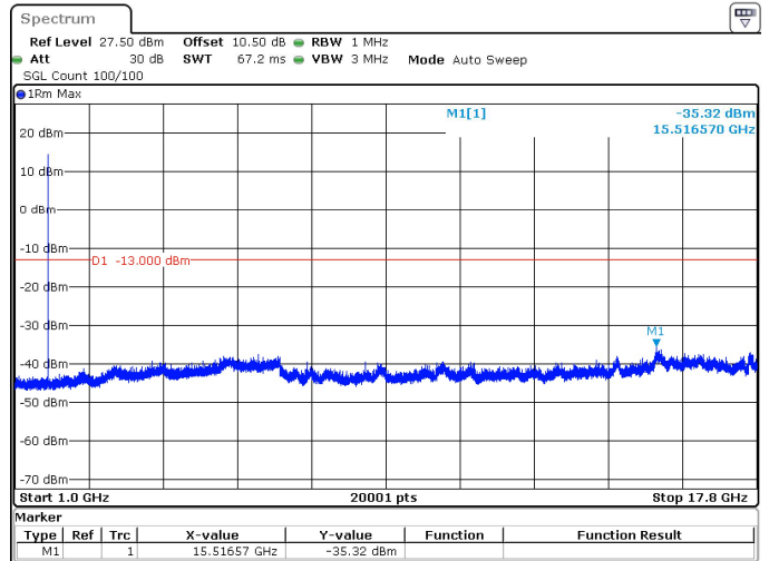
5MHz_15kHz_1745MHz_DFT-s-OFDM QPSK_RB1@24 -35.32 dBm
