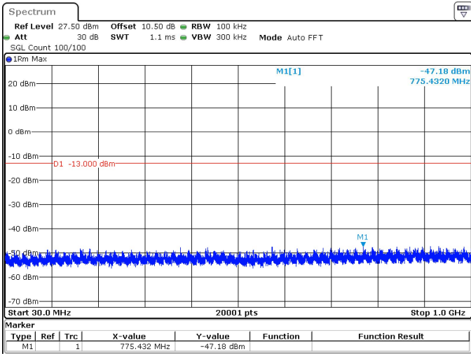
10MHz_15kHz_1715MHz_DFT-s-OFDM QPSK_RB1@0 -47.18 dBm
