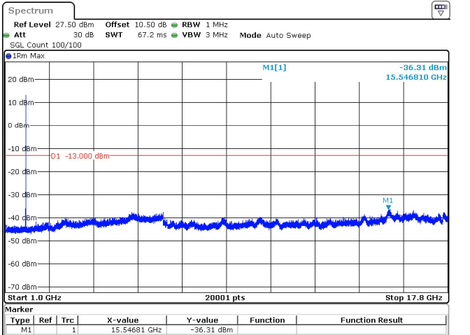
5MHz_15kHz_1777.5MHz_DFT-s-OFDM QPSK_RB1@24 -36.31 dBm
