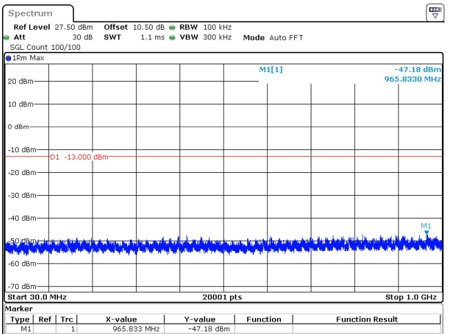
5MHz_15kHz_1745MHz_DFT-s-OFDM QPSK_RB1@24 -47.18 dBm
