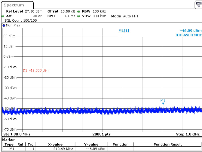
5MHz_15kHz_1777.5MHz_DFT-s-OFDM QPSK_RB1@0 -46.09 dBm
