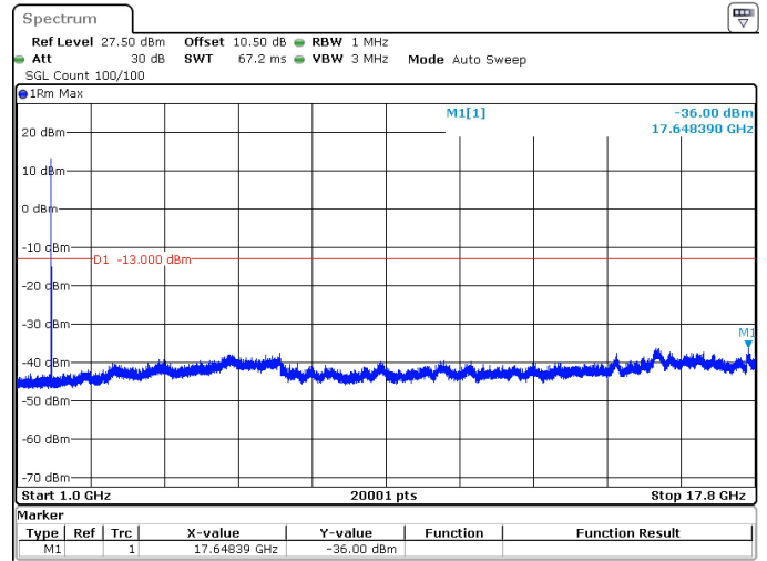
5MHz_15kHz_1777.5MHz_DFT-s-OFDM QPSK_RB1@0 -36.00 dBm
