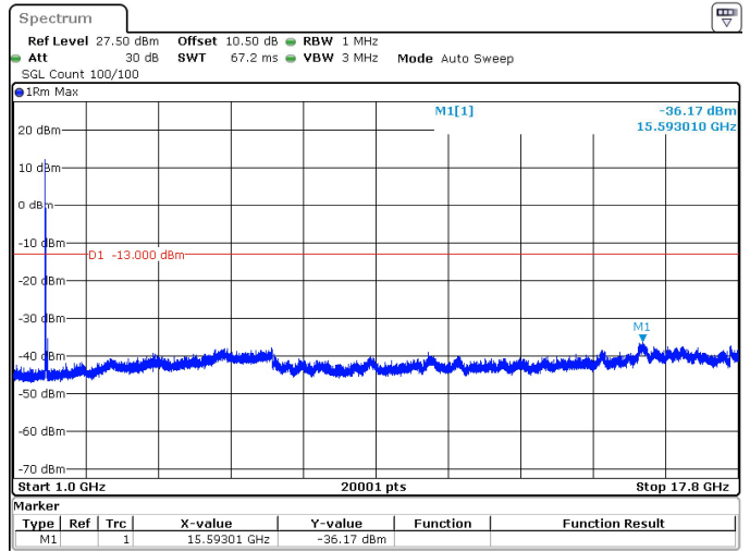
25MHz_15kHz_1745MHz_DFT-s-OFDM QPSK_RB1@0 -36.17 dBm
