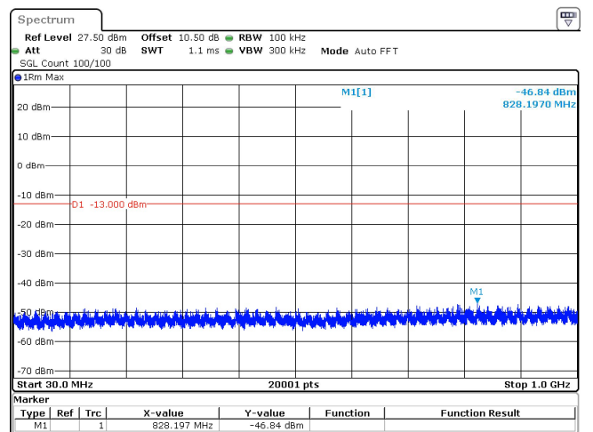
25MHz_15kHz_1767.5MHz_DFT-s-OFDM QPSK_RB128@0 -46.84 dBm
