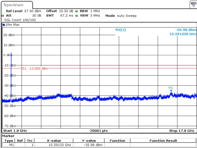
25MHz_15kHz_1767.5MHz_DFT-s-OFDM QPSK_RB128@0 -35.98 dBm
