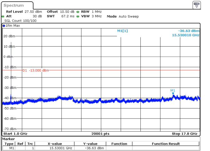
30MHz_15kHz_1725MHz_DFT-s-OFDM QPSK_RB1@159 -36.63 dBm
