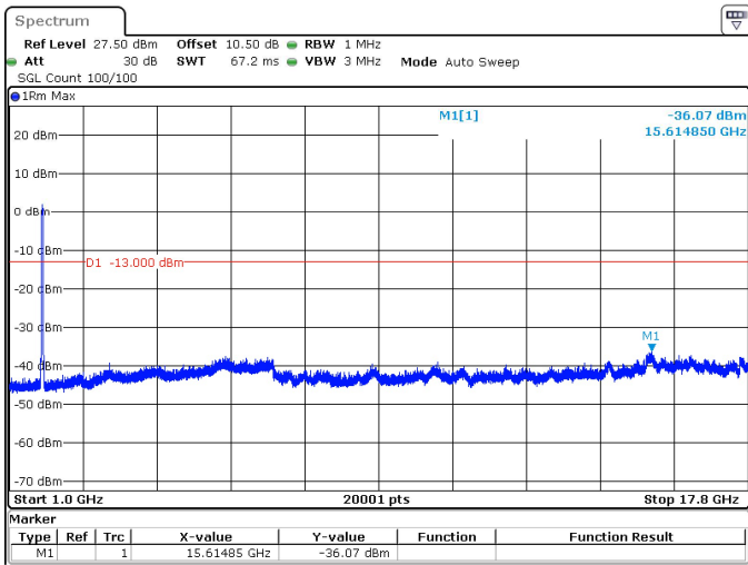
25MHz_15kHz_1745MHz_DFT-s-OFDM QPSK_RB128@0 -36.07 dBm
