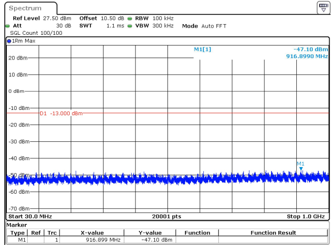
30MHz_15kHz_1725MHz_DFT-s-OFDM QPSK_RB1@159 -47.10 dBm
