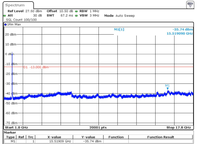
30MHz_15kHz_1725MHz_DFT-s-OFDM QPSK_RB160@0 -35.74 dBm
