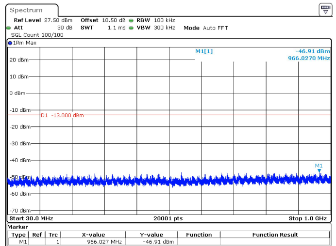
25MHz_15kHz_1767.5MHz_DFT-s-OFDM QPSK_RB1@132 -46.91 dBm
