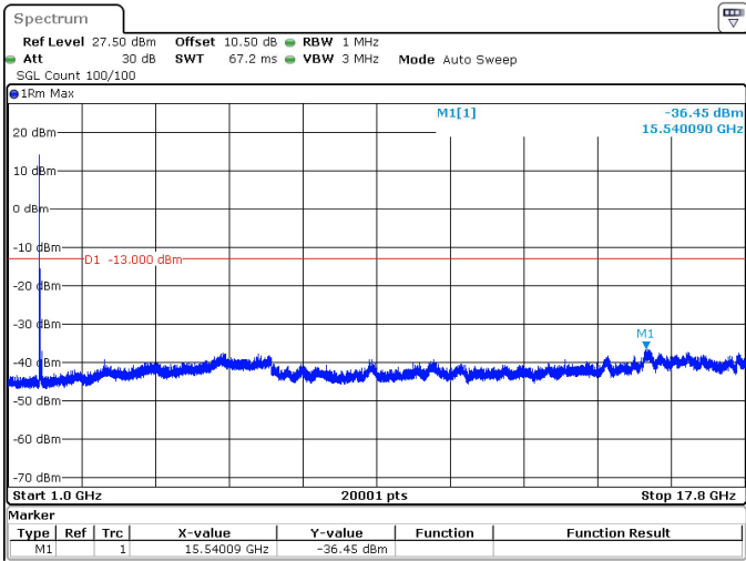
30MHz_15kHz_1725MHz_DFT-s-OFDM QPSK_RB1@0 -36.45 dBm
