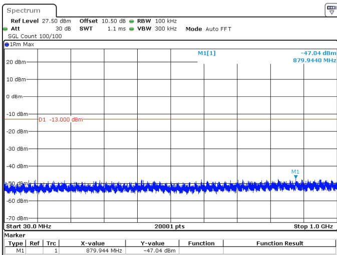
25MHz_15kHz_1767.5MHz_DFT-s-OFDM QPSK_RB1@0 -47.04 dBm
