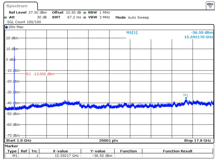
25MHz_15kHz_1767.5MHz_DFT-s-OFDM QPSK_RB1@0 -36.50 dBm
