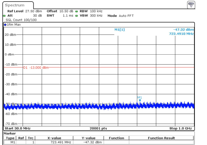
25MHz_15kHz_1745MHz_DFT-s-OFDM QPSK_RB128@0 -47.32 dBm
