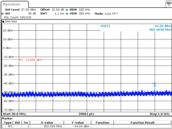
25MHz_15kHz_1722.5MHz_DFT-s-OFDM QPSK_RB128@0 -44.04 dBm
