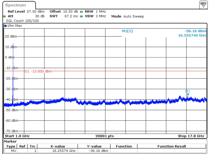
25MHz_15kHz_1745MHz_DFT-s-OFDM QPSK_RB1@132 -36.16 dBm
