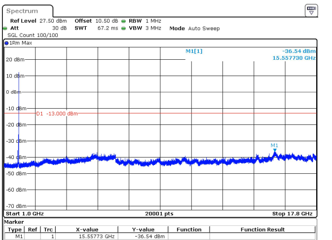
25MHz_15kHz_1767.5MHz_DFT-s-OFDM QPSK_RB1@132 -36.54 dBm
