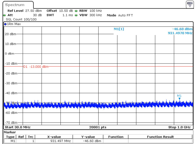
30MHz_15kHz_1725MHz_DFT-s-OFDM QPSK_RB1@0 -46.60 dBm
