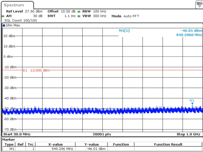
25MHz_15kHz_1745MHz_DFT-s-OFDM QPSK_RB1@0 -46.01 dBm
