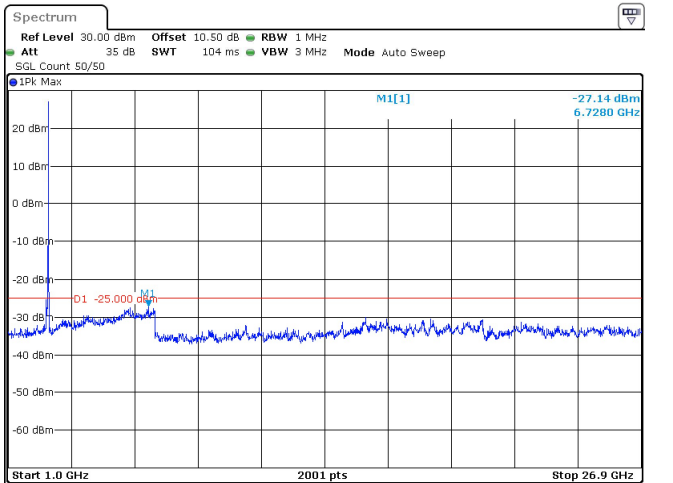
100MHz_30kHz_2592.99MHz_DFT-s-OFDM QPSK_RB1@272 -27.14 dBm
