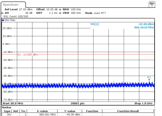
5MHz_15kHz_1712.5MHz_DFT-s-OFDM QPSK_RB1@24 -45.90 dBm
