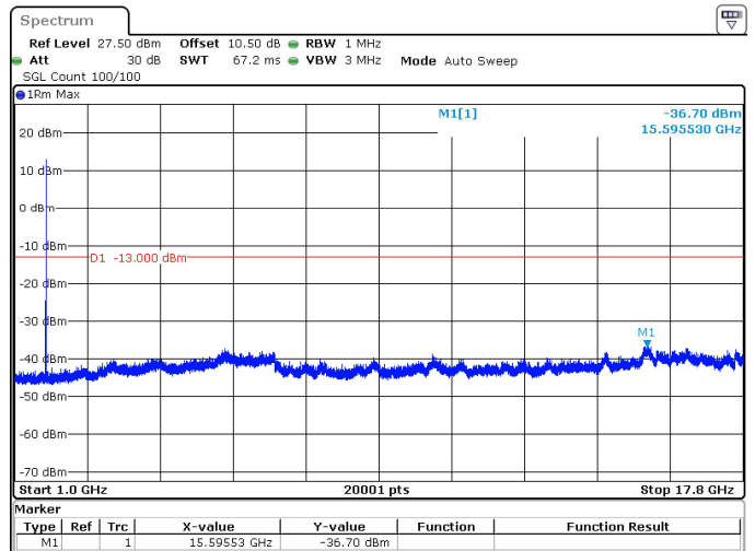
5MHz_15kHz_1712.5MHz_DFT-s-OFDM QPSK_RB1@24 -36.70 dBm
