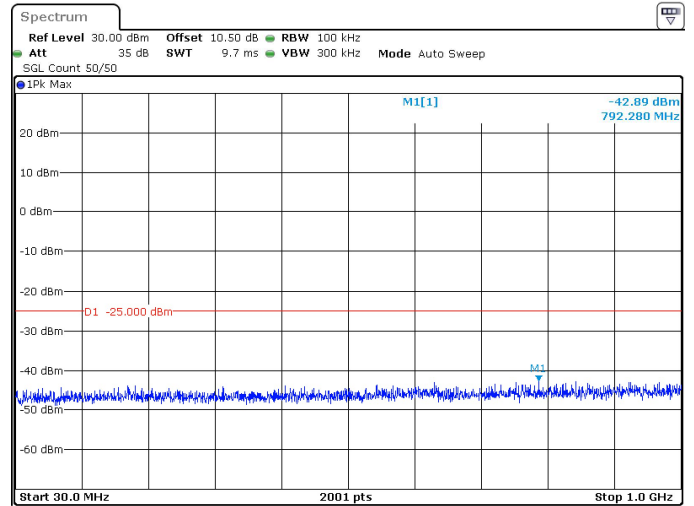
100MHz_30kHz_2592.99MHz_DFT-s-OFDM QPSK_RB1@272 -42.89 dBm
