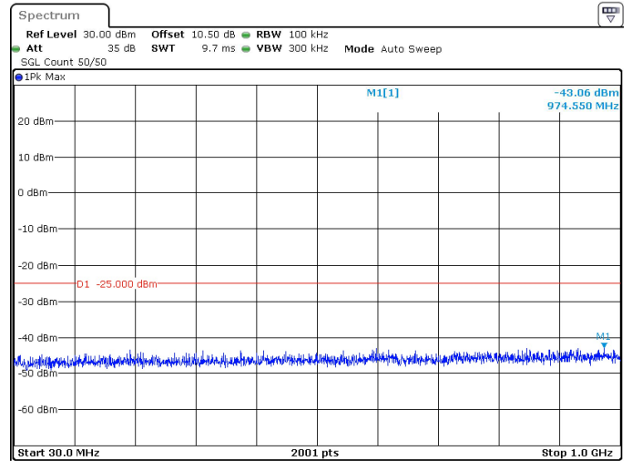
100MHz_30kHz_2592.99MHz_DFT-s-OFDM QPSK_RB1@0 -43.06 dBm
